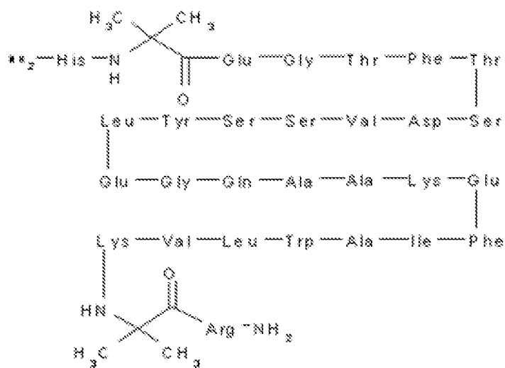
BIM-51077
