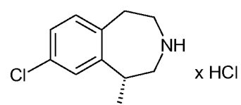
lorcaserin hydrochloride
