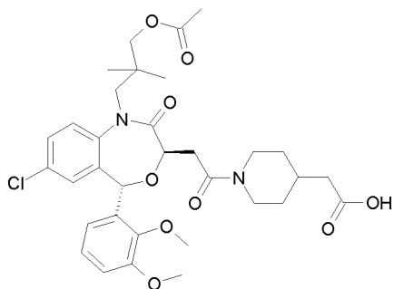
TAK-475
