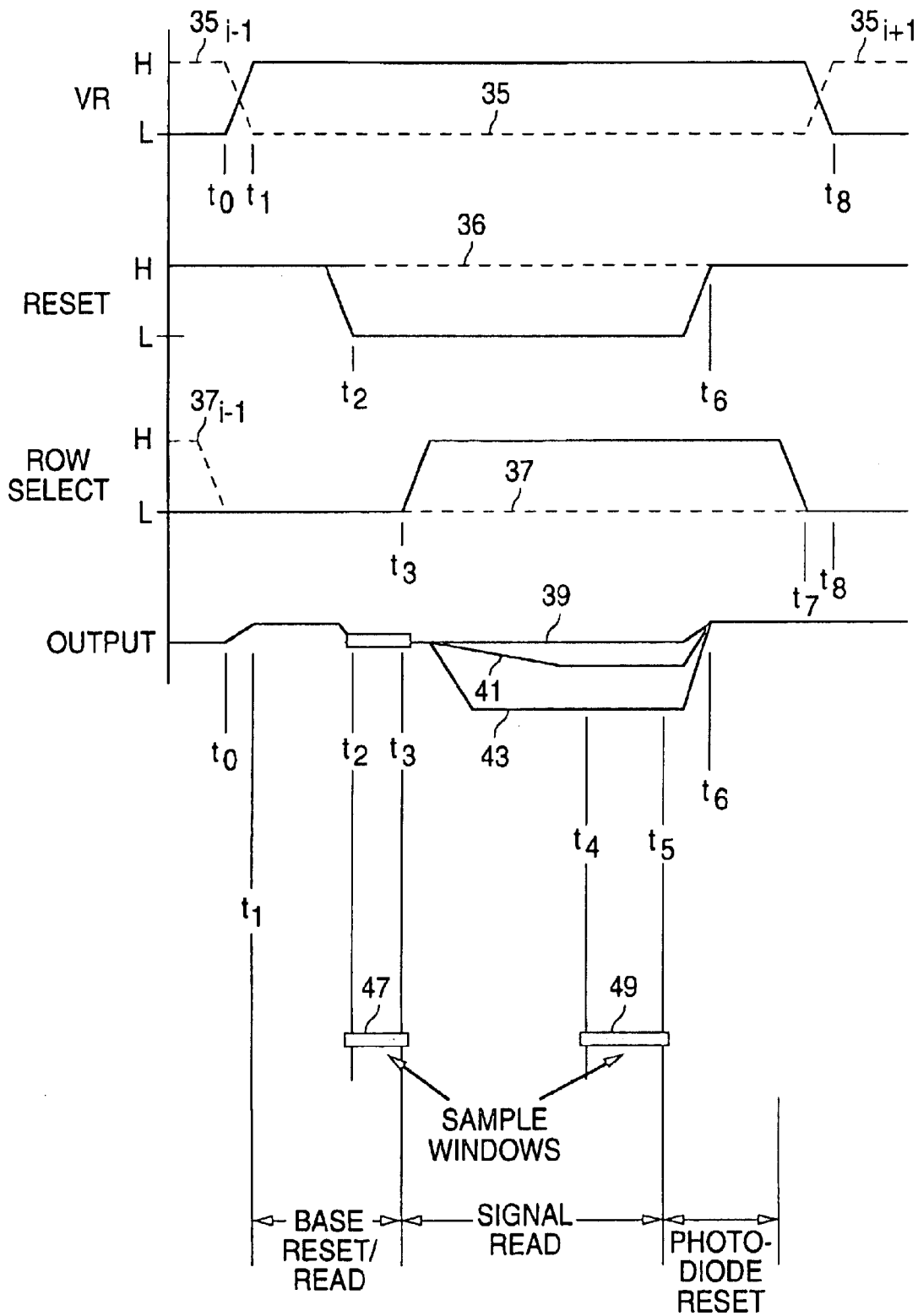
FIG. 2 (PRIOR ART)
