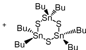
Di-n-butyltinsulfide
