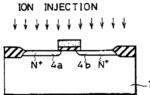
FIG. 1C PRIOR ART
