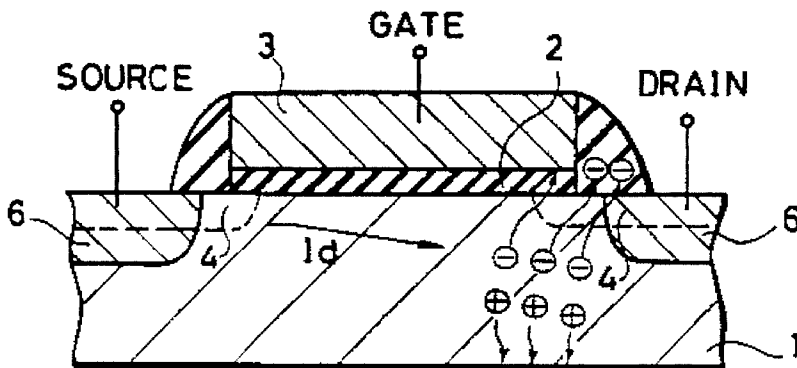
FIG. 7C PRIOR ART
