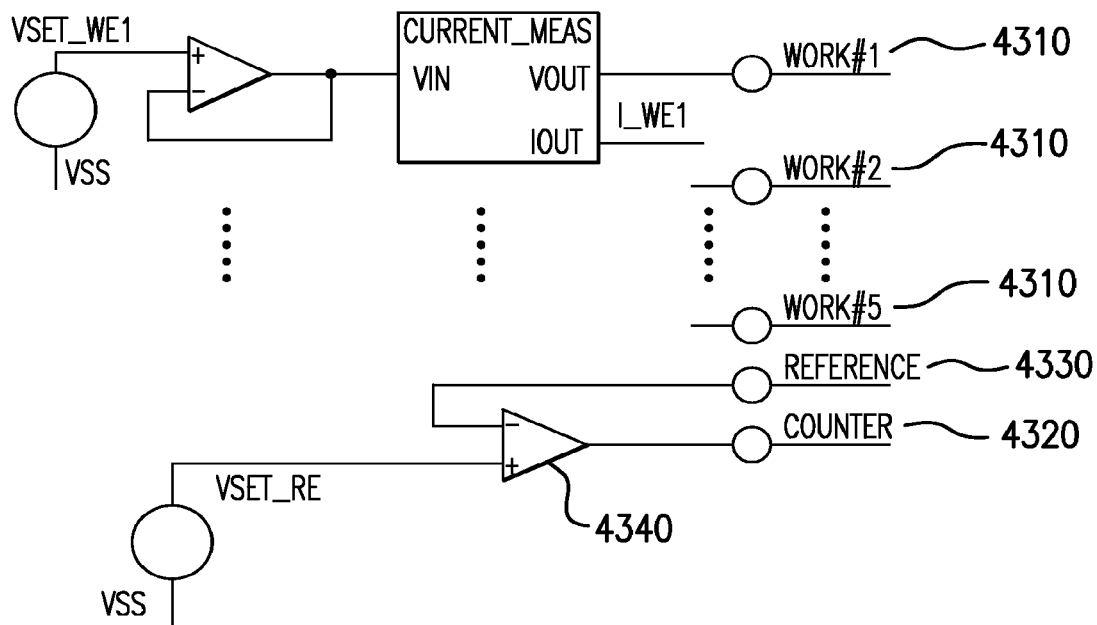
POTENTIOSTAT CONFIGURATION
