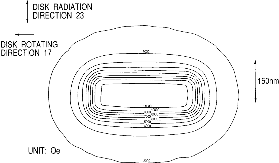
CONTOURS OF PERPENDICULAR COMPONENT OF WRITE FIELD GENERATED FROM A SINGLE POLE TYPE HEAD
