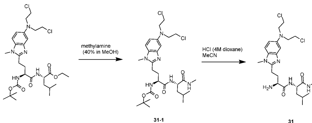
Scheme 9
