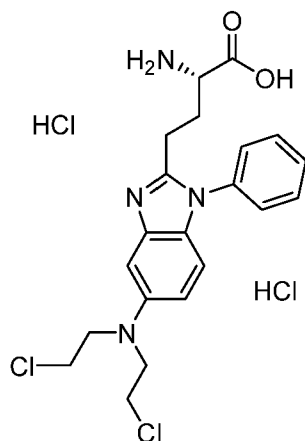
Scheme 11
