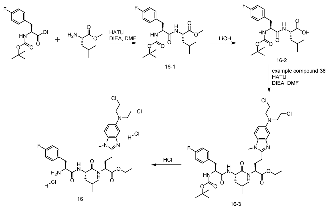
Scheme 5
