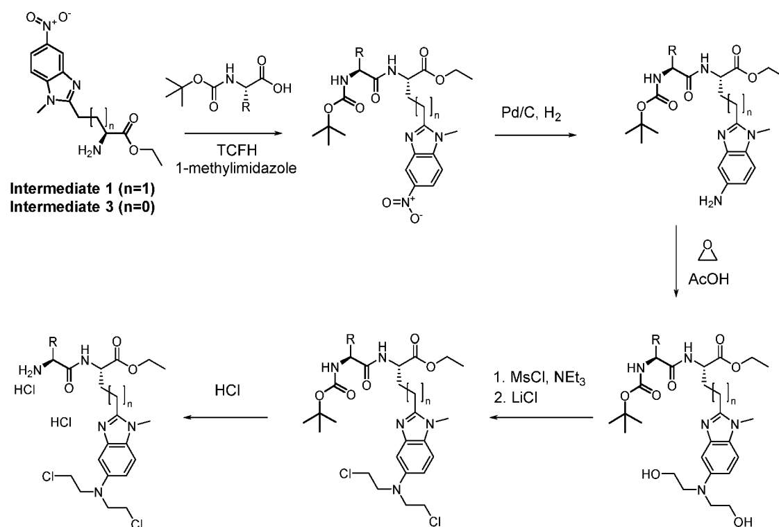
Scheme 3
