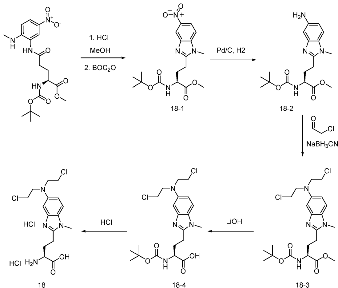
Scheme 7
