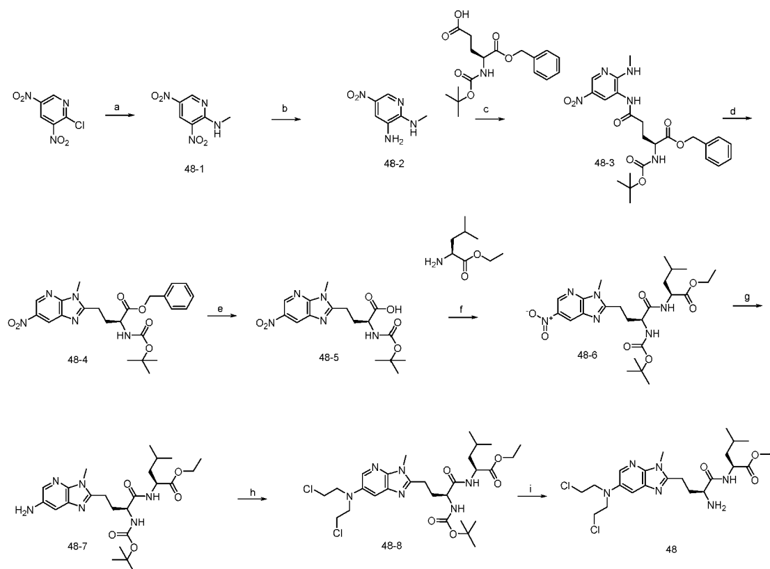
Scheme 14
