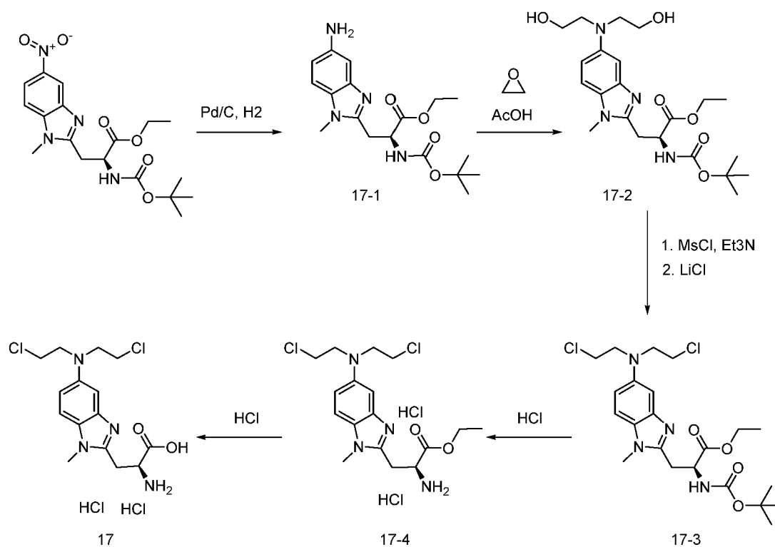
Scheme 6
