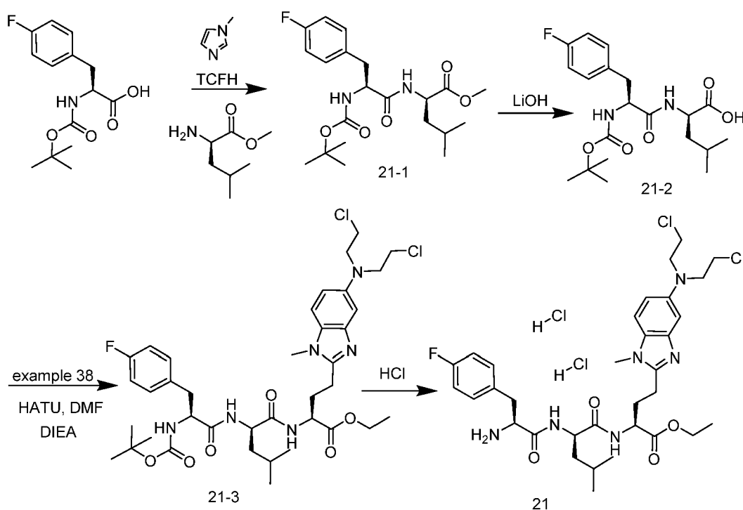
Scheme 8
