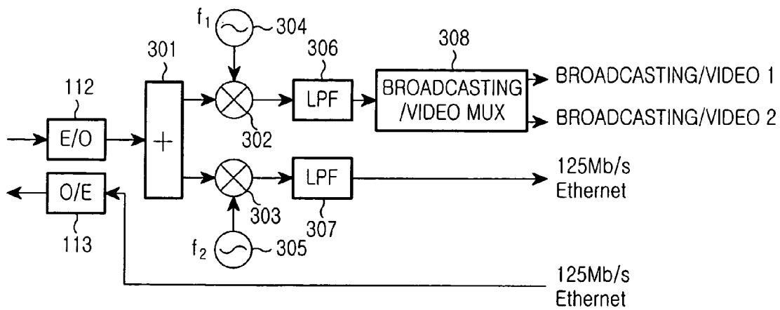
FIG.3 (PRIOR ART)
