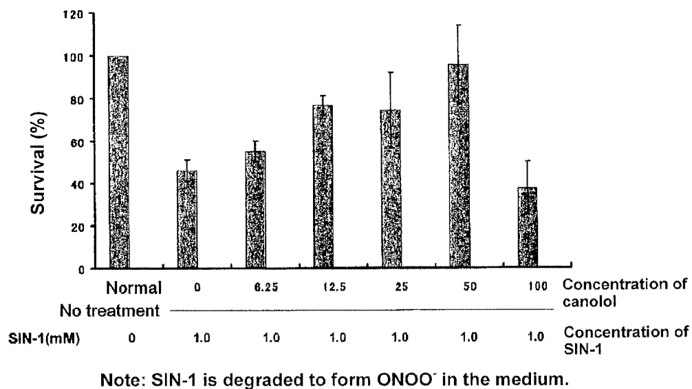
Figure 6 Protective effects of canolol on the cytotoxicity by \text{ONOO}^- in human embryonic kidney cell 293
