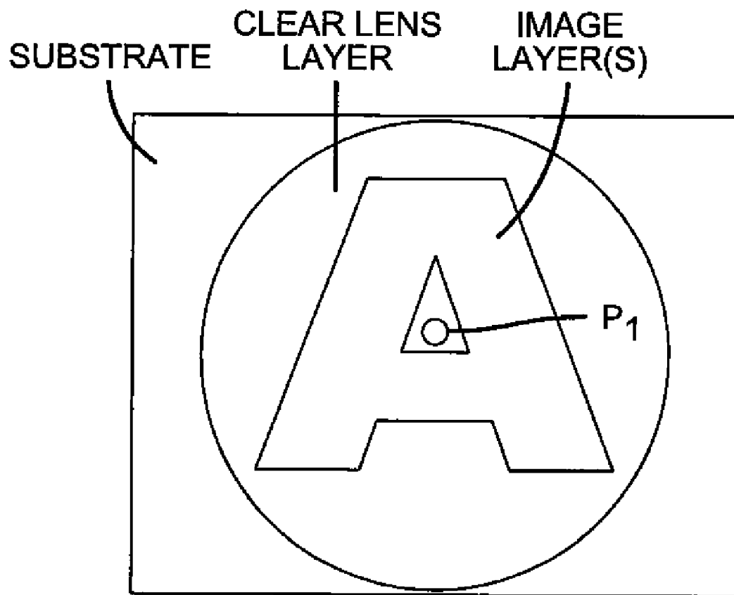
TOP VIEW (CIRCULAR LENS ON SINGLE LETTER)
