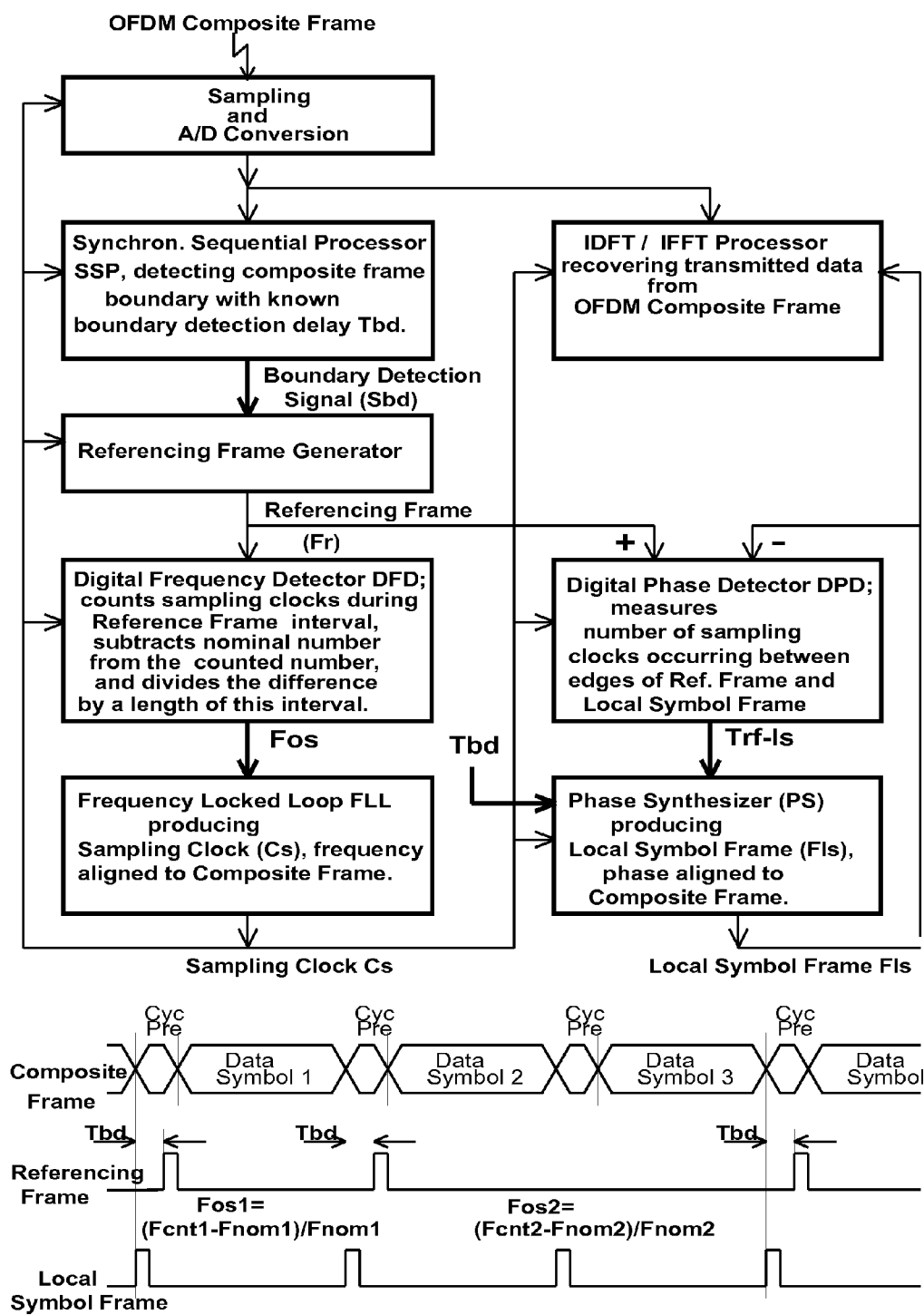
FIG.14 Synchronization System with Improved Stability
