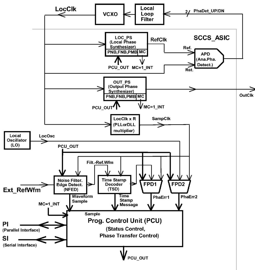
FIG.1 Open Ended Configuration of SCCS
