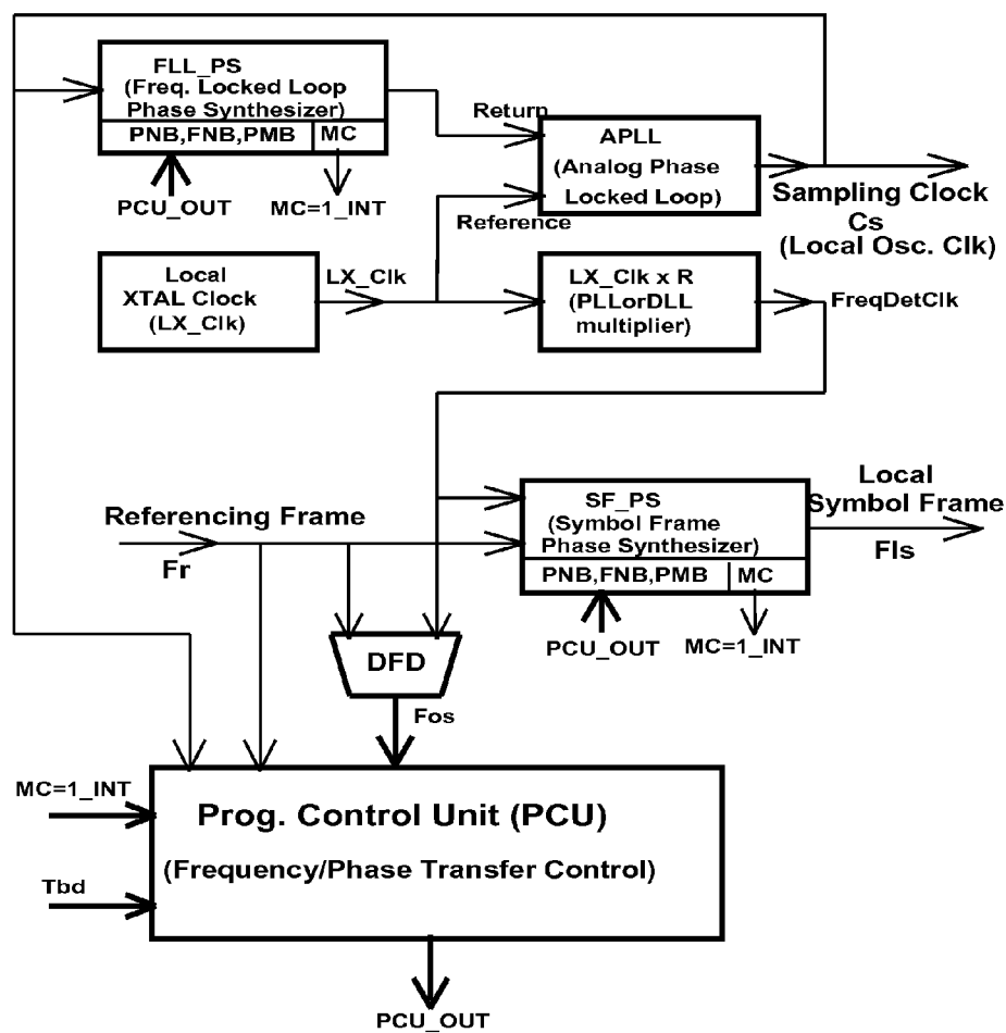
FIG.16 FLPS with Freq. Detector using XTAL clock
