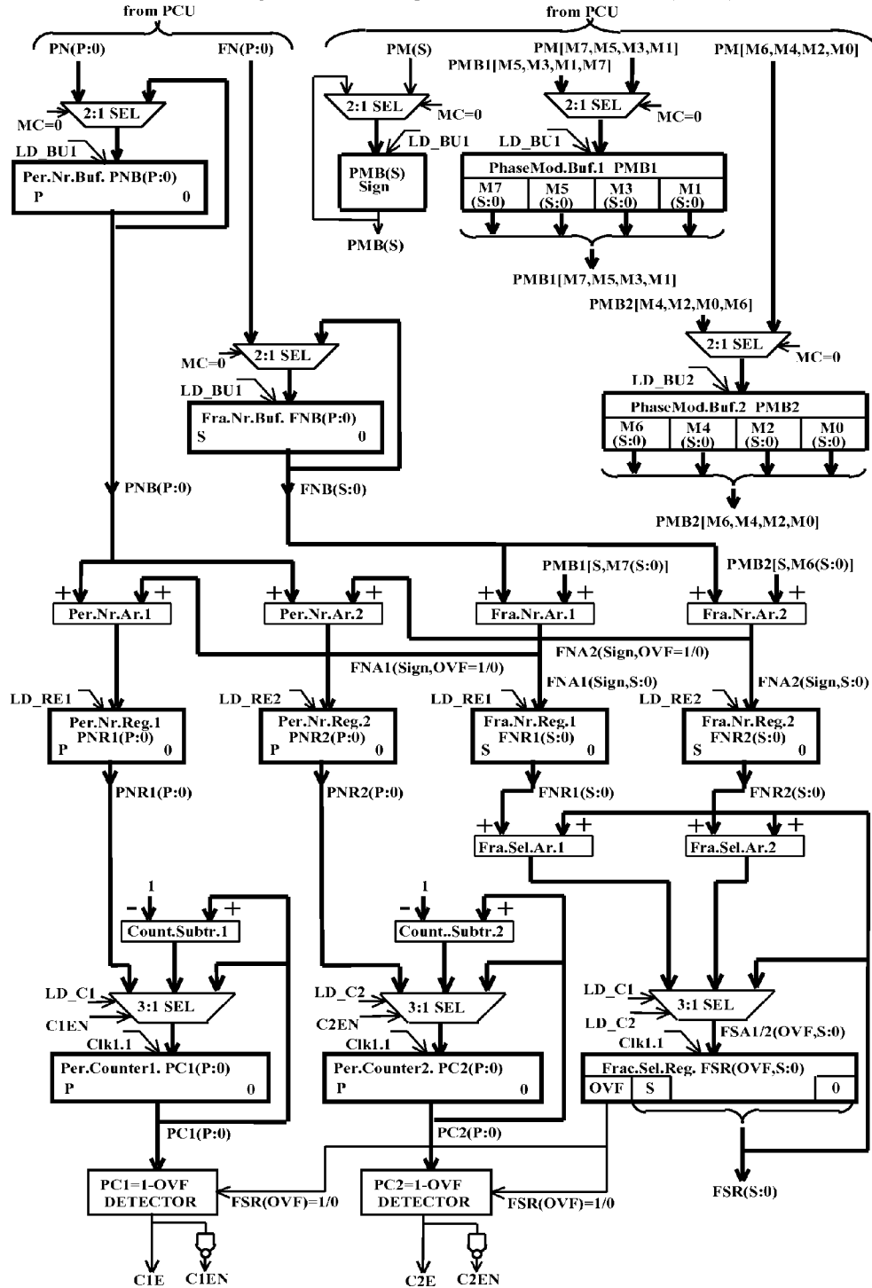
FIG. 6 Synchronous Sequential Phase Processor (SSPP)
