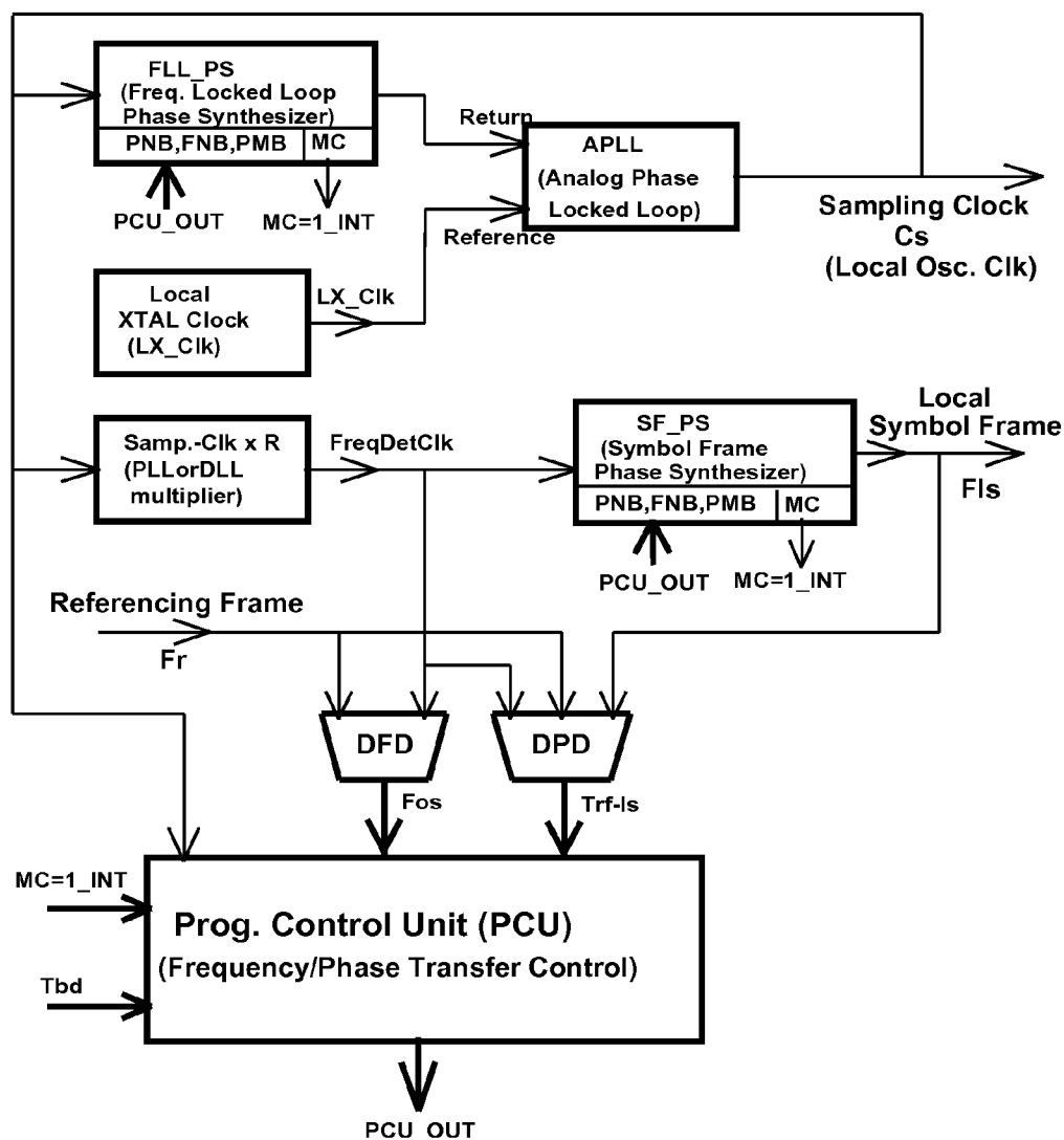
FIG.17 FLPS with Improved Stability
