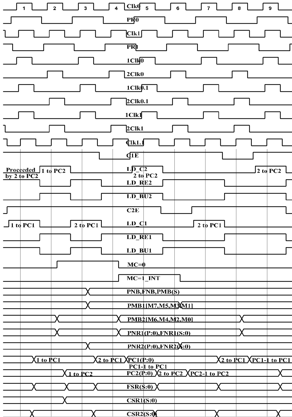
FIG. 7 Timing Diagram of Phase Synthesizer
