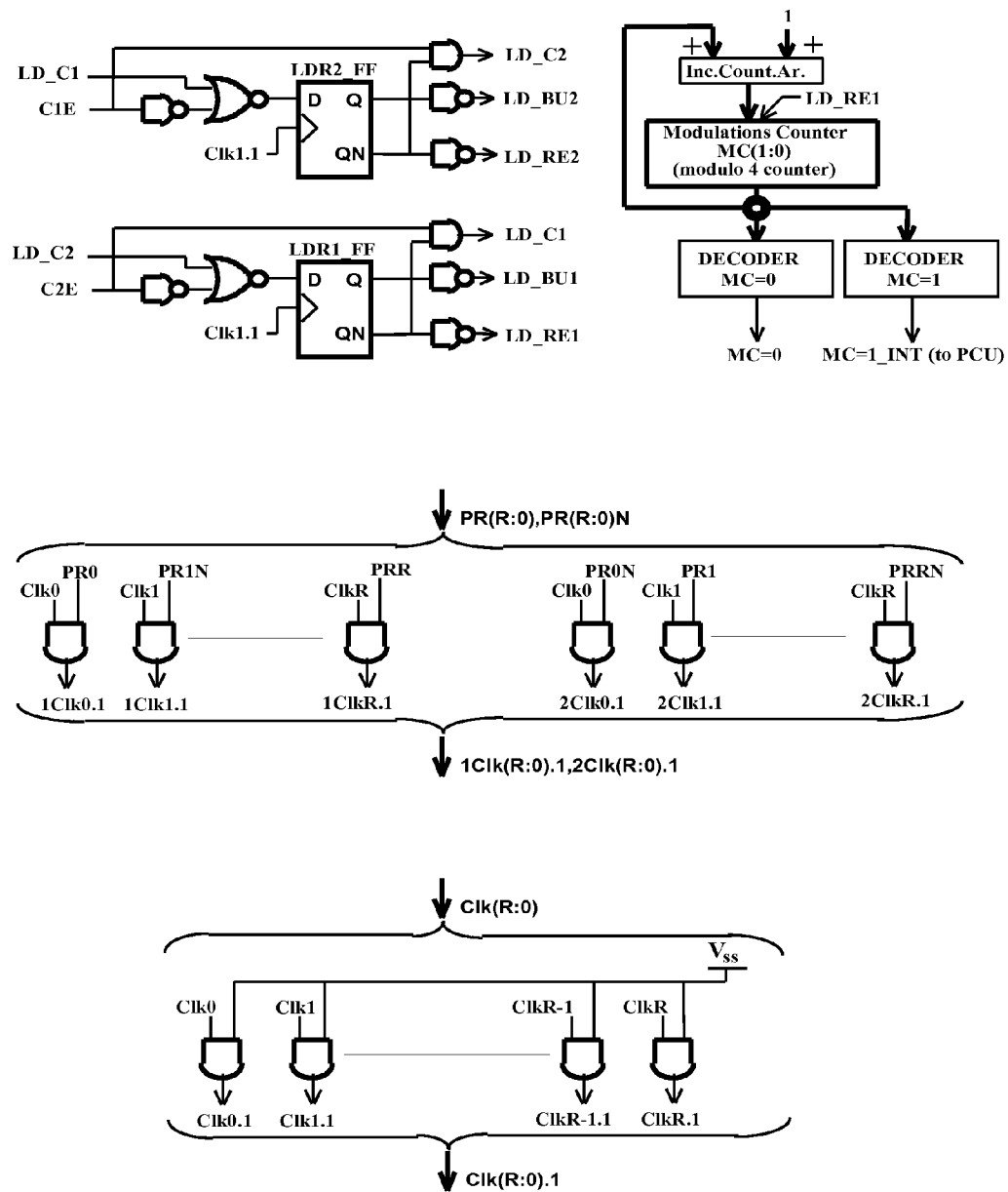
FIG.5 Timing Control (TC) and Clocks Equalization (CE)
