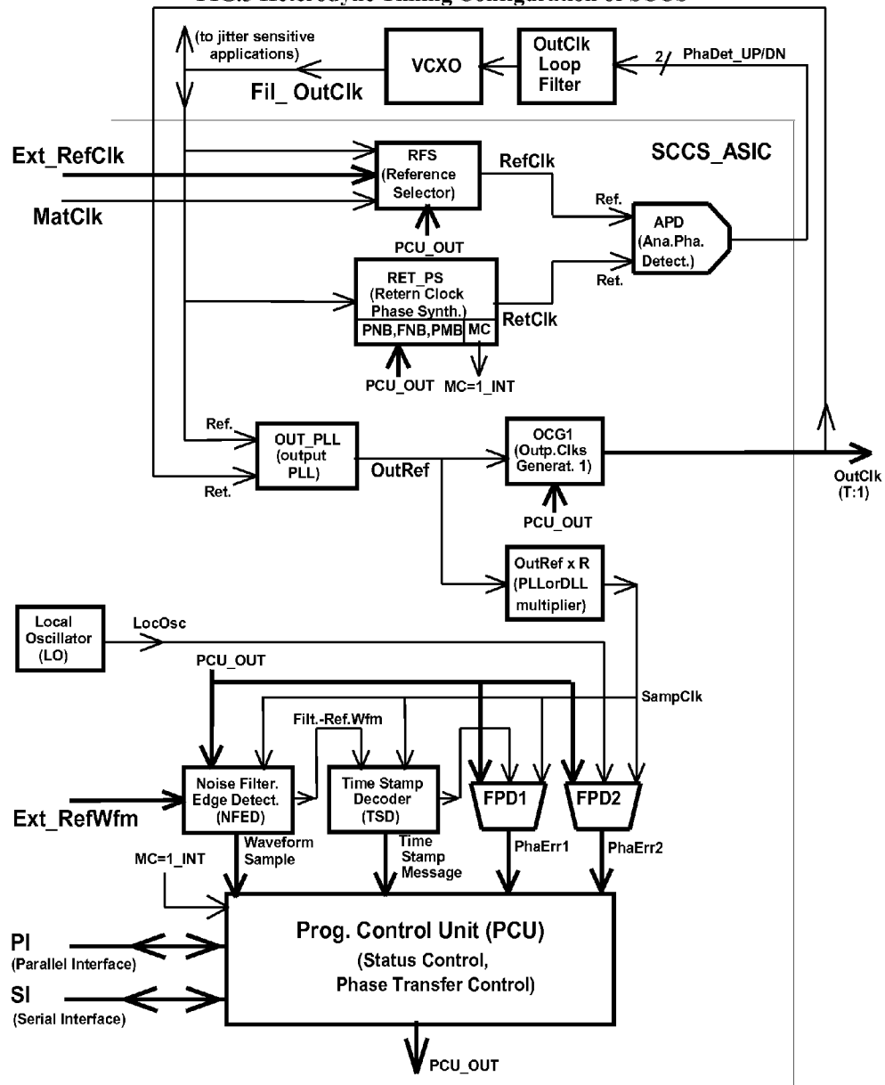
FIG.3 Heterodyne Timing Configuration of SCCS
