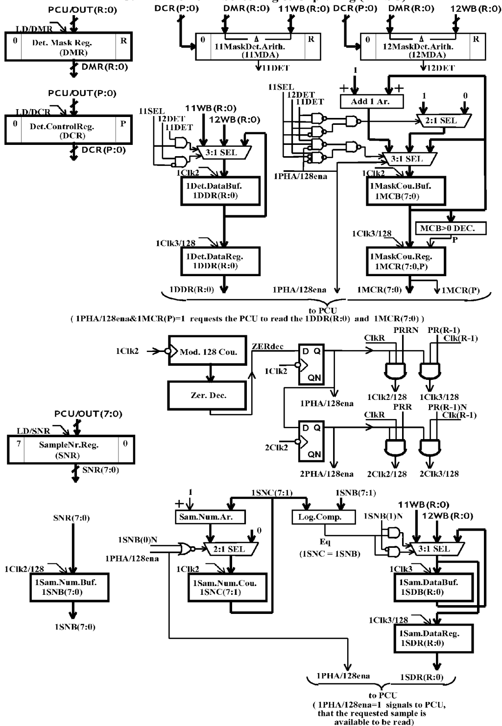
FIG.11 Wave Form Screening & Capturing (WFSC)
