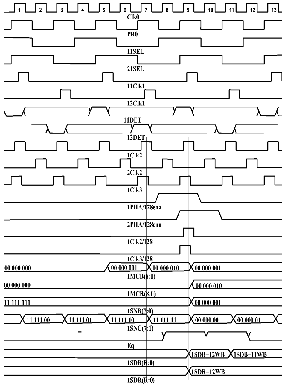
FIG.12 Timing Diagrams of the WFSC
