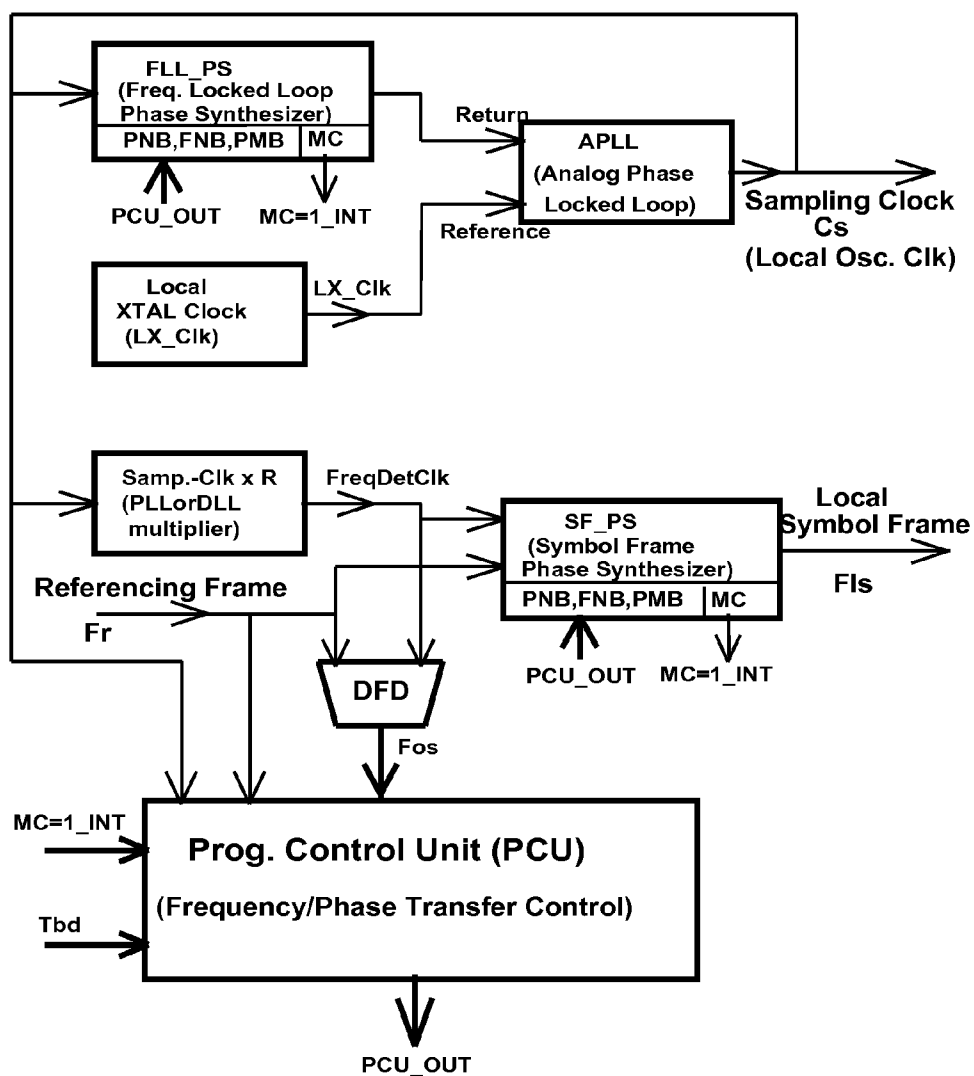
FIG.15 Inherently Stable FLPS
