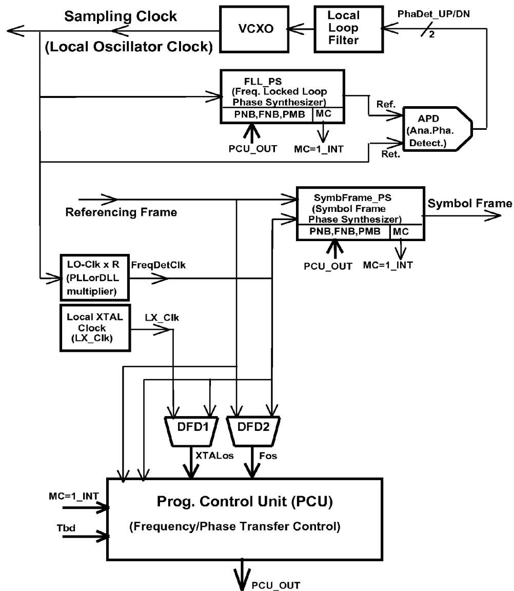
FIG.18 High Accuracy FLPS
