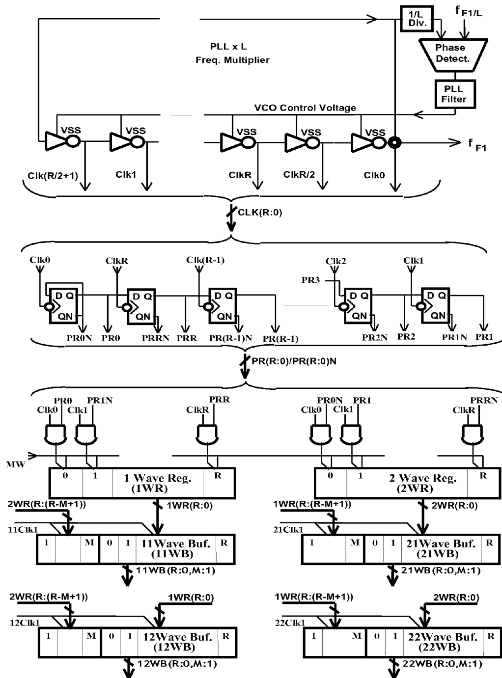
FIG.8 Wave Capturing including Edge Regions (WCER)
