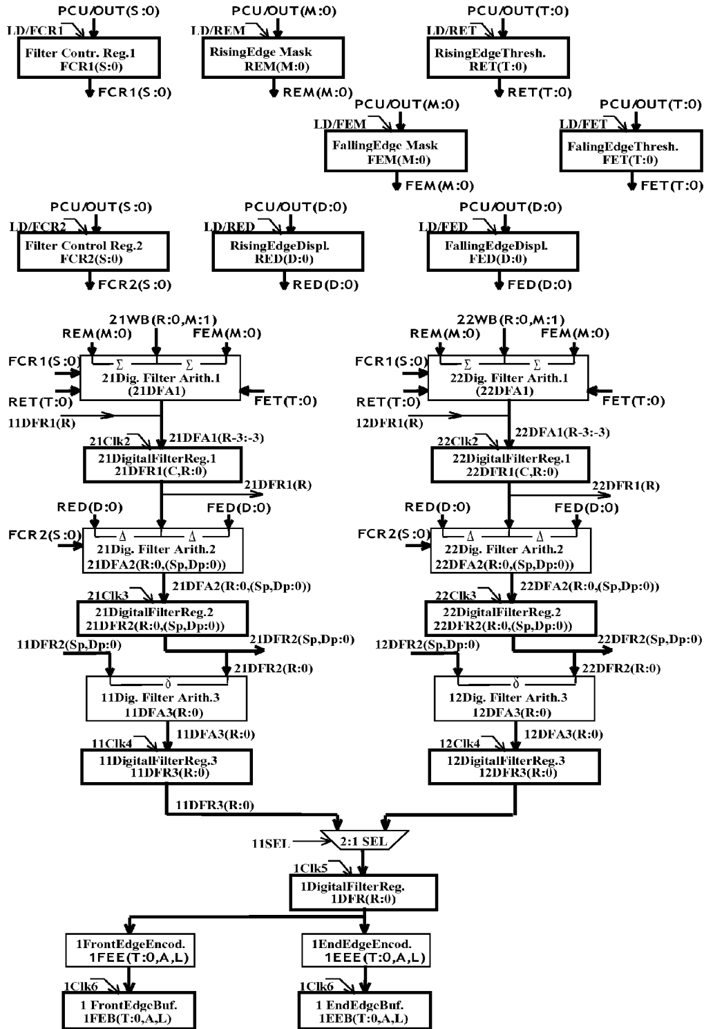
FIG.10 Noise Filtering Edge Detectors (NFED)
