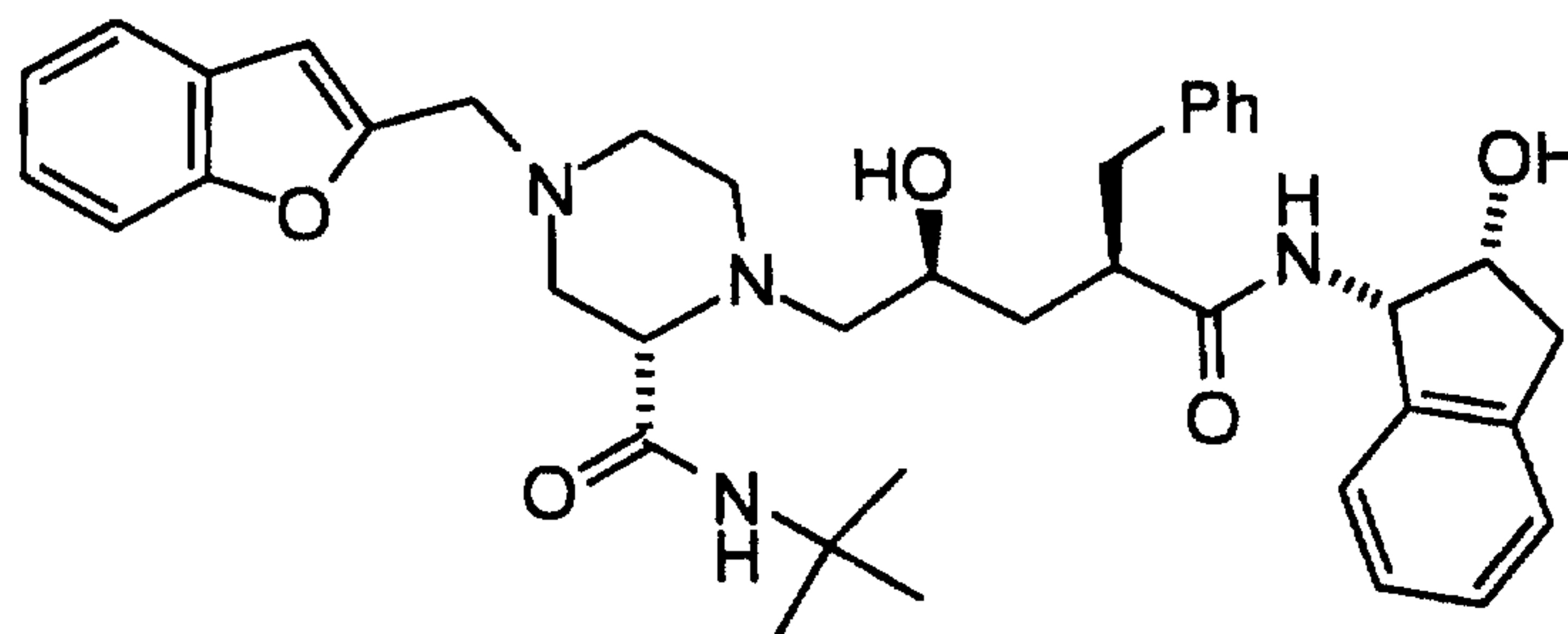
Compound A
