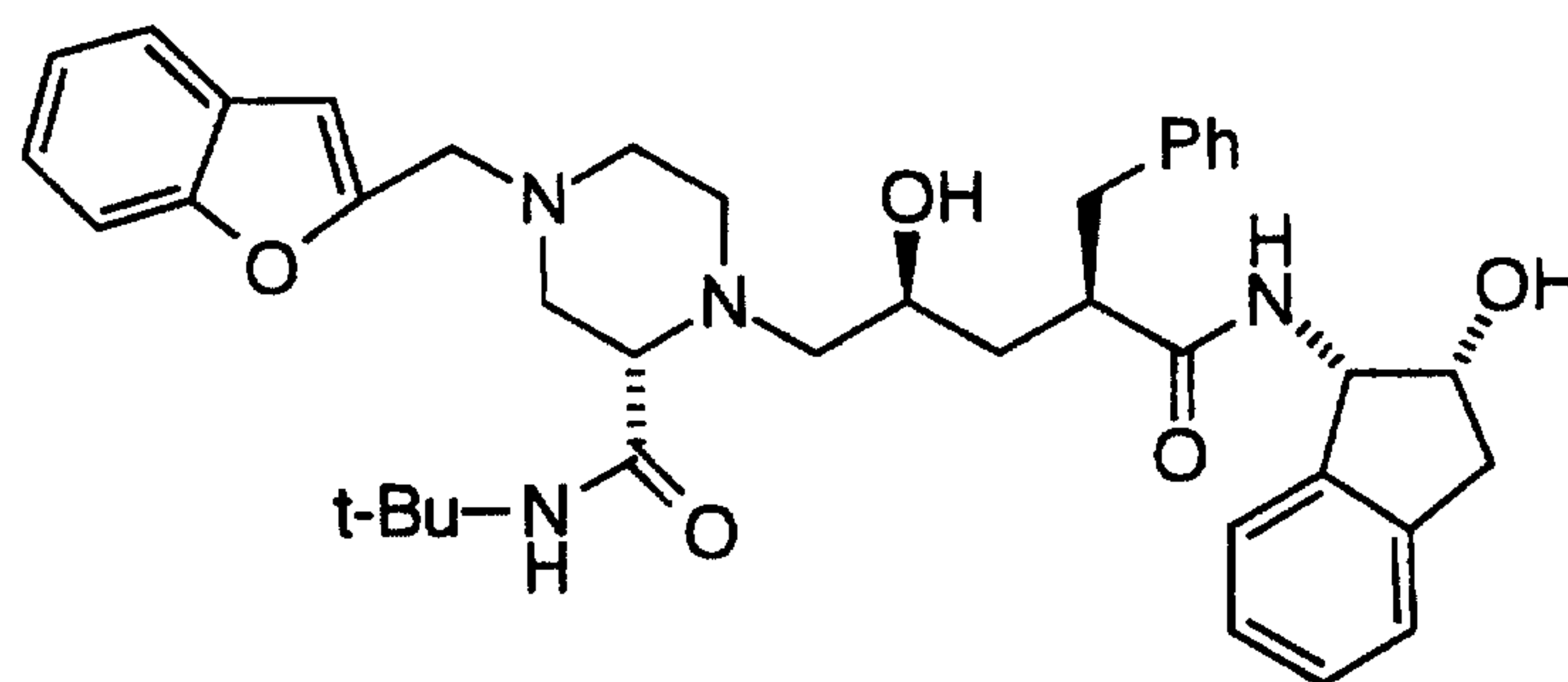
Compound A•sulfate
