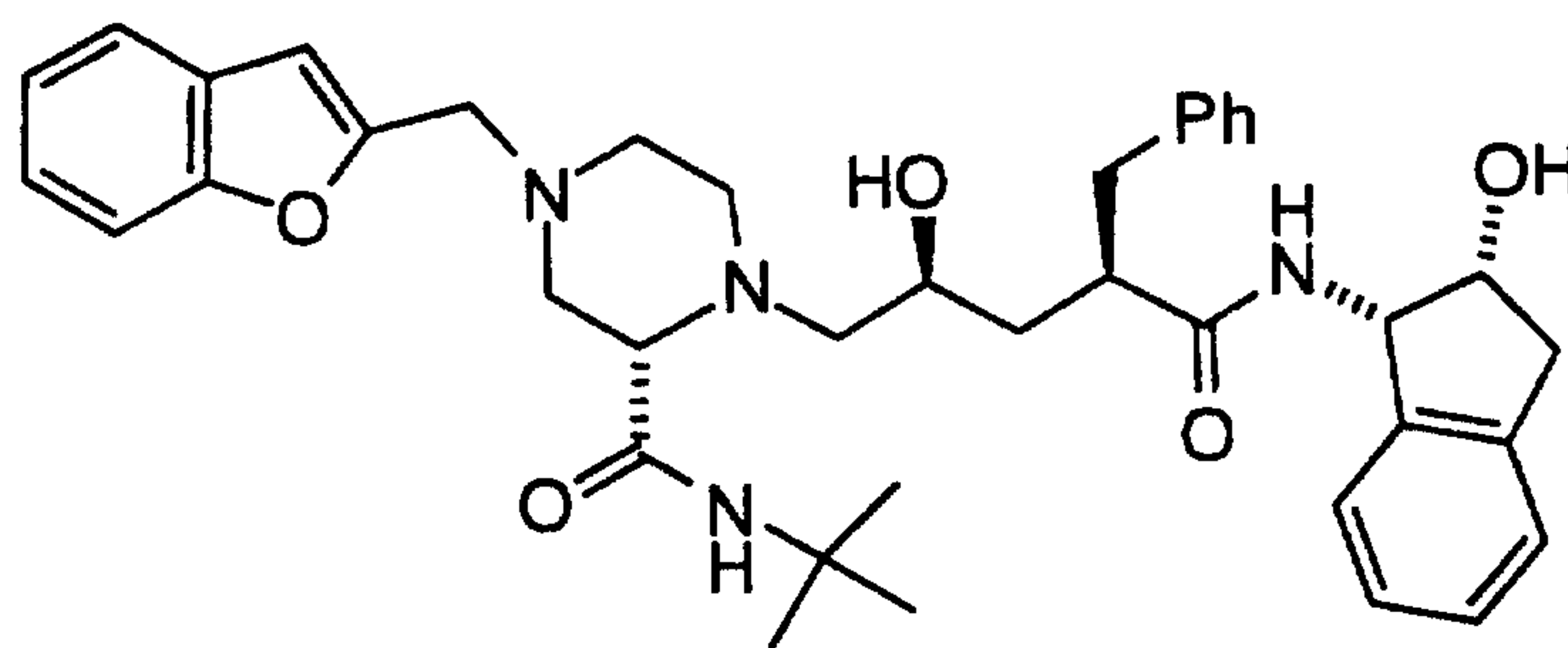
Compound A
