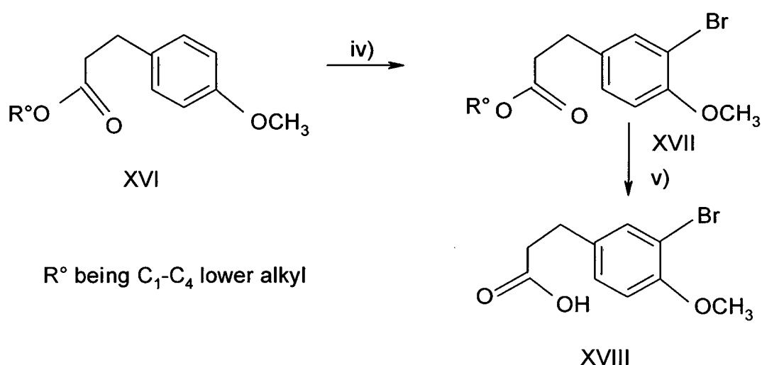
Reaction scheme 2
