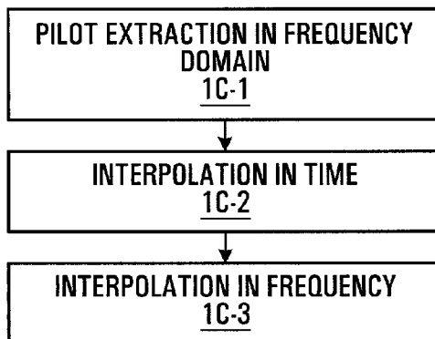
FIG. 1C (PRIOR ART)
