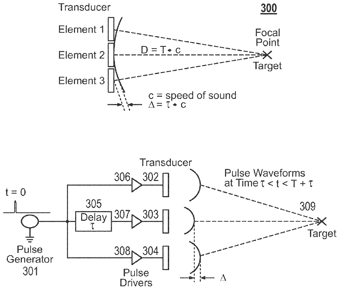
Conventional Transmit Beamforming Single Focal Point
