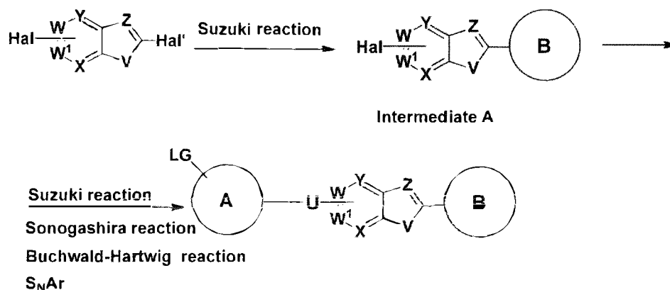
Scheme 6
