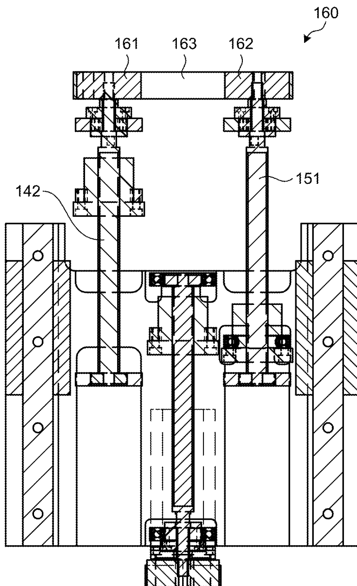
CROSS-SECTION D-D
