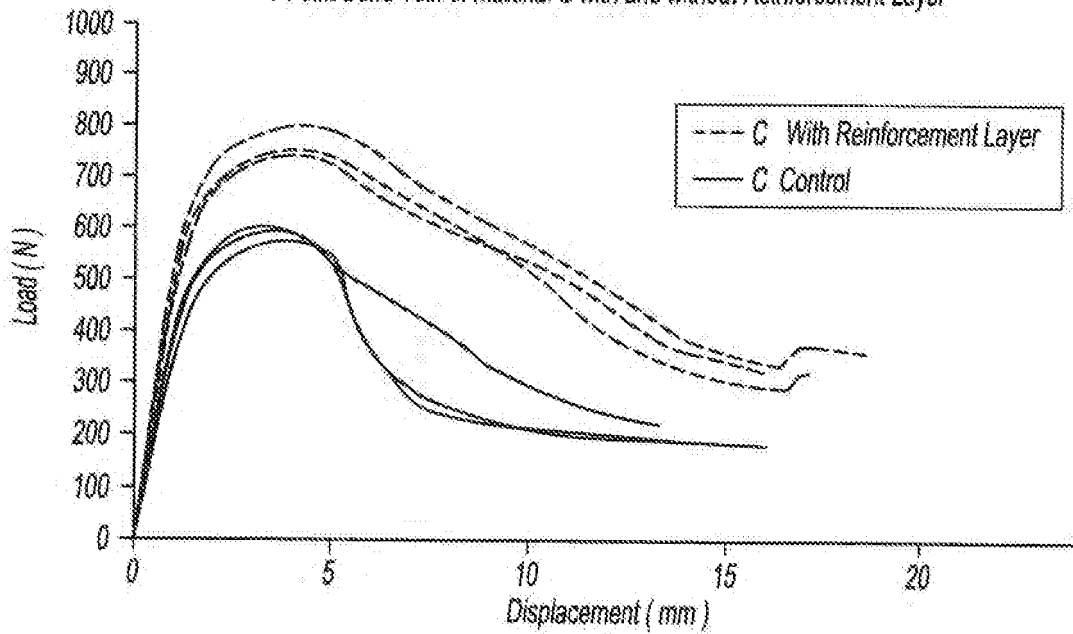
Flexural Testing Load Displacement Curves for Material C
