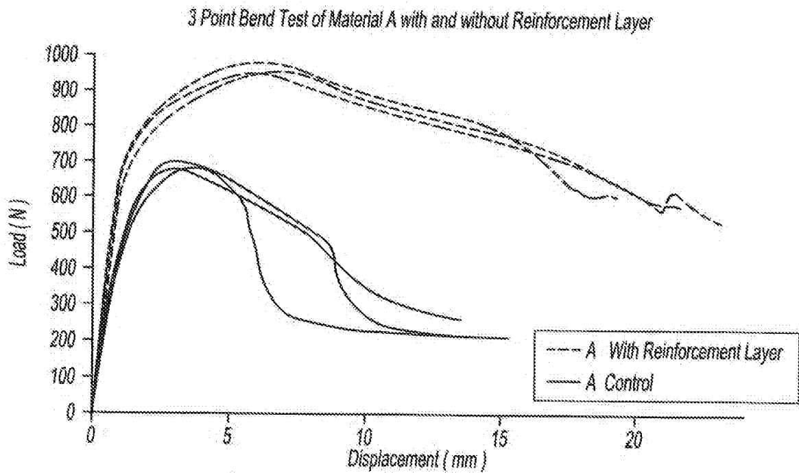
Flexural Testing Load Displacement Curves for Material A
