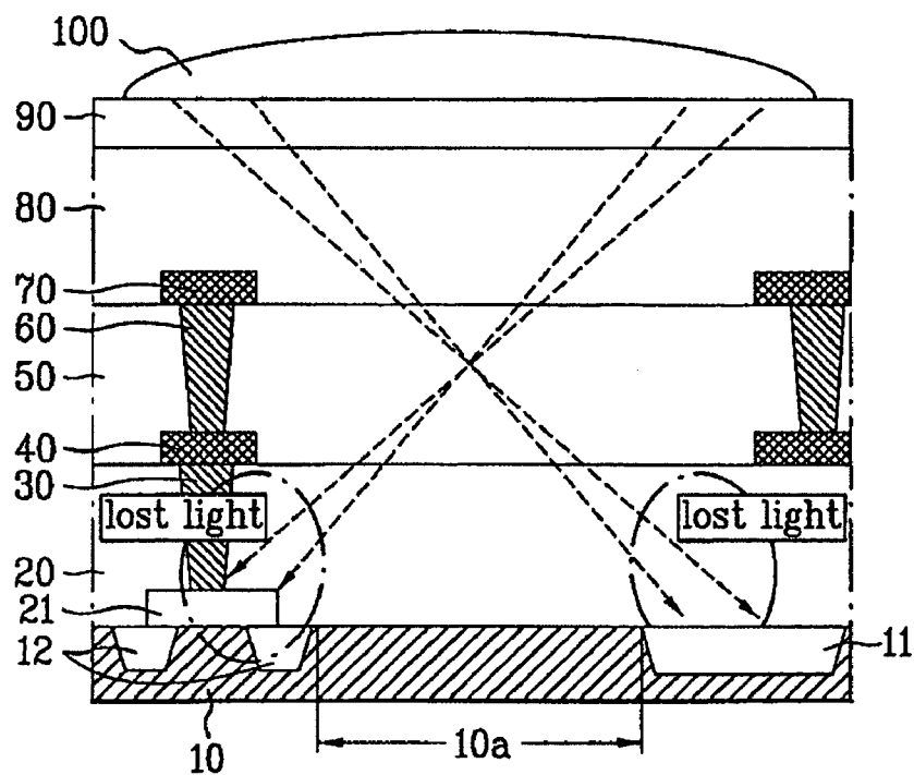
FIG. 1 Related Art
