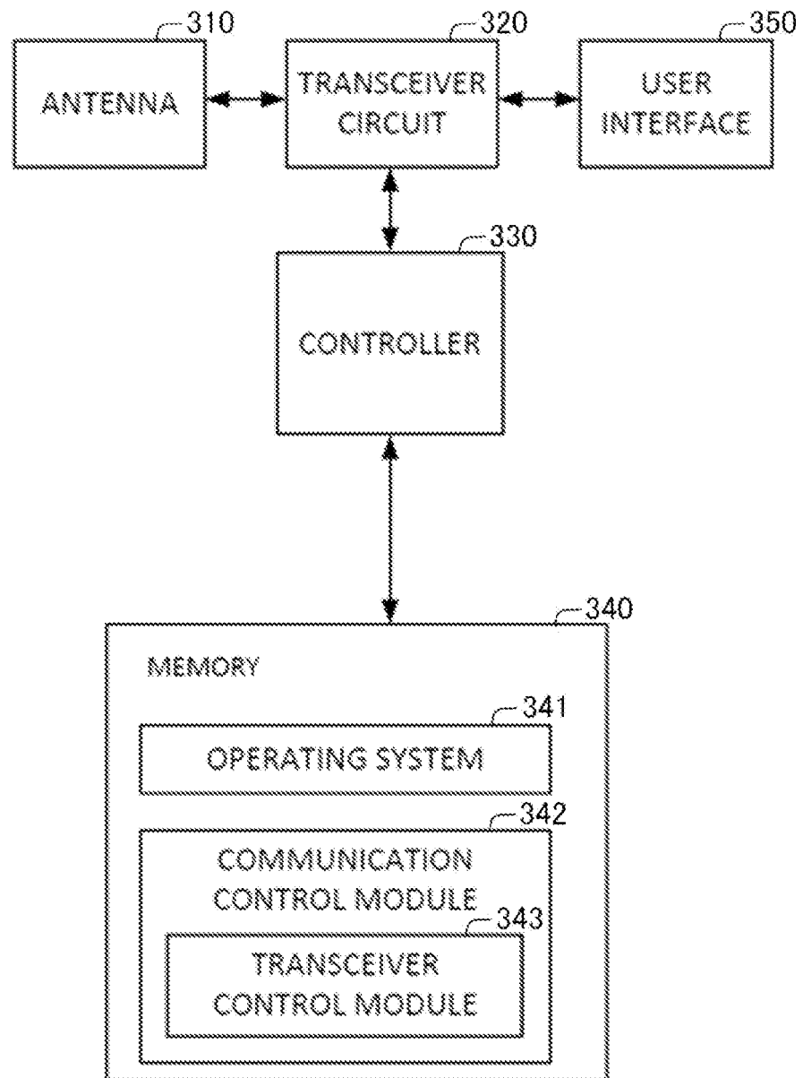
Figure 5: General block diagram for UE 30
