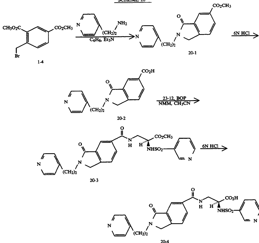
SCHEME 20
