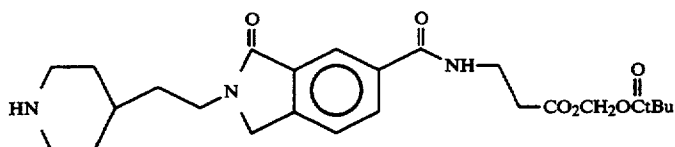
1-H-Isoindole-5-carboxamide, 2,3-dihydro-N-[2-(t-butylcarbonyloxymethylcarboxy)ethyl]-2-[2-(4-piperidinylethyl)ethyl]-3-oxo (1-16)
