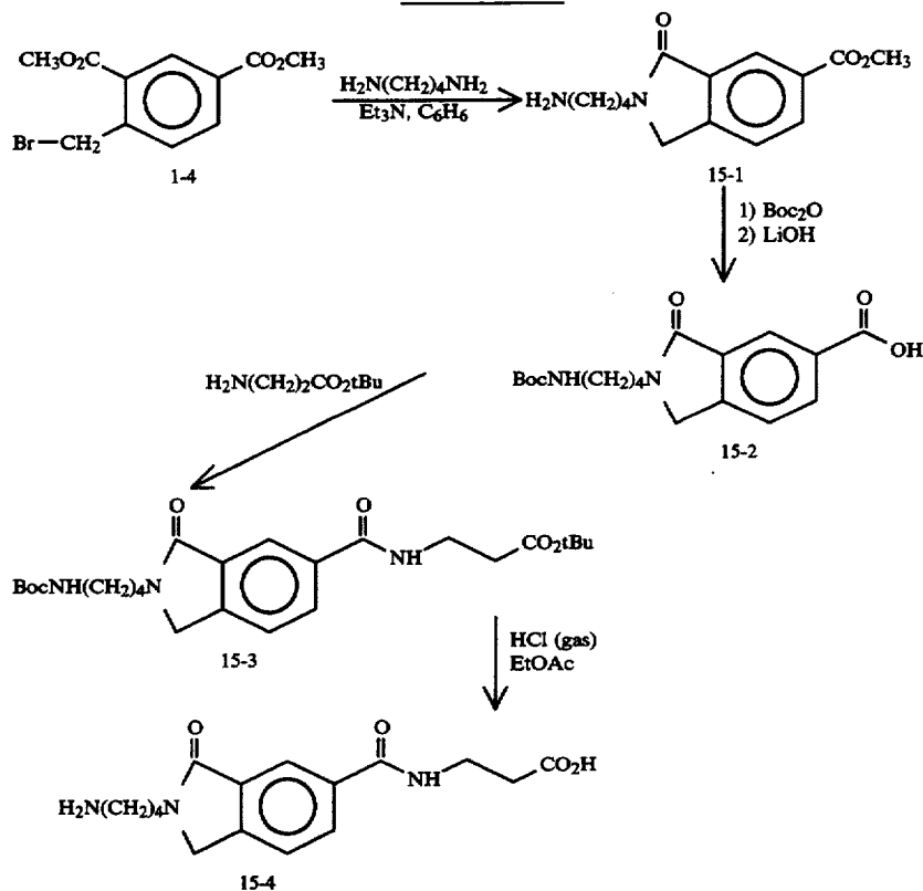
SCHEME 15
