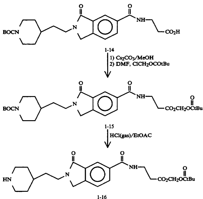
1H-Isoindole-5-carboxamide, 2,3-dihydro-N-[2-(t-butylcarbonyloxymethylcarboxy)ethyl]-2-[2-(4-N-t-butyloxycarbonylpiperidinylethyl)ethyl]-3-oxo (1-15)
