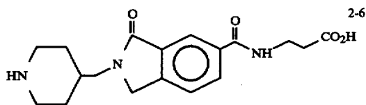
1-H-Isoindole-5-carboxamide, 2,3-dihydro-N-(2-carboxyethyl)-2-[(4-piperidyl)methyl]-3-oxo (2-6)
