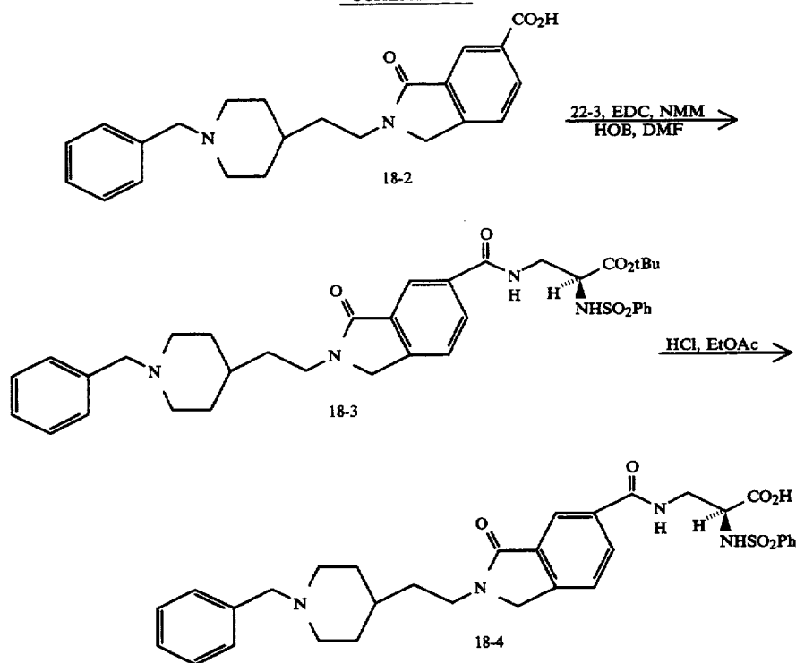
SCHEME 18
