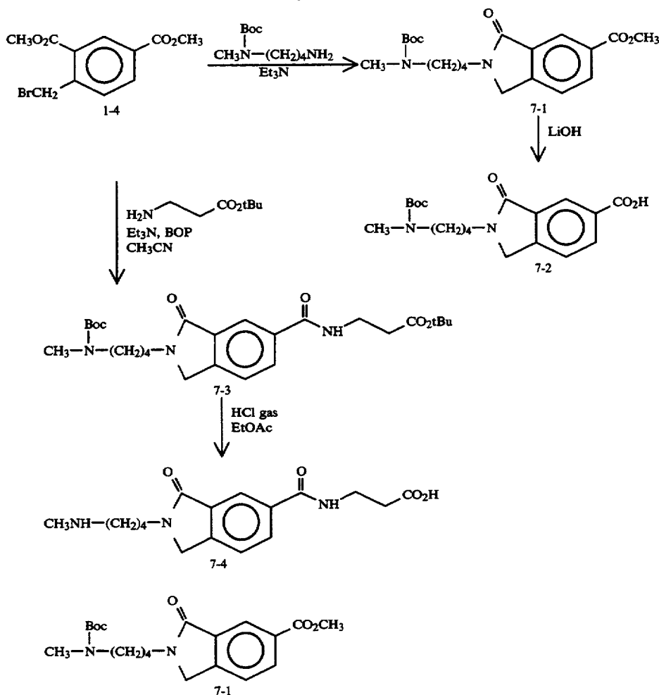
SCHEME 7
