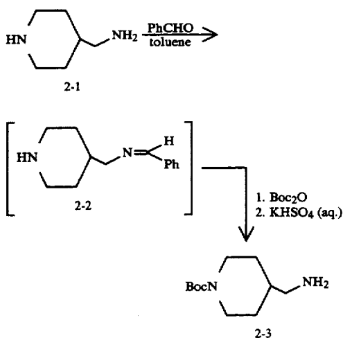
SCHEME 2
