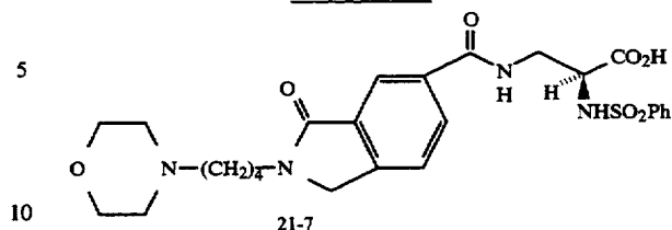
-continued SCHEME 21
