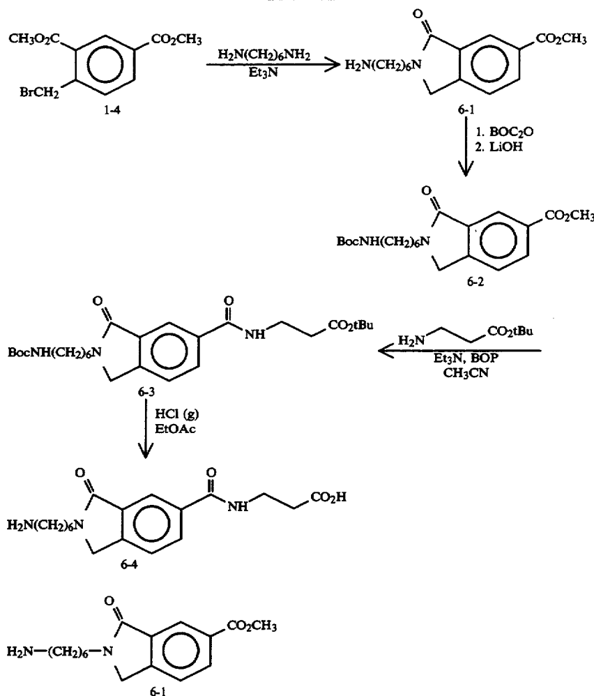
SCHEME 6
