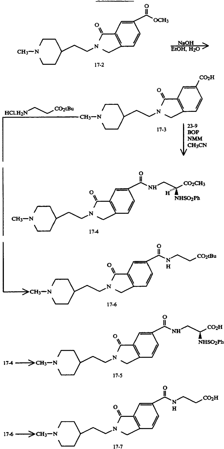
SCHEME 17
