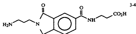
1-H-Isoindole-5-carboxamide, 2,3-dihydro-N-(2-carboxyethyl)-2-[3-aminopropyl]-3-oxo (3-4)
