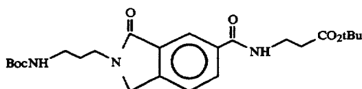
1-H-Isoindole-5-carboxamide, 2,3-dihydro-N-[2-(t-butyloxycarbonyl)-ethyl]-2-[3-(N-t-butyloxycarbonylamino)propyl]-3-oxo (3-3)
