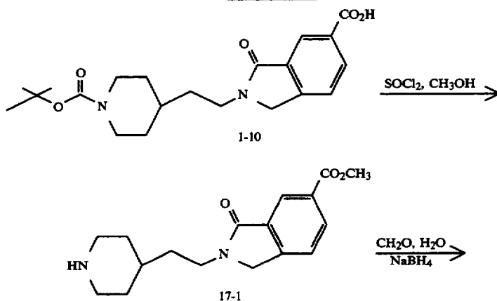
SCHEME 17
