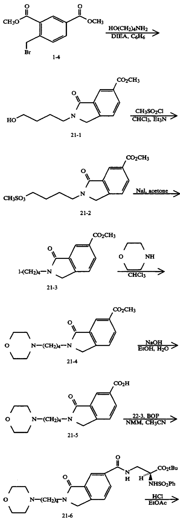
SCHEME 21
