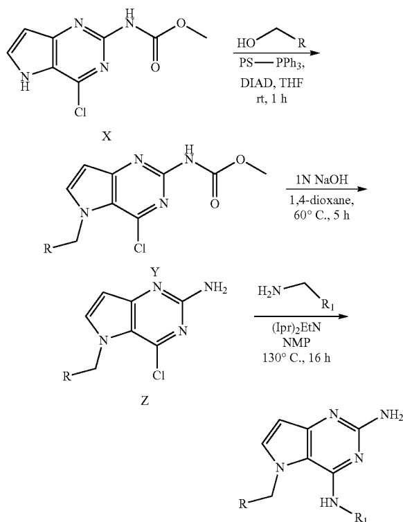
Scheme 2. Overall reaction scheme
