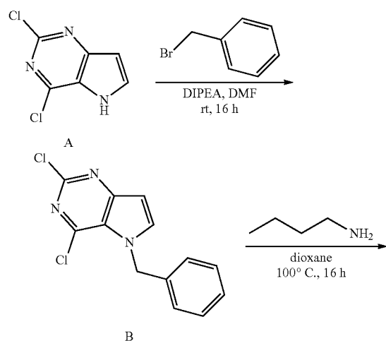
Scheme 1. Overall reaction scheme
