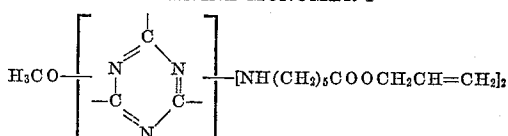
TRIAZINE MONOMER I
