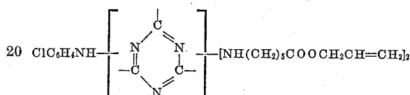
TRIAZINE MONOMER VI
