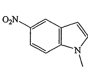
5-Nitroindole
