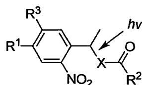
o-nitrobenzyl
