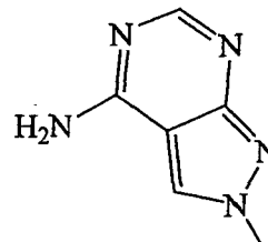
N 8 -8aza-7deazaadenine
