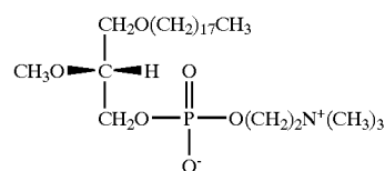
Formula I: L-EL (1-O-octadecyl-2-O-methyl-sn-glycero-3-phosphocholine)
