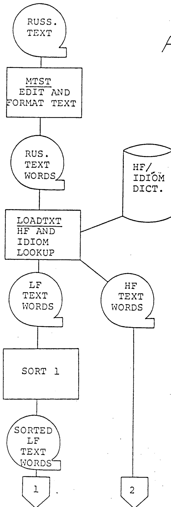
SYSTRAN 360/65 Operation FLOW DIAGRAM
