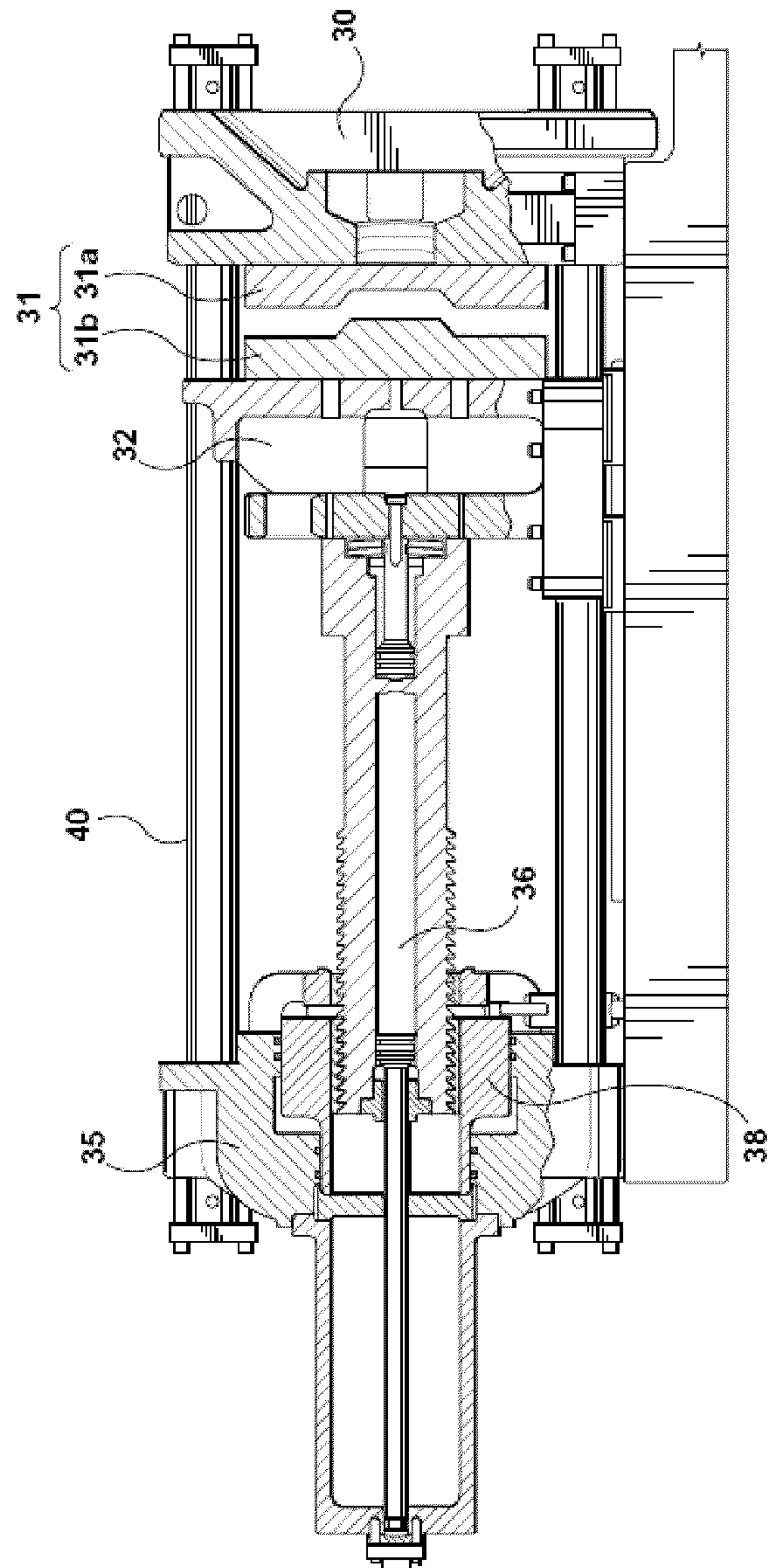
FIG. 2 (PRIOR ART)
