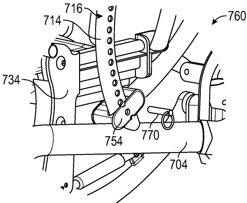
DETAIL K
