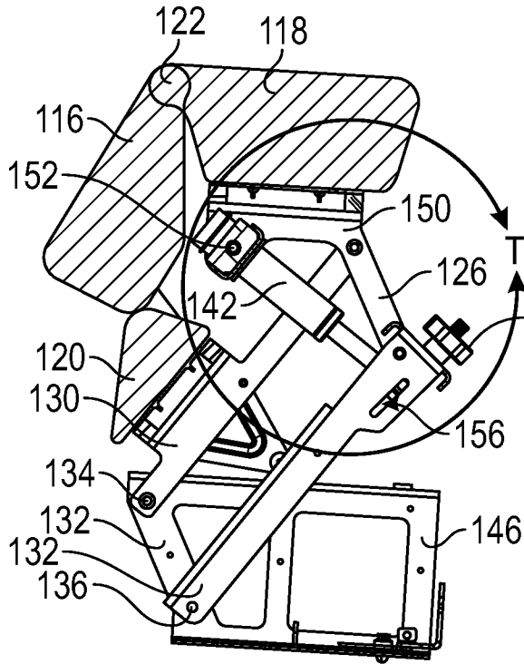
SECTION 17-17 FIG. 17A
