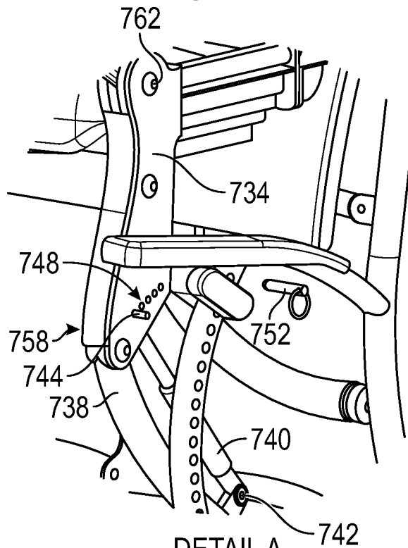
DETAIL A SCALE 1:5 FIG. 47B
