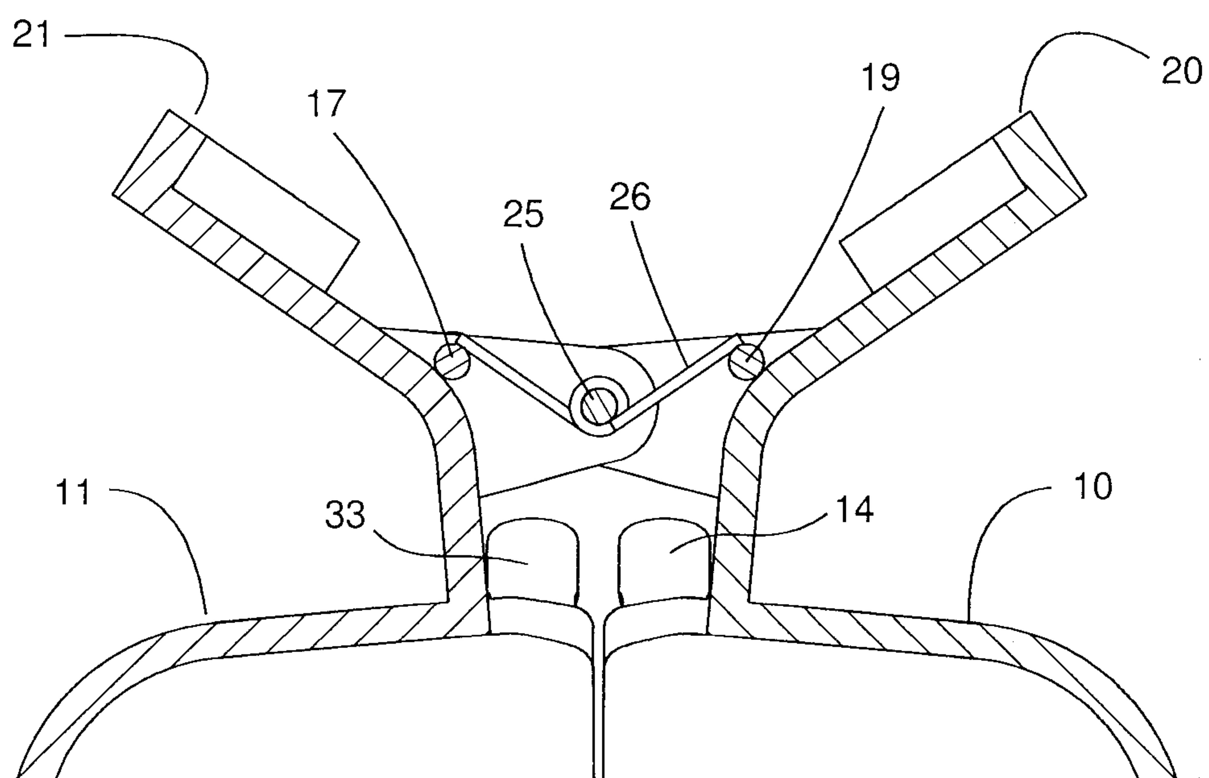
SECTION E-E
