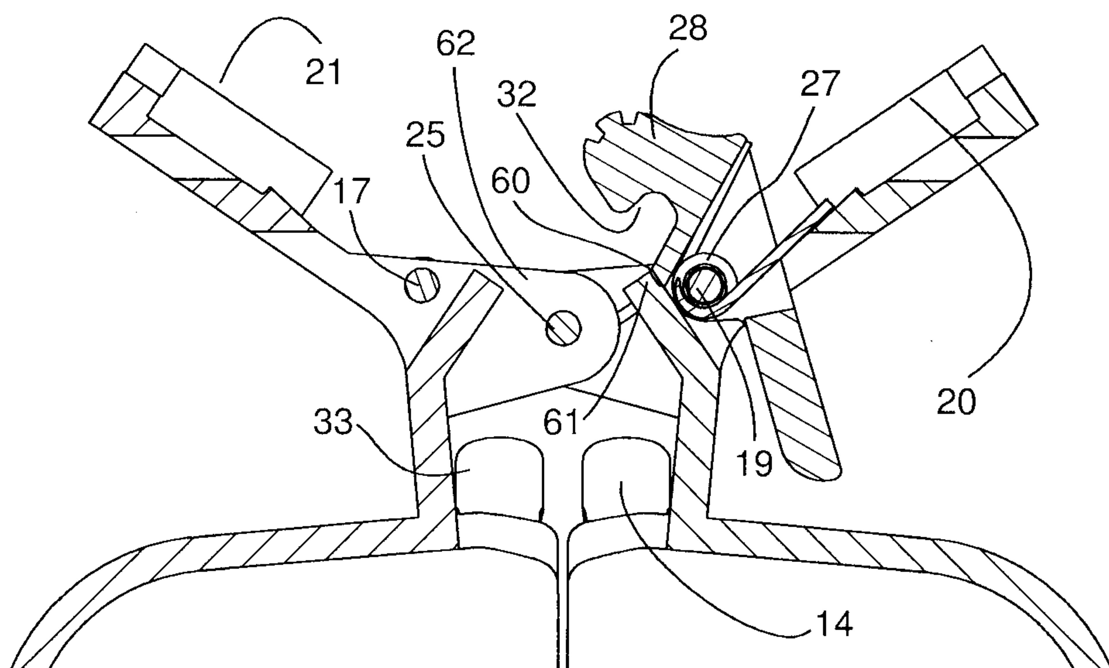
SECTION B-B
