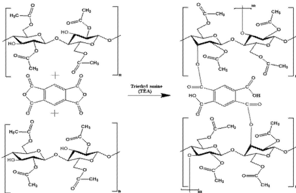
Scheme 1. Crosslinking of Cellulose Acetate with PMDA.
