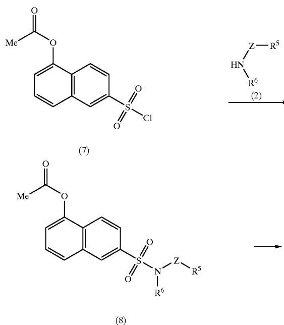
<<Reaction Scheme 2>>
