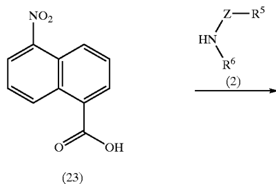
<Reaction Scheme 6>
