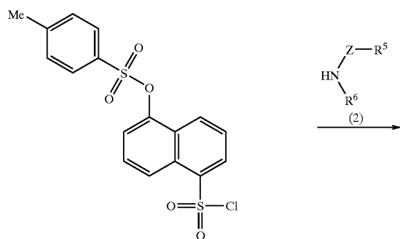
&lt;Reaction Scheme 1&gt;
