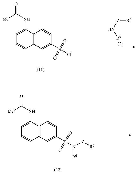
<Reaction Scheme 3>
