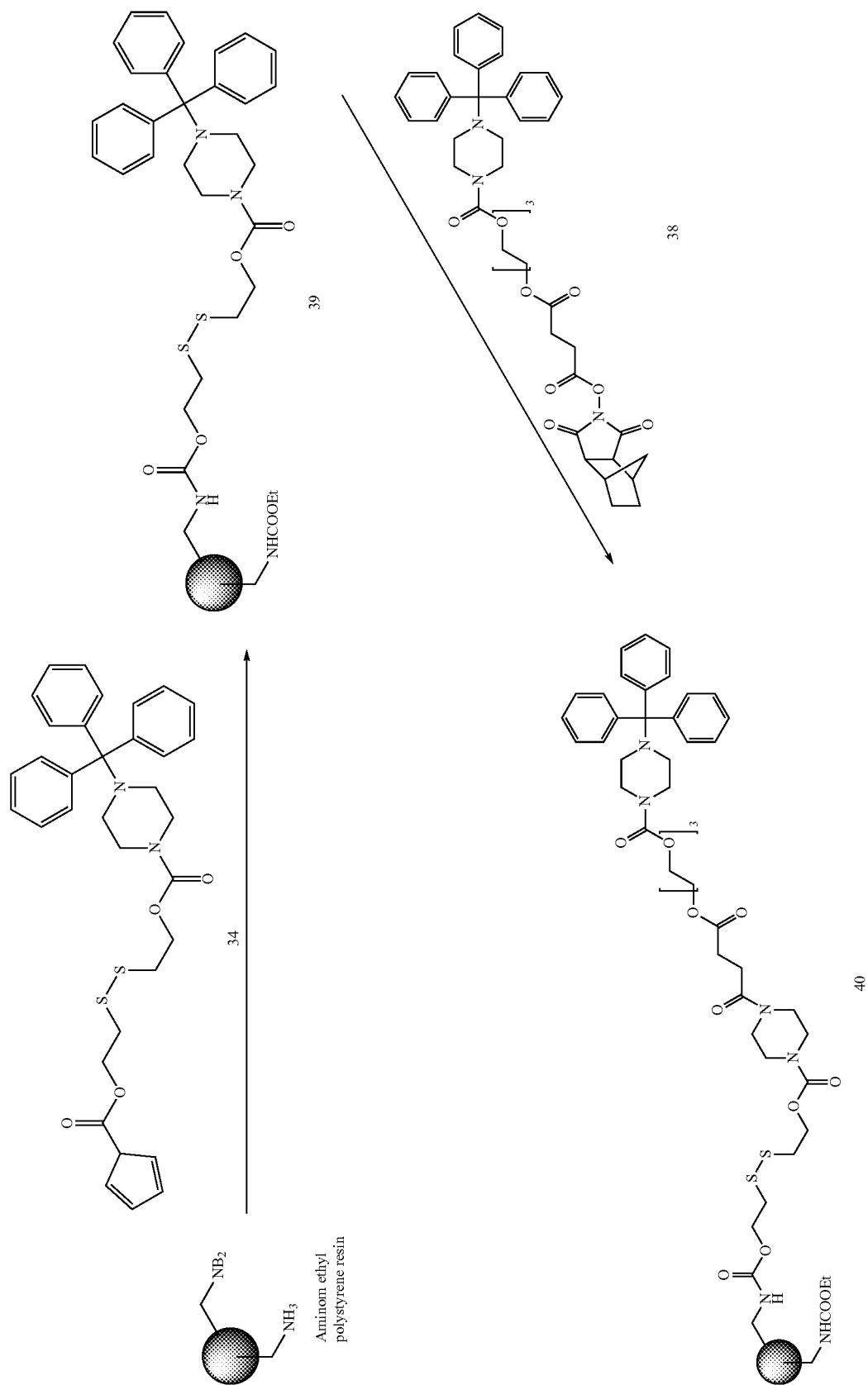
Scheme 3: Preparation of the Solid Support for Synthesis of Morpholino Oligomers
