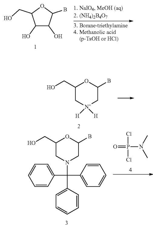
Scheme 1: General synthetic route to PMO Subunits
