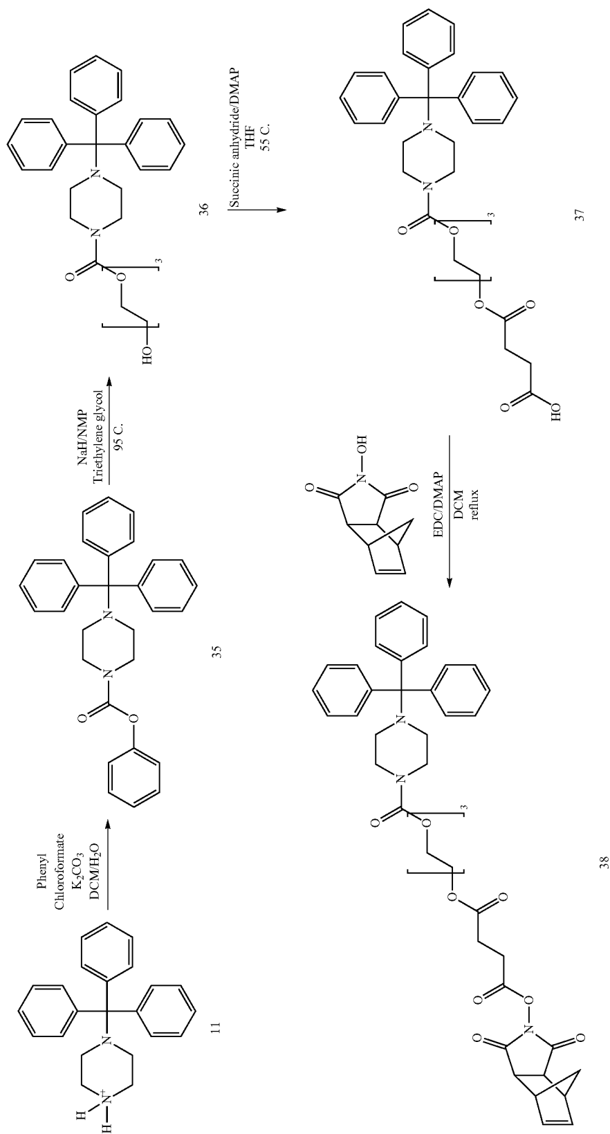
Scheme 2: Preparation of Activated Tail Acid
