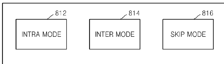
PREDICTION MODE (810)
