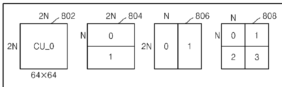
PARTITION TYPE (800)
