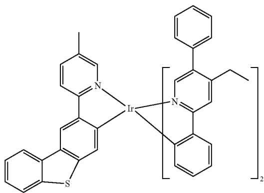
Compound 79
