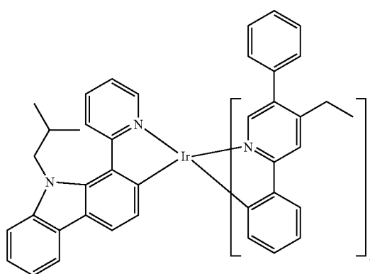
Compound 94
