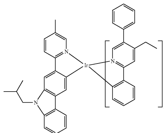
Compound 101
