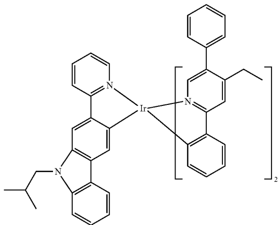
Compound 96
