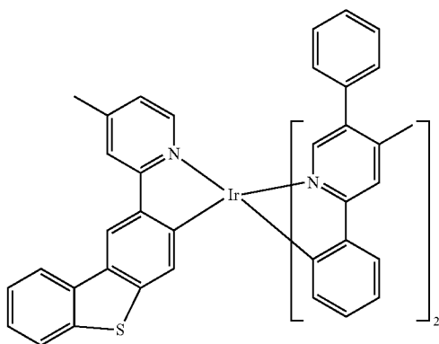
Compound 67
