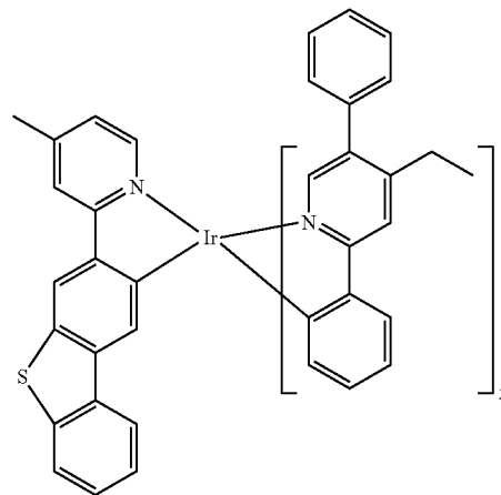
Compound 75
