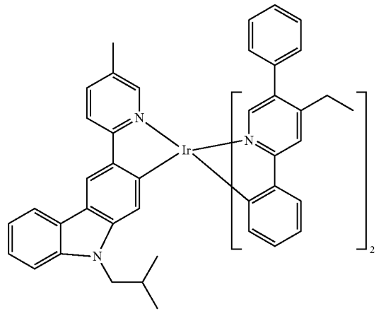
Compound 102
