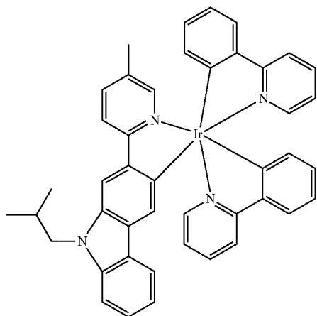
Compound 104
