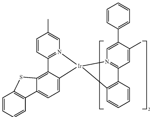
Compound 67
