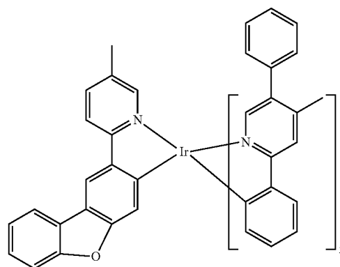
Compound 45
