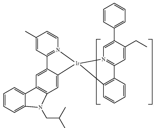
Compound 100
