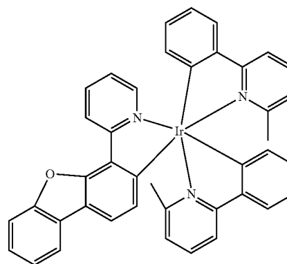
Compound 1
