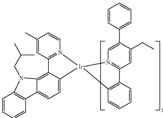
Compound 86
