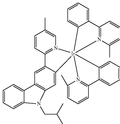
Compound 108
