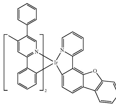
Compound 37
