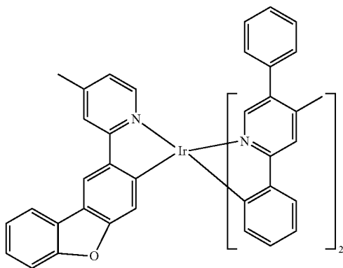
Compound 42
