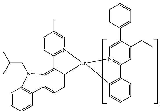
Compound 90
