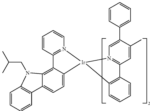
Compound 85
