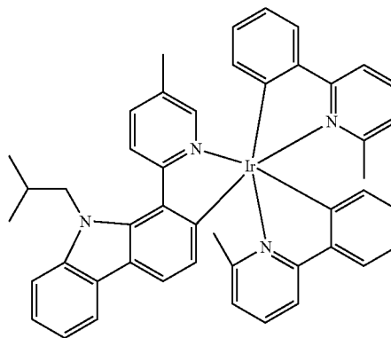
Compound 107
