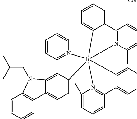
Compound 28
