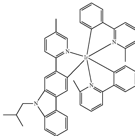
Compound 107
