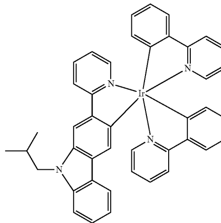
Compound 26
