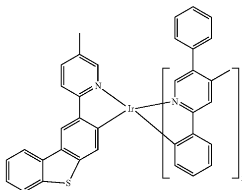
Compound 70
