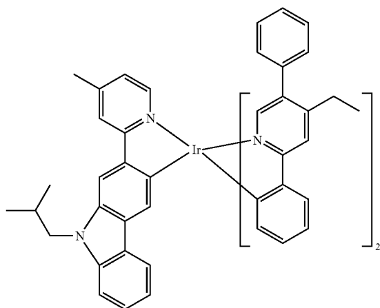
Compound 98
