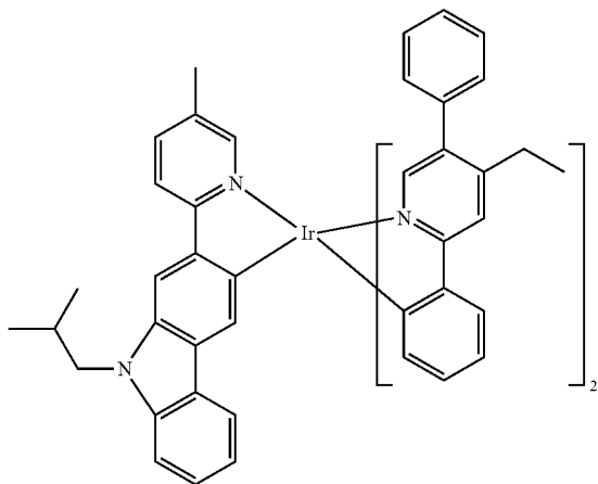
Compound 102
