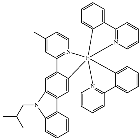
Compound 32
