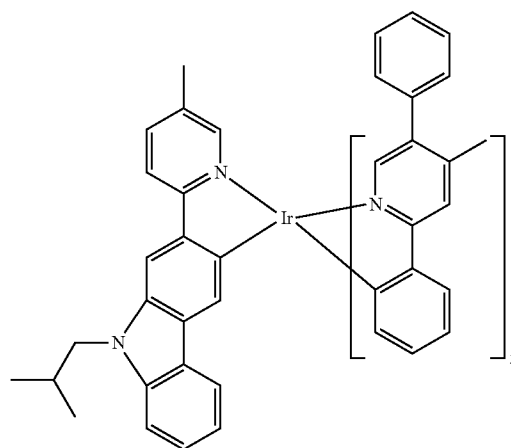
Compound 93
