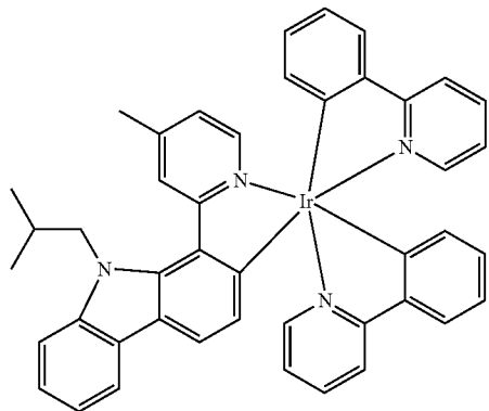
Compound 32
