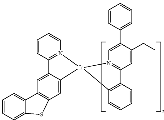
Compound 73
