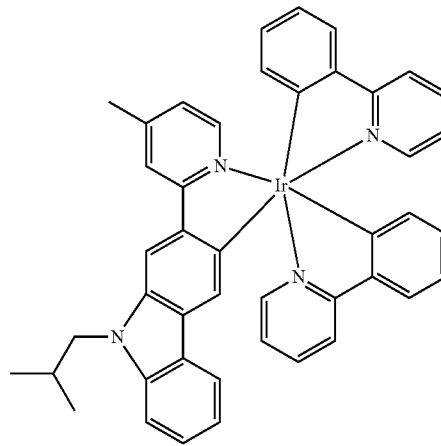
Compound 32
