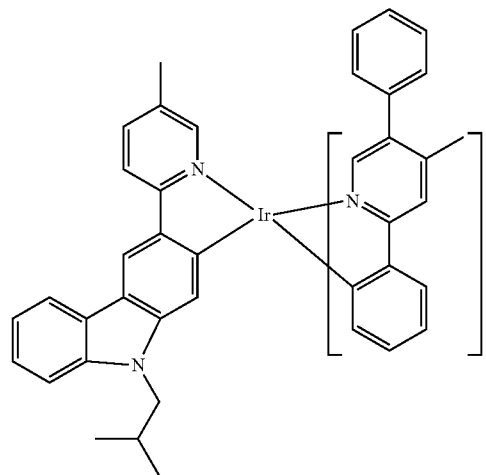
Compound 94
