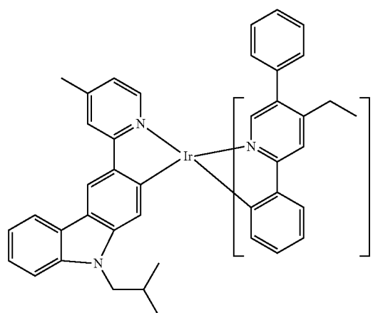
Compound 87
