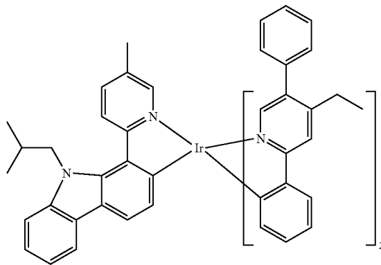
Compound 101
