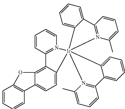
Compound 4
