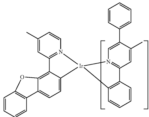
Compound 40
