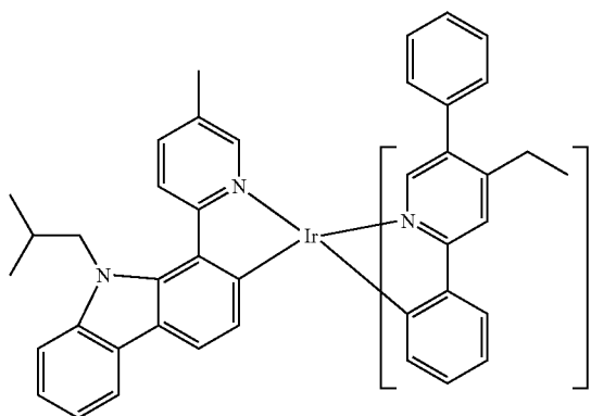
Compound 88
