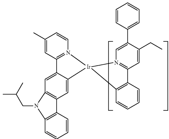
Compound 87
