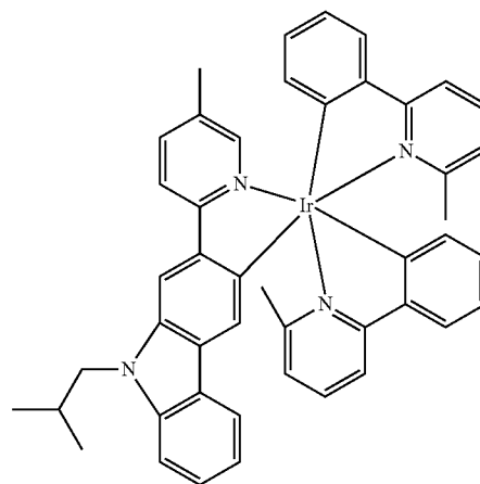
Compound 107
