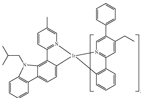
Compound 100
