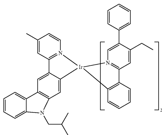
Compound 100
