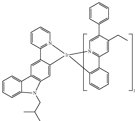
Compound 97
