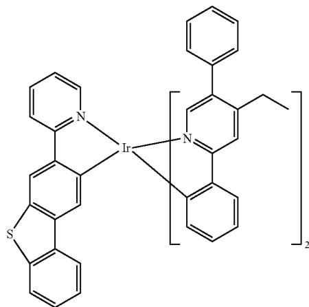
Compound 72
