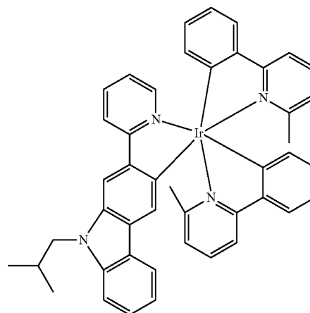
Compound 29
