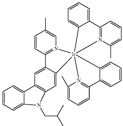
Compound 108
