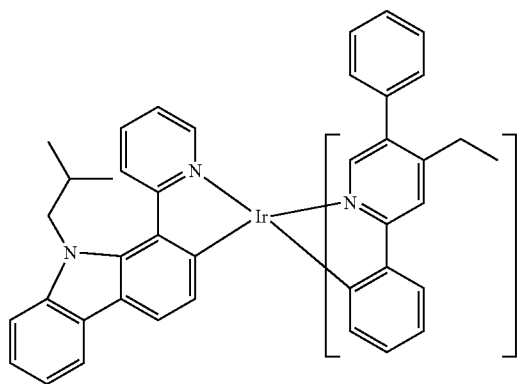
Compound 95
