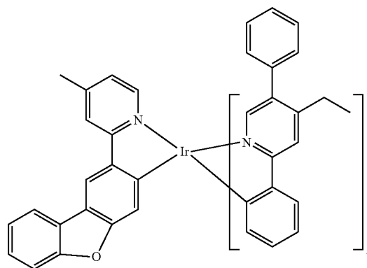
Compound 51
