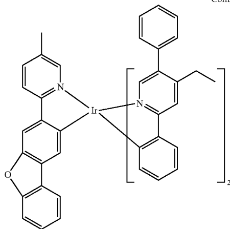
Compound 53
