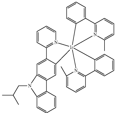
Compound 30
