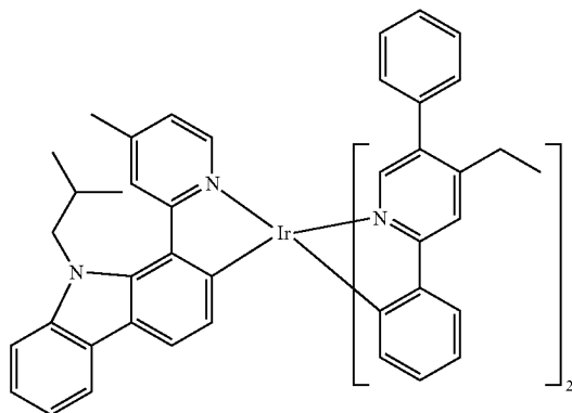
Compound 85
