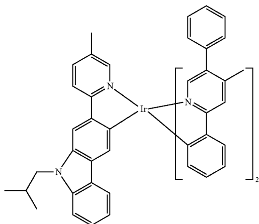
Compound 92
