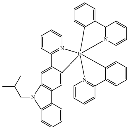
Compound 26
