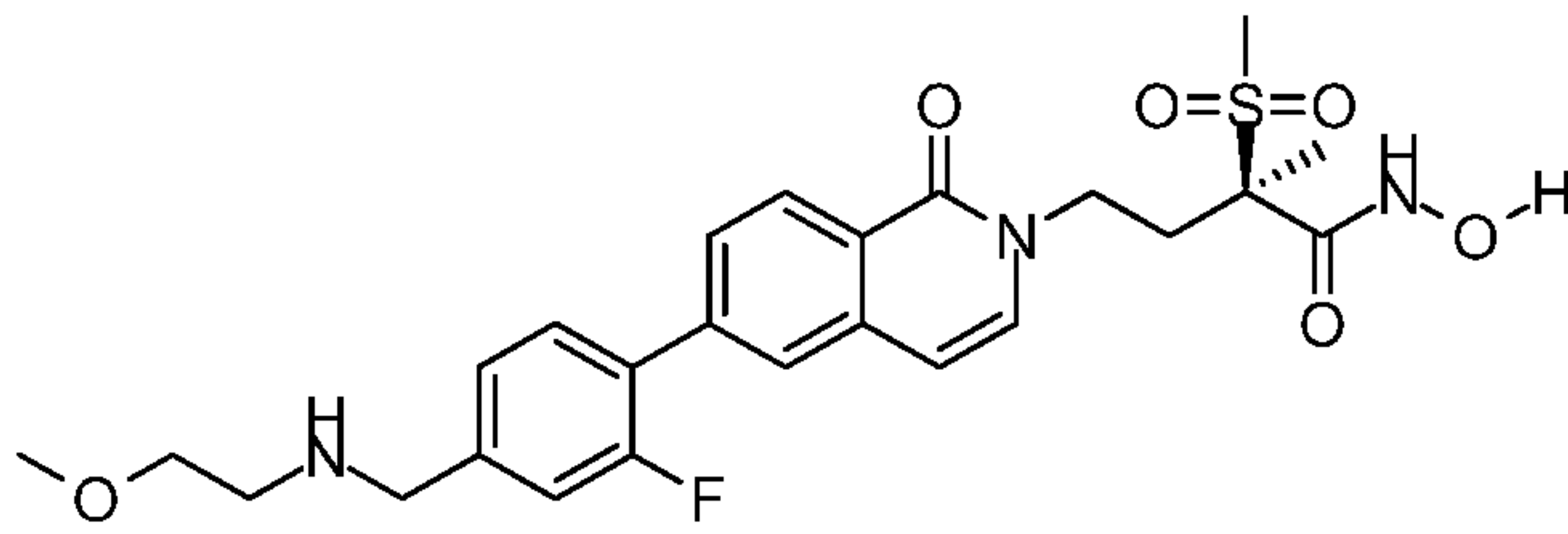
(2R)-4-[6-(2-fluoro-4-[(2-methoxyethyl)amino]methyl)phenyl]-1-oxo-1,2-dihydroisoquinolin-2-yl)-N-hydroxy-2-methanesulfonyl-2-methylbutanamide (Example 67)
