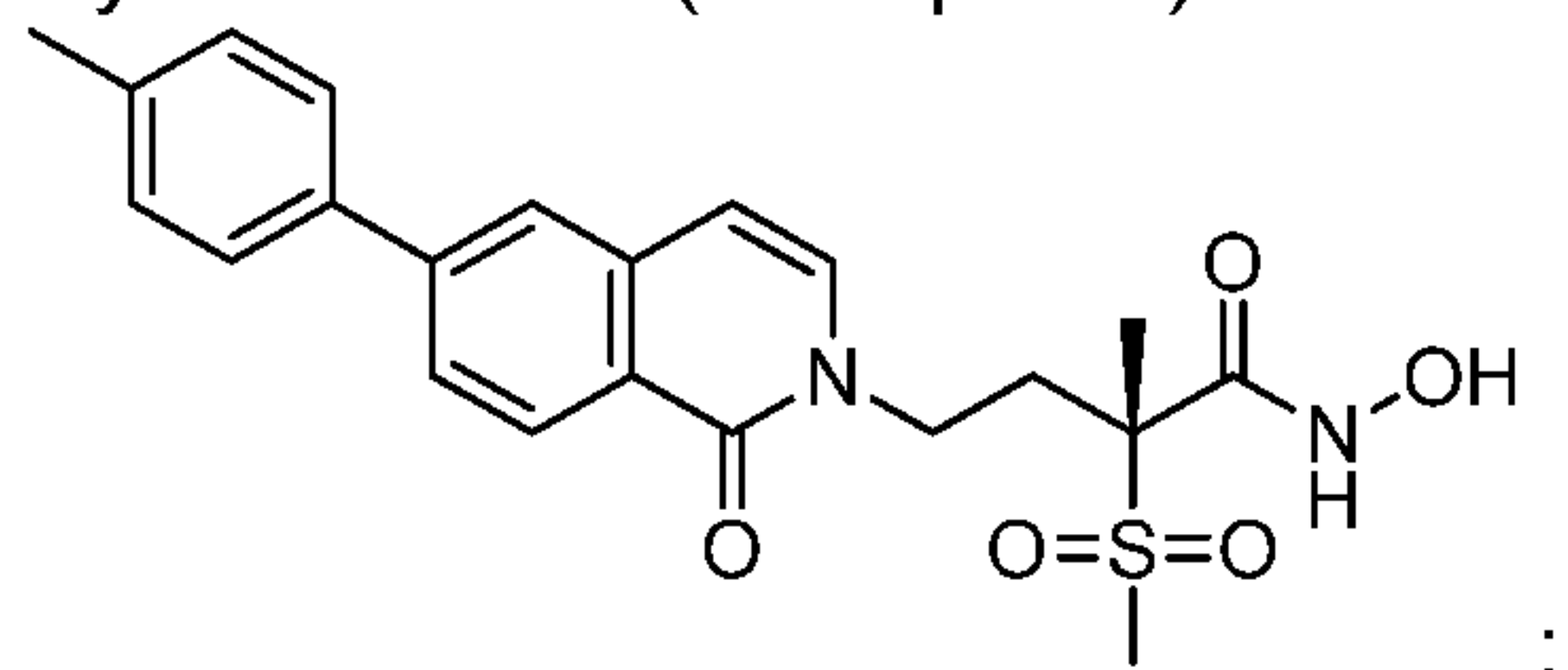
20 (2R)-N-hydroxy-2-methanesulfonyl-4-[6-(4-methoxyphenyl)-1-oxo-1,2-dihydroisoquinolin-2-yl]-2-methylbutanamide (Example 53)
