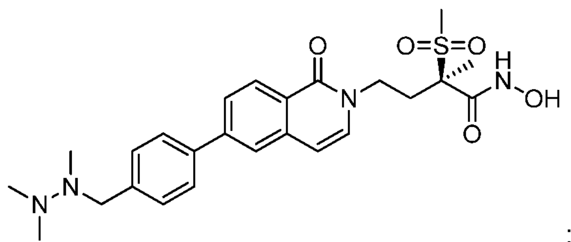
5 (2R)-N-hydroxy-2-methanesulfonyl-2-methyl-4-(1-oxo-6-{4-[(1,2,2-trimethylhydrazin-1-yl)methyl]phenyl}-1,2-dihydroisoquinolin-2-yl)butanamide (Example 77)
