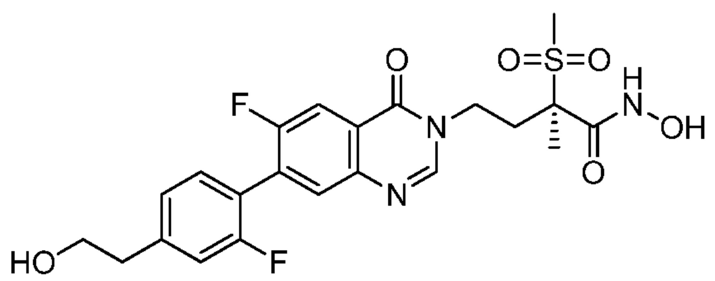
10 (2R)-4-{6-fluoro-7-[4-(2-hydroxyethyl)phenyl]-4-oxo-3,4-dihydroquinazolin-3-yl}-N-hydroxy-2-methanesulfonyl-2-methylbutanamide (Example 28)
