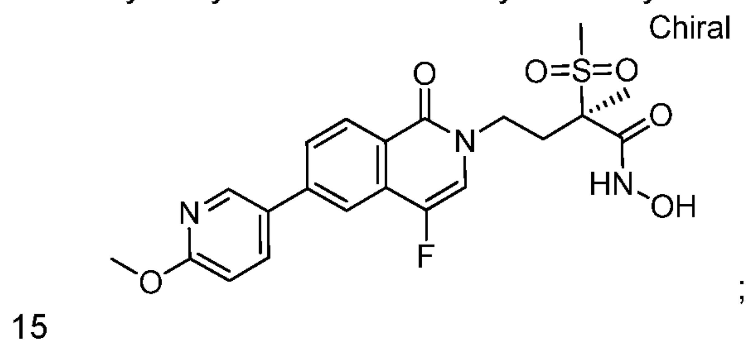
(2R)-4-[4-fluoro-6-(6-methoxypyridin-3-yl)-1-oxo-1,2-dihydroisoquinolin-2-yl]-N-hydroxy-2-methanesulfonyl-2-methylbutanamide (Example 87)
