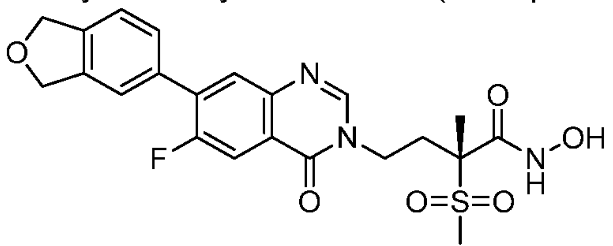
(2R)-4-[7-(1,3-dihydro-2-benzofuran-5-yl)-6-fluoro-4-oxo-3,4-dihydroquinazolin-3-yl]-N-hydroxy-2-methanesulfonyl-2-methylbutanamide (Example 32)
