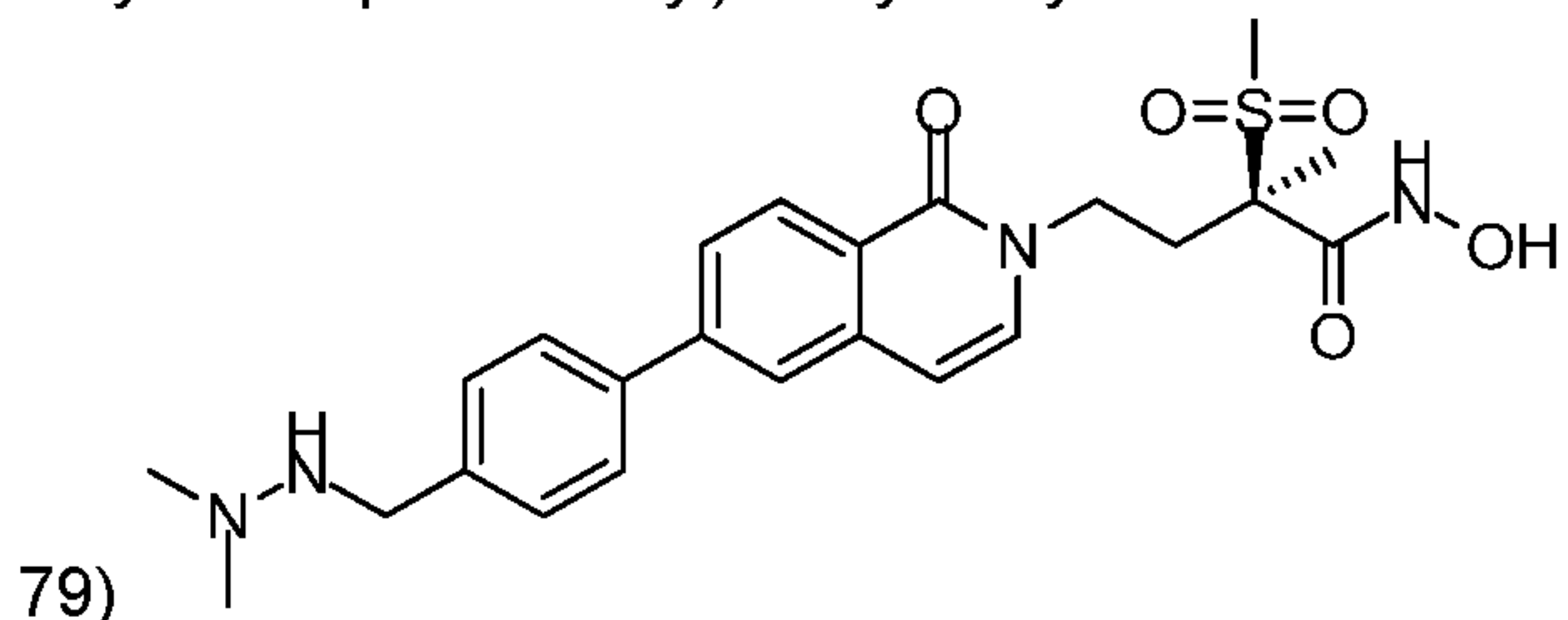
20 (2R)-4-(6-{4-[(2,2-dimethylhydrazin-1-yl)methyl]phenyl}-1-oxo-1,2-dihydroisoquinolin-2-yl)-N-hydroxy-2-methanesulfonyl-2-methylbutanamide (Example 79)
