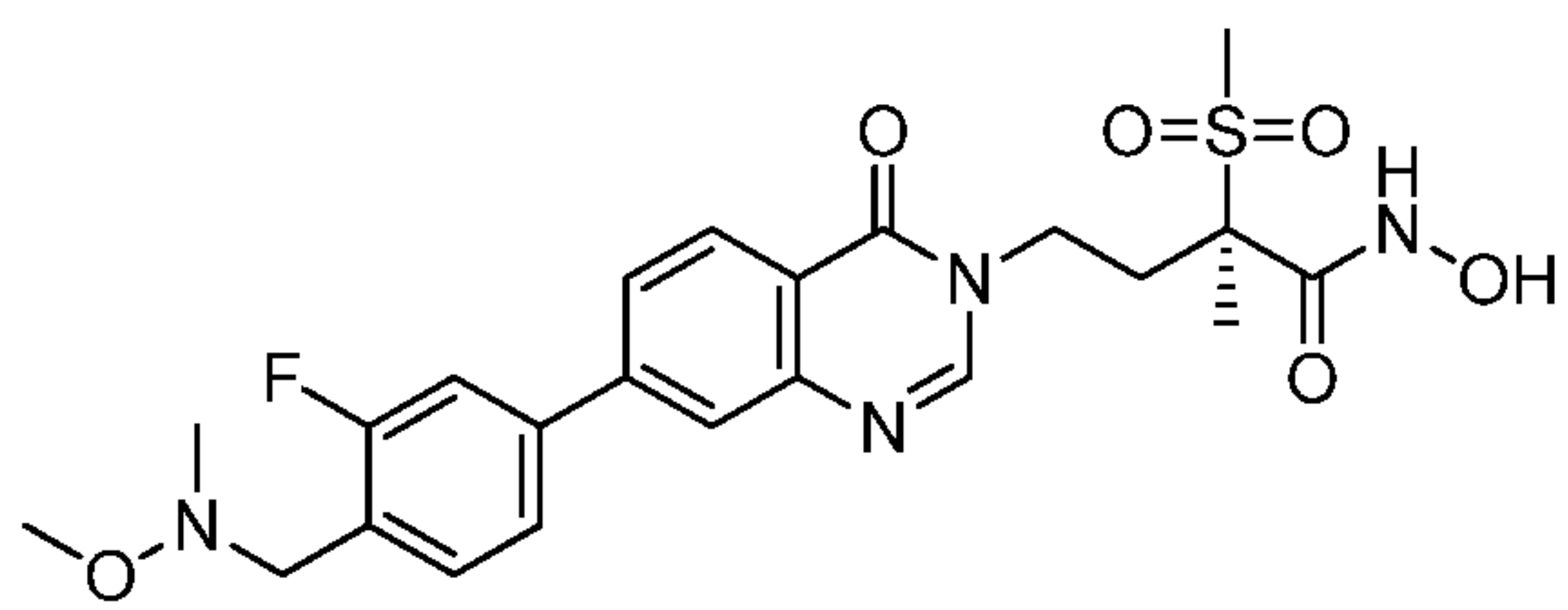
5 (2R)-4-(7-{2-fluoro-4-[(methoxyamino)methyl]phenyl}-4-oxo-3,4-dihydroquinazolin-3-yl)-N-hydroxy-2-methanesulfonyl-2-methylbutanamide (Example 50)
