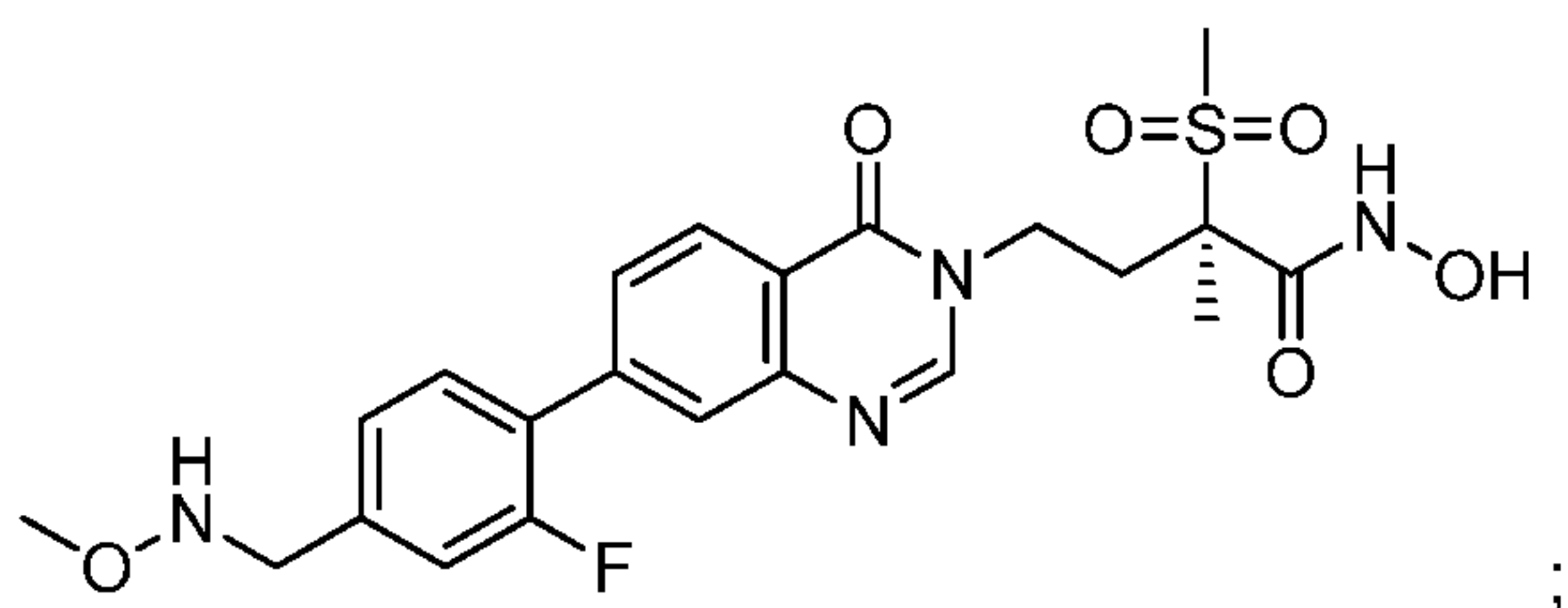
5 (2R)-4-(7-{2-fluoro-4-[(methoxyamino)methyl]phenyl}-4-oxo-3,4-dihydroquinazolin-3-yl)-N-hydroxy-2-methanesulfonyl-2-methylbutanamide (Example 50)
