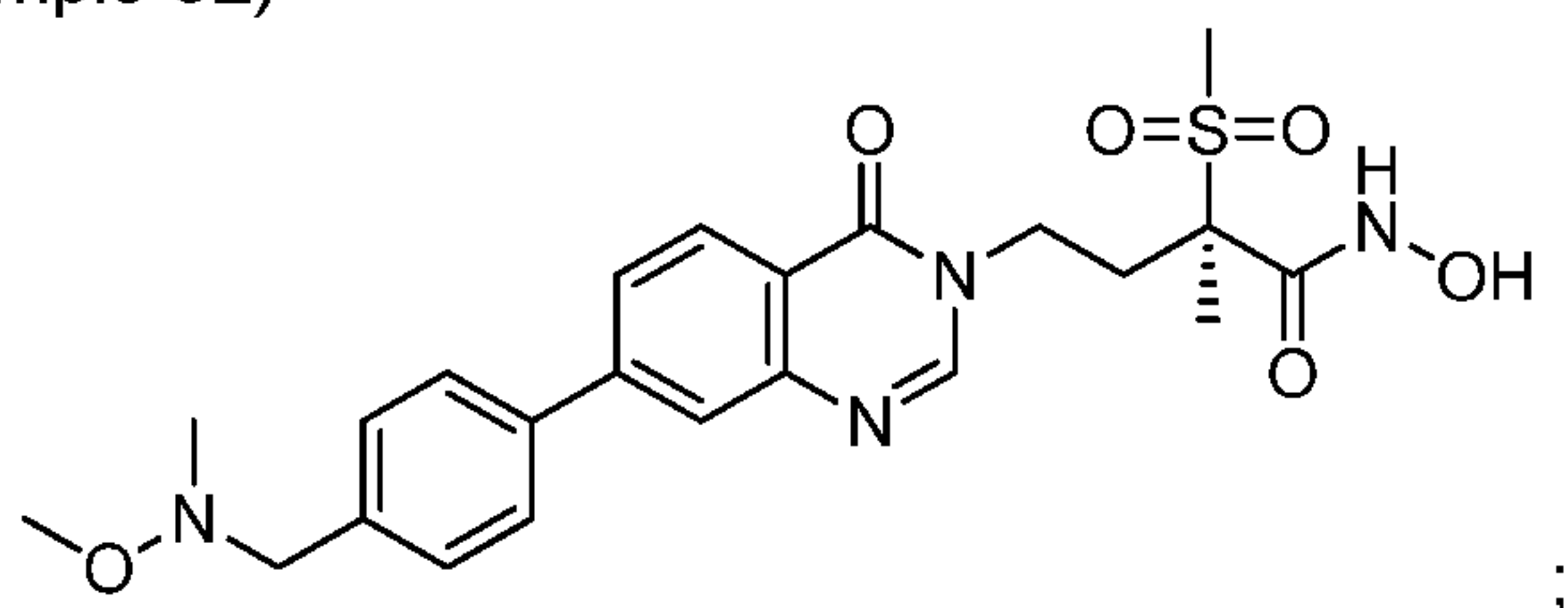
15 (2R)-N-hydroxy-2-methanesulfonyl-4-[7-(4-{[methoxy(methyl)amino]methyl}phenyl)-4-oxo-3,4-dihydroquinazolin-3-yl]-2-methylbutanamide (Example 52)
