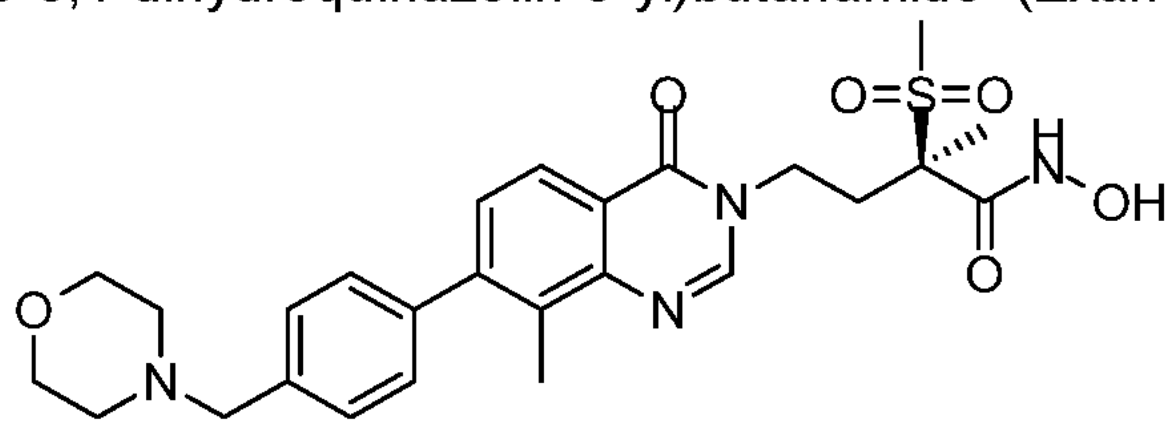
15 (2R)-N-hydroxy-2-methanesulfonyl-2-methyl-4-(8-methyl-7-{4-[(morpholin-4-yl)methyl]phenyl}-4-oxo-3,4-dihydroquinazolin-3-yl)butanamide (Example 29)
