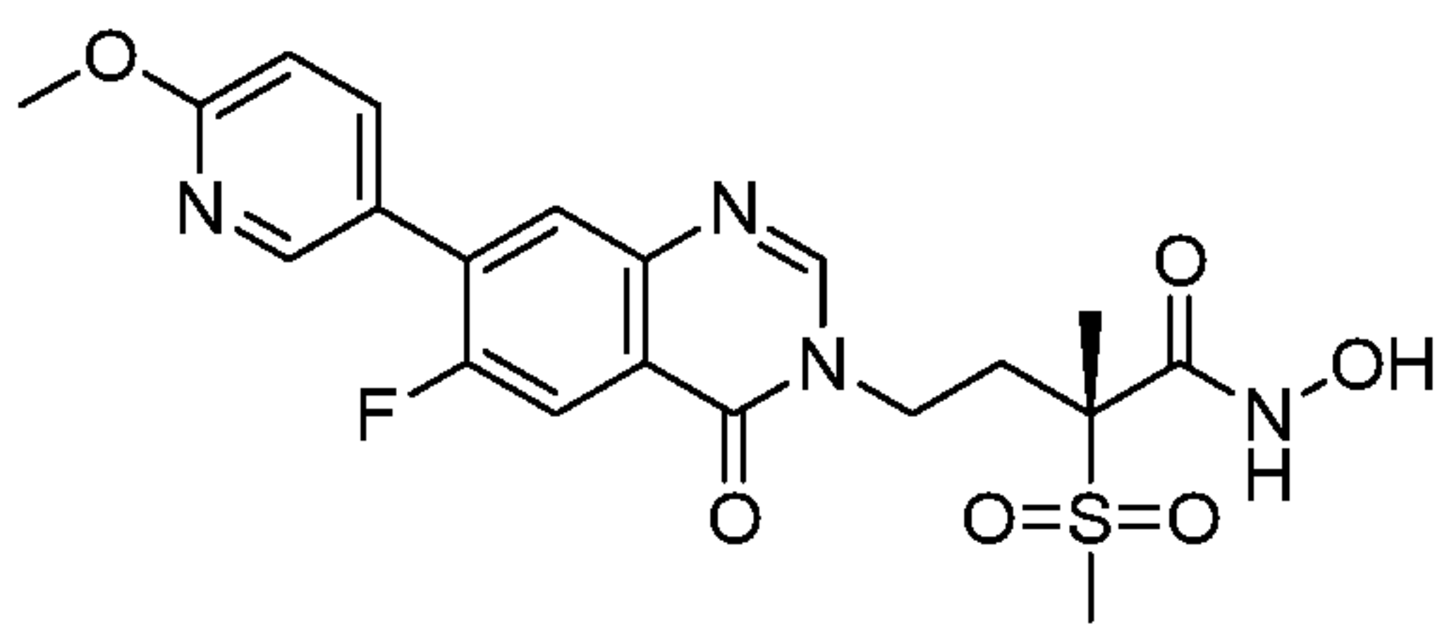
(2R)-4-(6-fluoro-4-oxo-7-phenyl-3,4-dihydroquinazolin-3-yl)-N-hydroxy-2-methanesulfonyl-2-methylbutanamide (Example 31)
