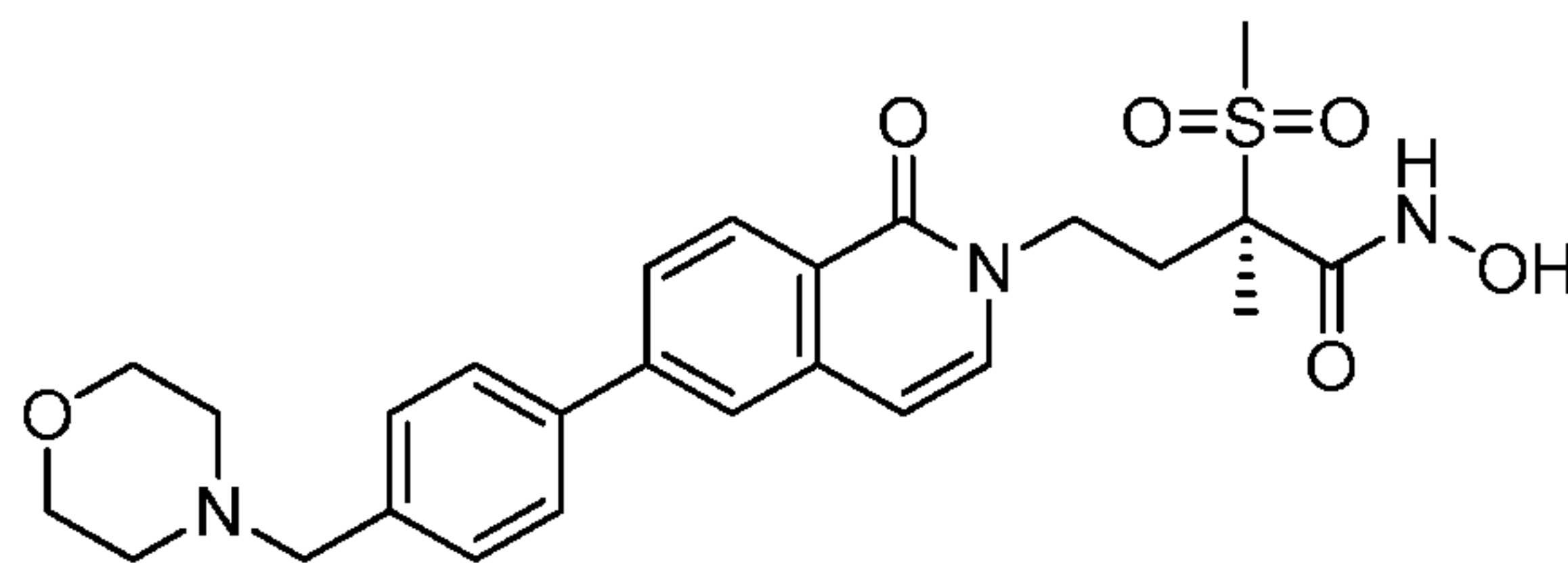
(2R)-4-(6-{4-[(dimethylamino)methyl]-2-fluorophenyl}-1-oxo-1,2-dihydroisoquinolin-2-yl)-N-hydroxy-2-methanesulfonyl-2-methylbutanamide (Example 65)
