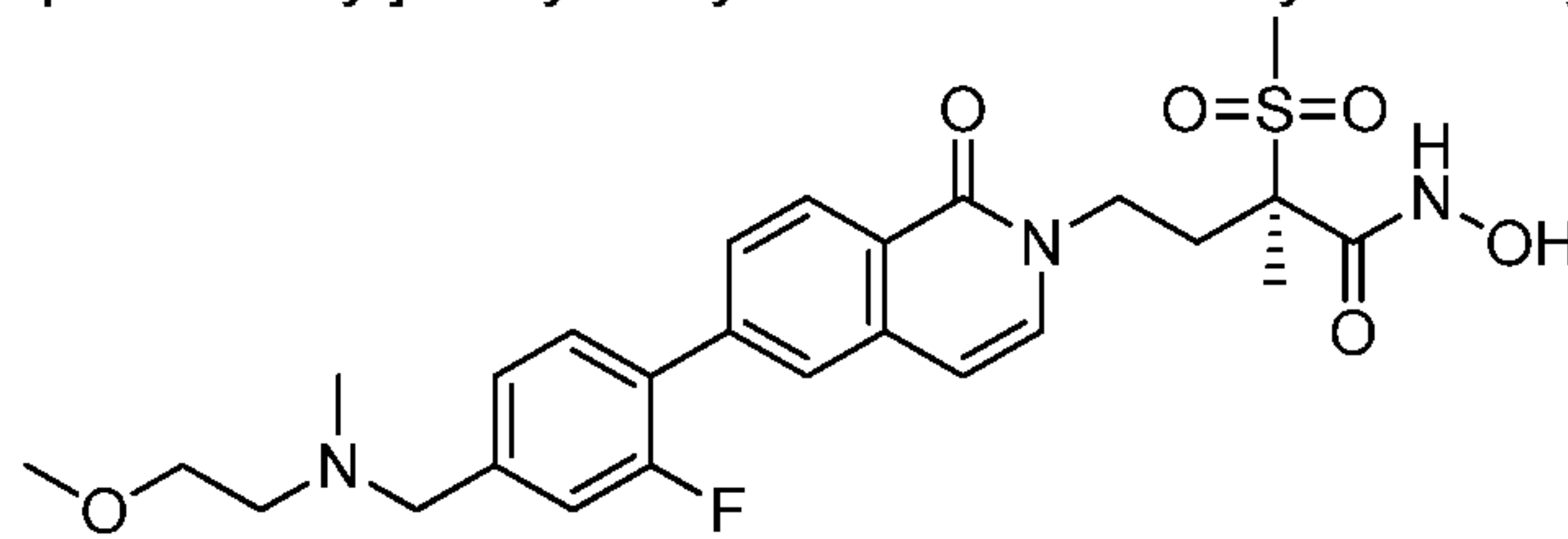
(2R)-4-[6-(2-fluoro-4-[(2-methoxyethyl)(methyl)amino]methyl)phenyl]-1-oxo-1,2-dihydroisoquinolin-2-yl)-N-hydroxy-2-methanesulfonyl-2-methylbutanamide
