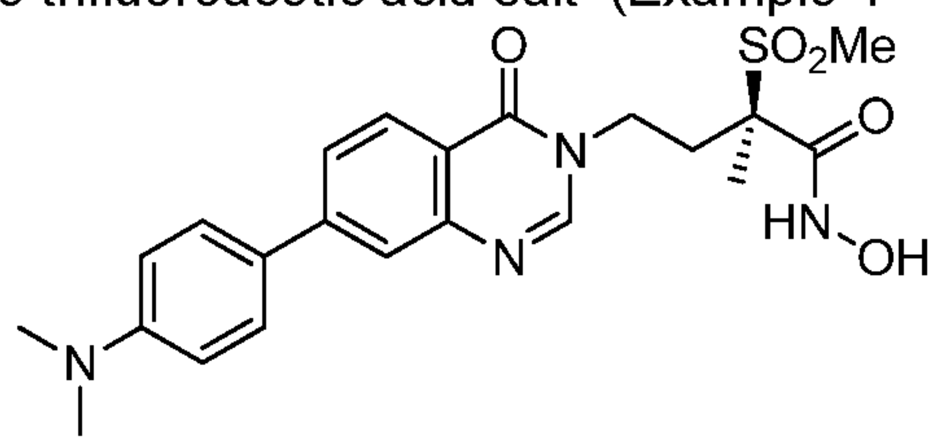
(R)-4-(7-(4-(dimethylamino)phenyl)-4-oxoquinazolin-3(4H)-yl)-N-hydroxy-2-methyl-2-(methylsulfonyl)butanamide trifluoroacetic acid salt (Example 4
