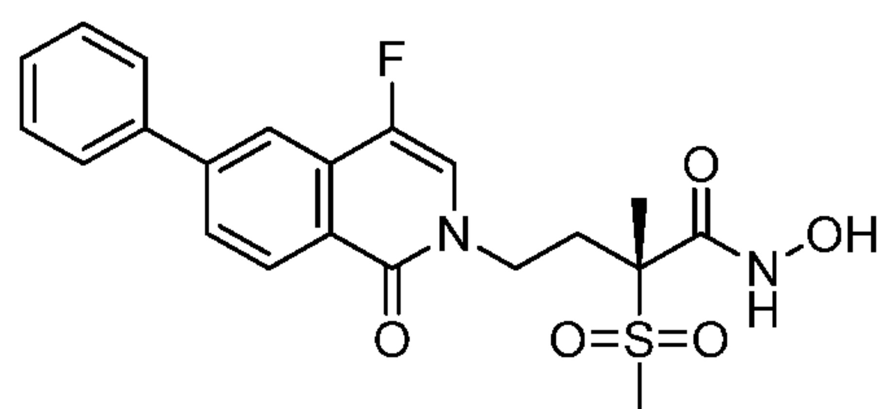
(2R)-4-(6-{4-[(dimethylamino)methyl]phenyl}-4-fluoro-1-oxo-1,2-dihydroisoquinolin-2-yl)-N-hydroxy-2-methanesulfonyl-2-methylbutanamide (Example 85)
