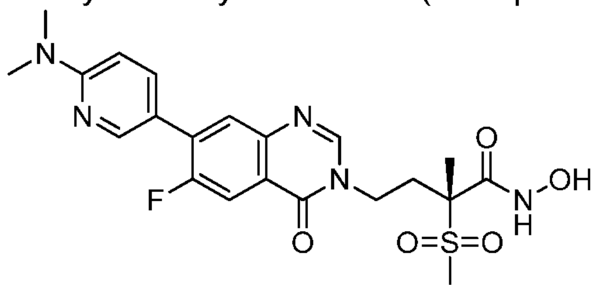
(2R)-4-{7-[6-(dimethylamino)pyridin-3-yl]-6-fluoro-4-oxo-3,4-dihydroquinazolin-3-yl}-N-hydroxy-2-methanesulfonyl-2-methylbutanamide (Example 33)
