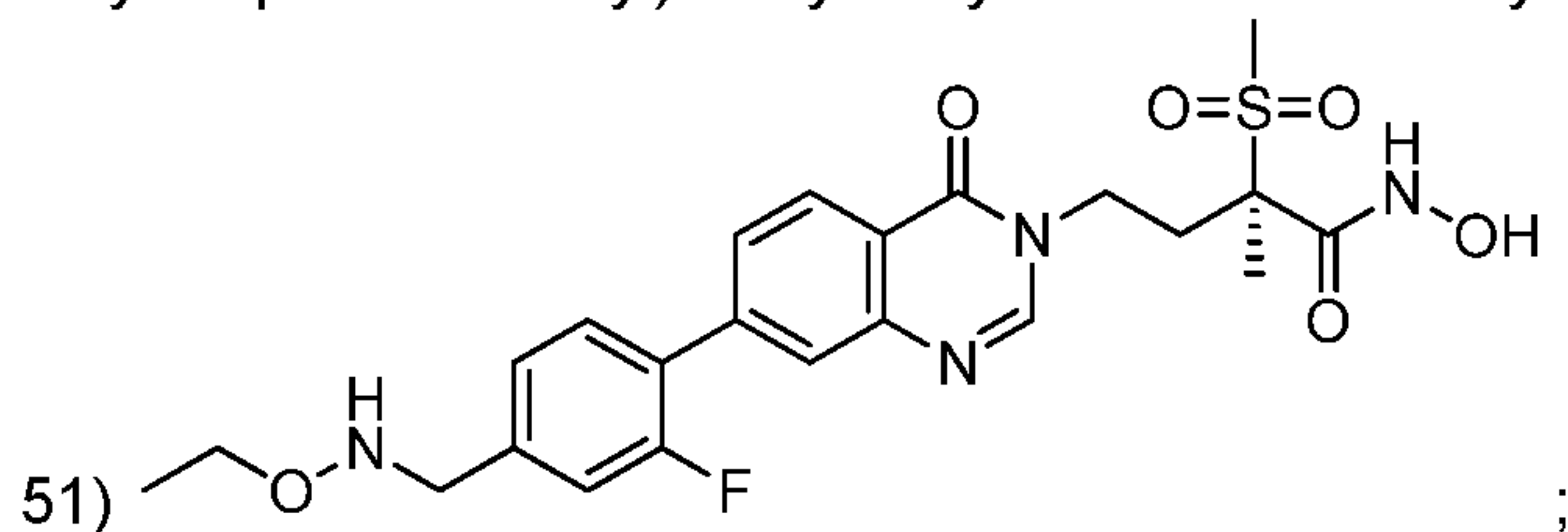
10 (2R)-4-(7-{4-[(ethoxyamino)methyl]-2-fluorophenyl}-4-oxo-3,4-dihydroquinazolin-3-yl)-N-hydroxy-2-methanesulfonyl-2-methylbutanamide (Example 51)
