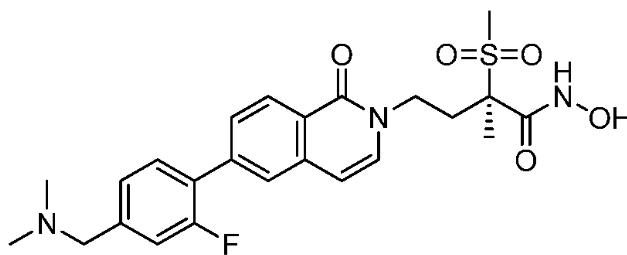
(2R)-4-(6-{4-[(dimethylamino)methyl]-2-fluorophenyl}-1-oxo-1,2-dihydroisoquinolin-2-yl)-N-hydroxy-2-methanesulfonyl-2-methylbutanamide (Example 65)
