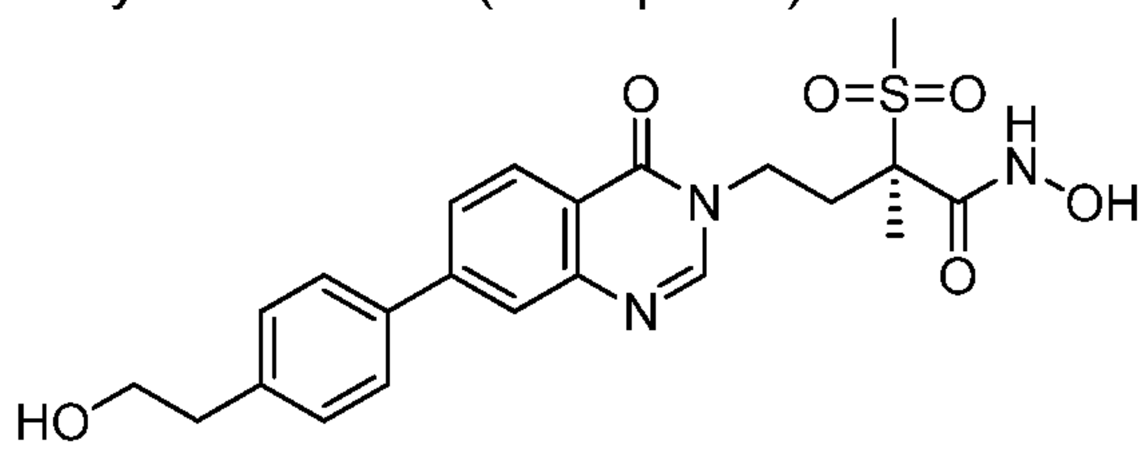
15 (2R)-N-hydroxy-4-{7-[4-(2-hydroxyethyl)phenyl]-4-oxo-3,4-dihydroquinazolin-3-yl}-2-methanesulfonyl-2-methylbutanamide (Example 44)
