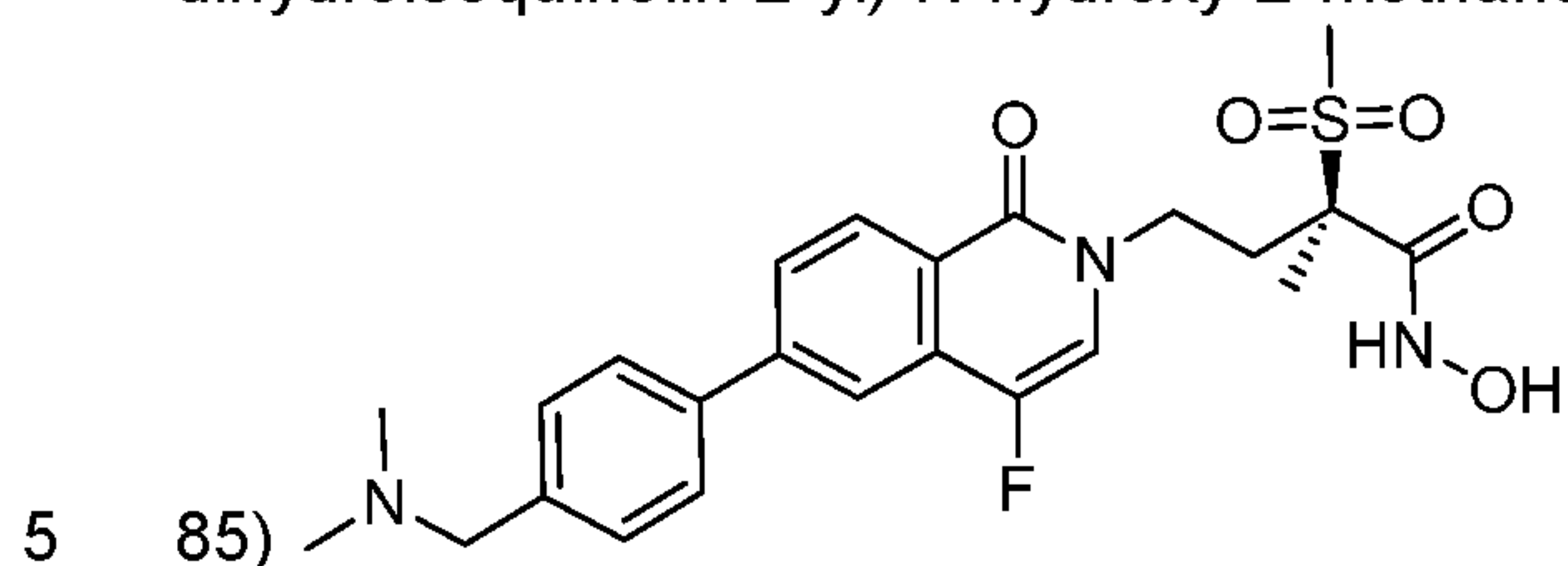
(2R)-4-(6-{4-[(dimethylamino)methyl]phenyl}-4-fluoro-1-oxo-1,2-dihydroisoquinolin-2-yl)-N-hydroxy-2-methanesulfonyl-2-methylbutanamide (Example 85)
