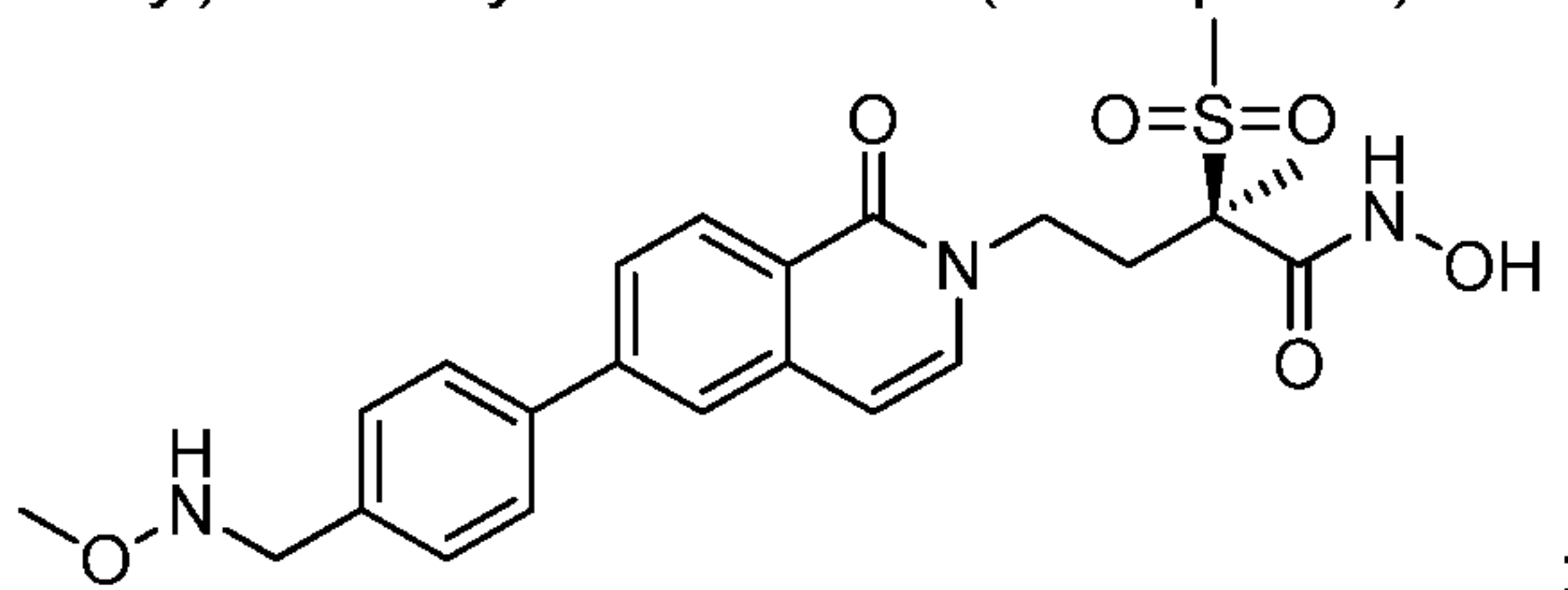
10 (2R)-N-hydroxy-2-methanesulfonyl-4-(6-{4-[(methoxyamino)methyl]phenyl}-1-oxo-1,2-dihydroisoquinolin-2-yl)-2-methylbutanamide (Example 78)
