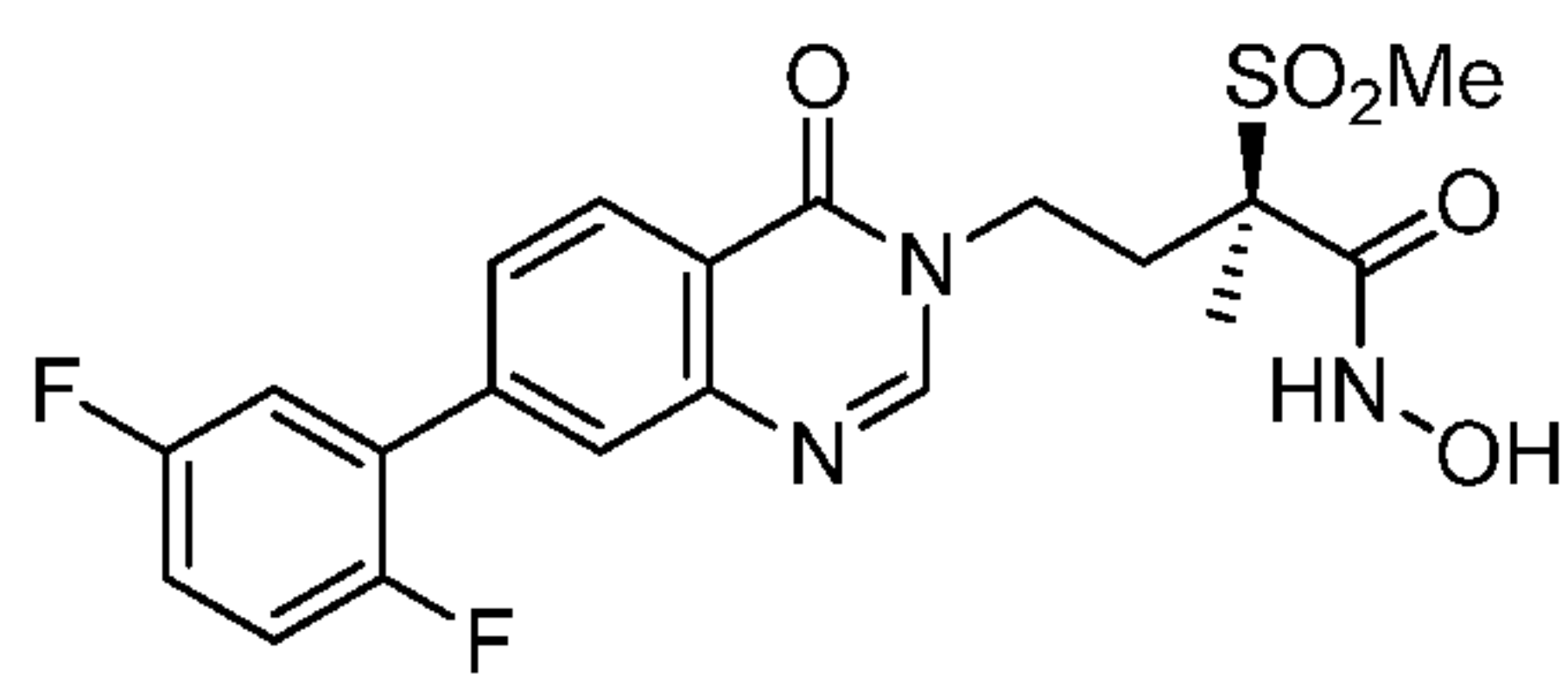
(R)-4-(7-(2,5-difluorophenyl)-4-oxoquinazolin-3(4H)-yl)-N-hydroxy-2-methyl-2-(methylsulfonyl)butanamide (Example 7)
