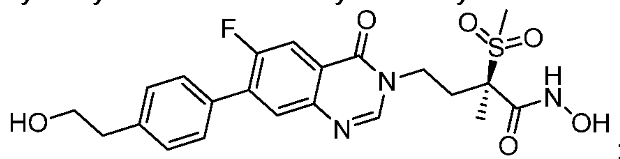
10 (2R)-4-{6-fluoro-7-[4-(2-hydroxyethyl)phenyl]-4-oxo-3,4-dihydroquinazolin-3-yl}-N-hydroxy-2-methanesulfonyl-2-methylbutanamide (Example 28)
