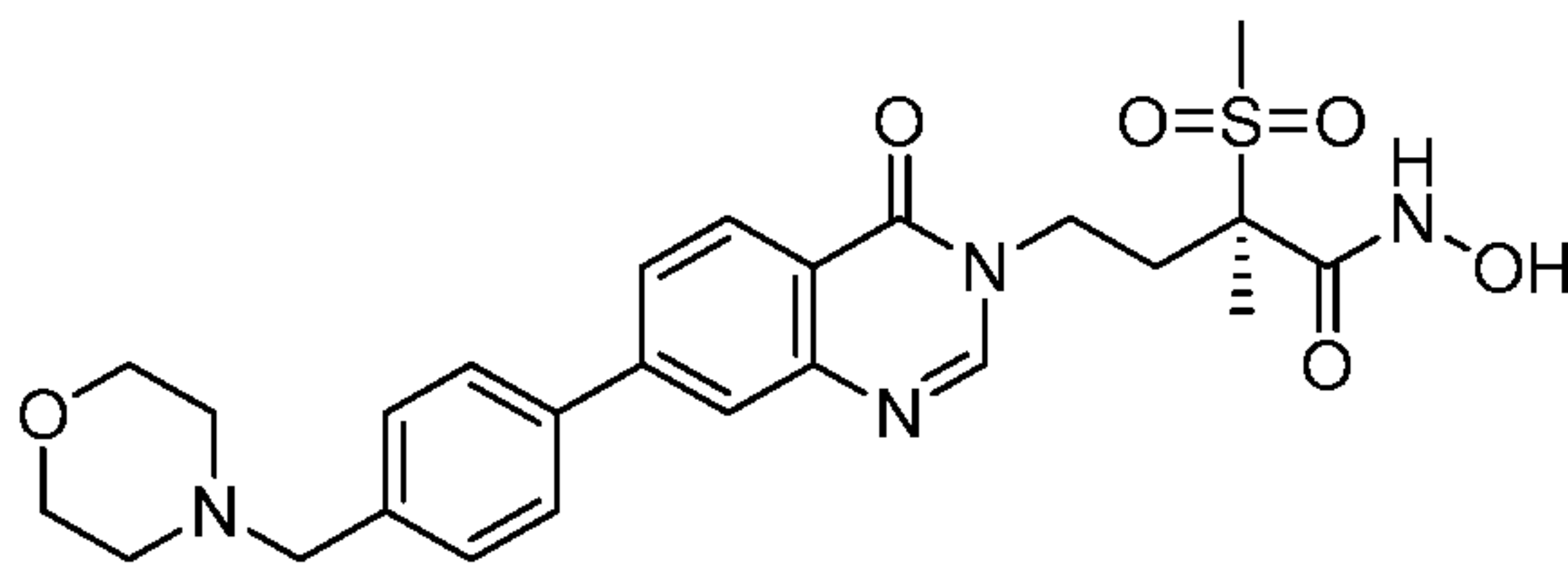
(2R)-N-hydroxy-2-methanesulfonyl-2-methyl-4-(7-{4-[(morpholin-4-yl)methyl]phenyl}-4-oxo-3,4-dihydroquinazolin-3-yl)butanamide (Example 35)
