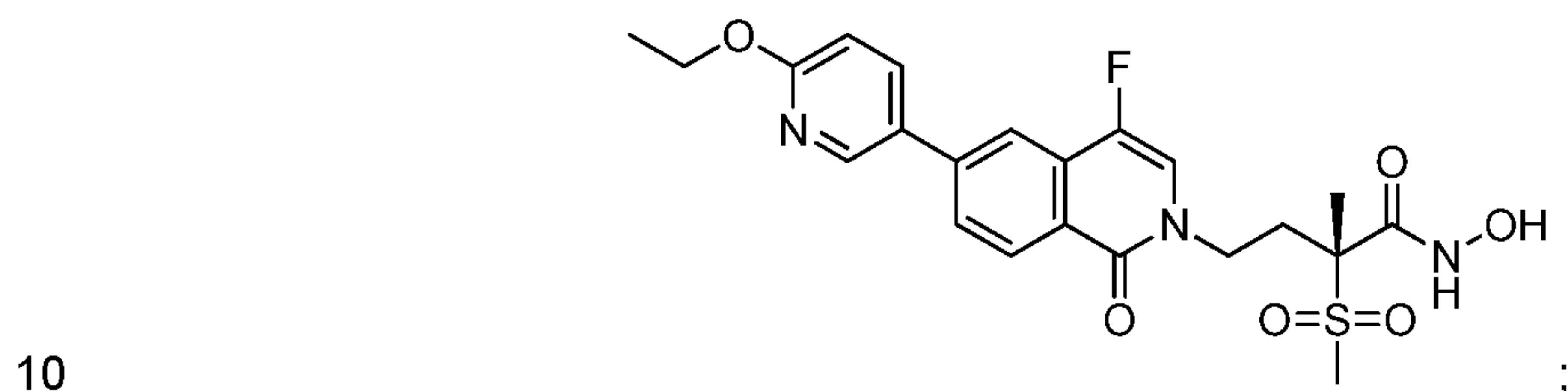
(2R)-4-[4-fluoro-6-(6-methoxypyridin-3-yl)-1-oxo-1,2-dihydroisoquinolin-2-yl]-N-hydroxy-2-methanesulfonyl-2-methylbutanamide (Example 87)
