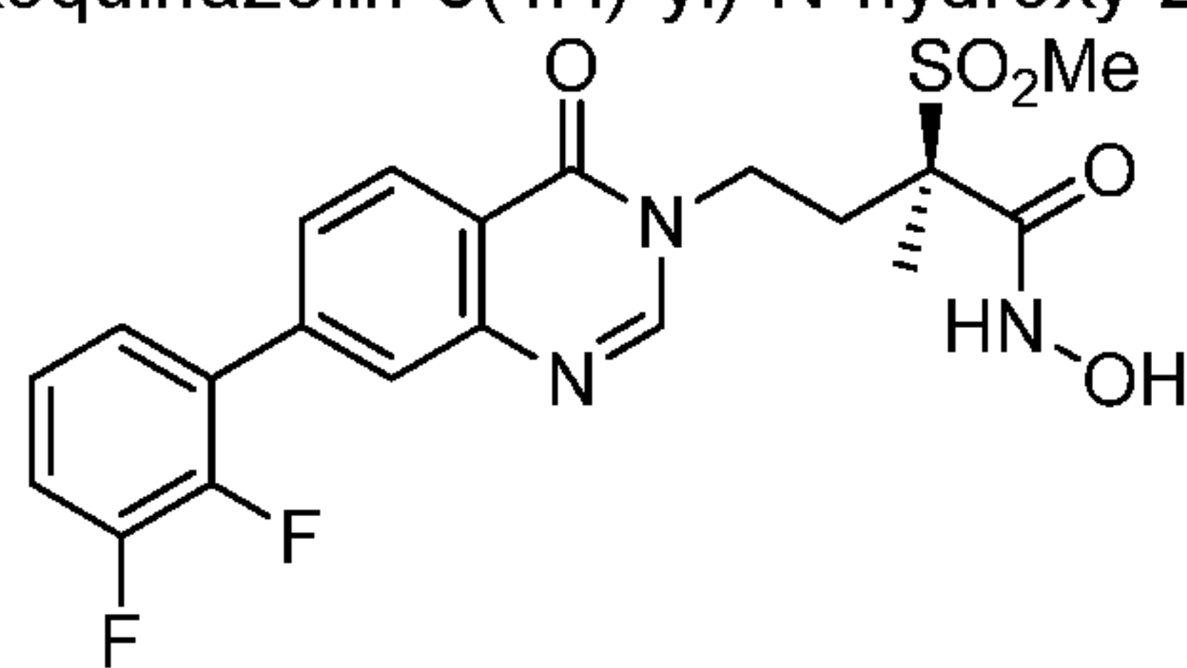
(R)-4-(7-(2,3-difluorophenyl)-4-oxoquinazolin-3(4H)-yl)-N-hydroxy-2-methyl-2-
