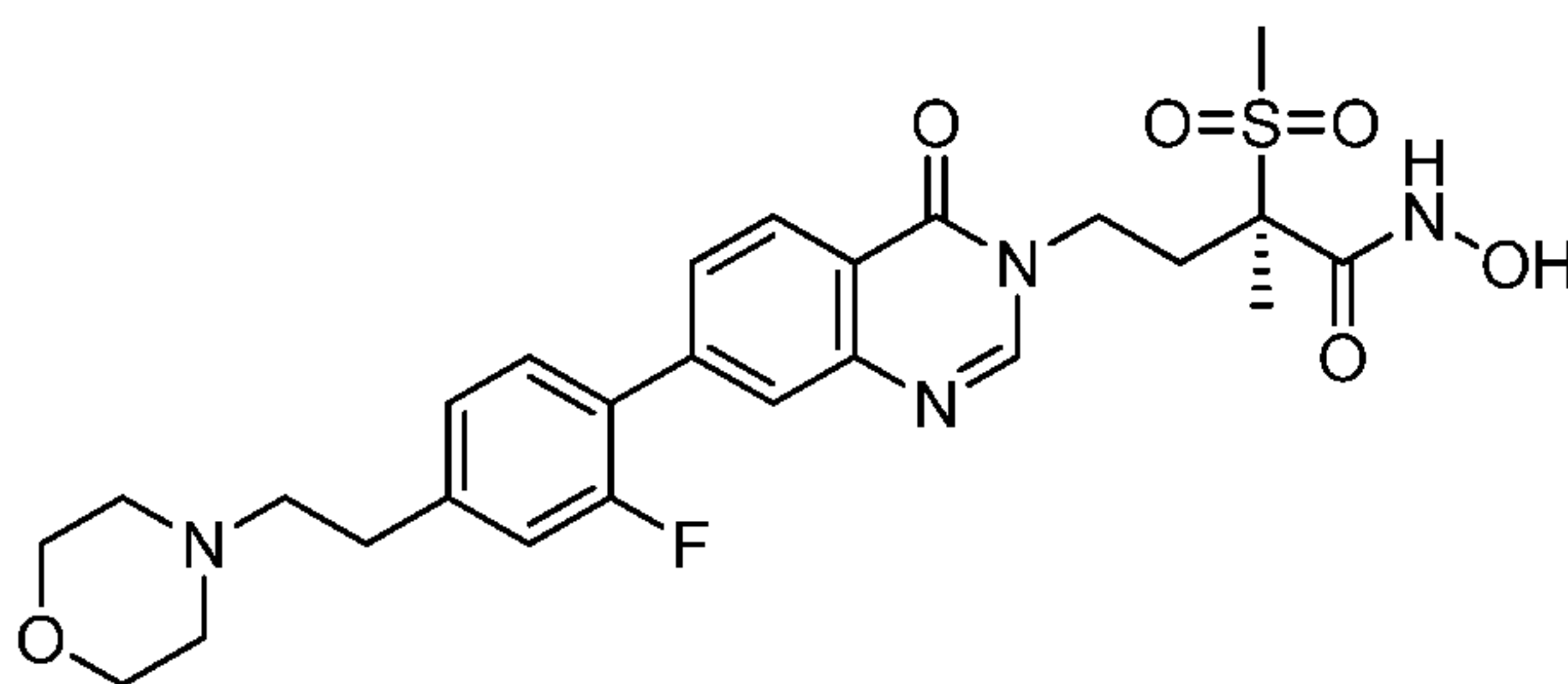
15 (2R)-4-(7-{2-fluoro-4-[2-(morpholin-4-yl)ethyl]phenyl}-4-oxo-3,4-dihydroquinazolin-3-yl)-N-hydroxy-2-methanesulfonyl-2-methylbutanamide (Example 43)
