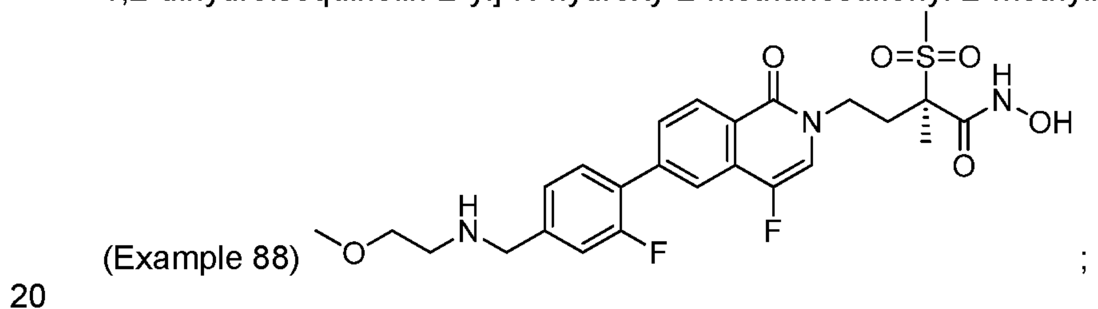
(2R)-4-[4-fluoro-6-(2-fluoro-4-[(2-methoxyethyl)amino]methyl]phenyl)-1-oxo-1,2-dihydroisoquinolin-2-yl]-N-hydroxy-2-methanesulfonyl-2-methylbutanamide
