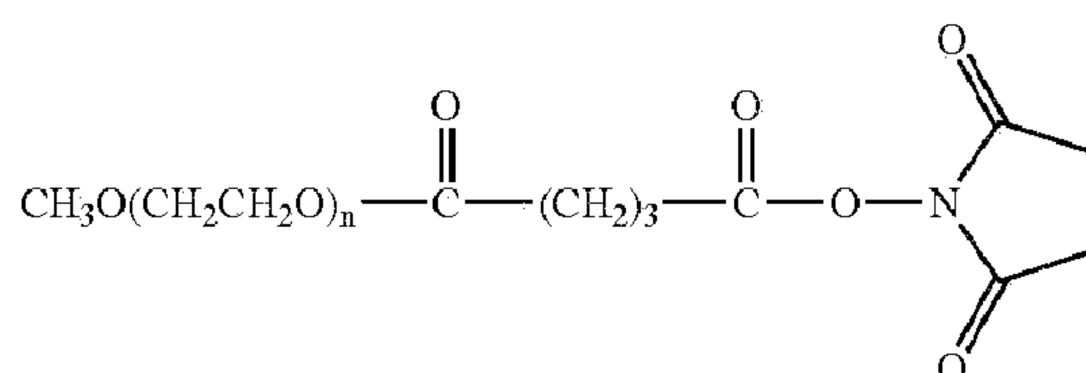
mPEG Succinimidyl glutarate
