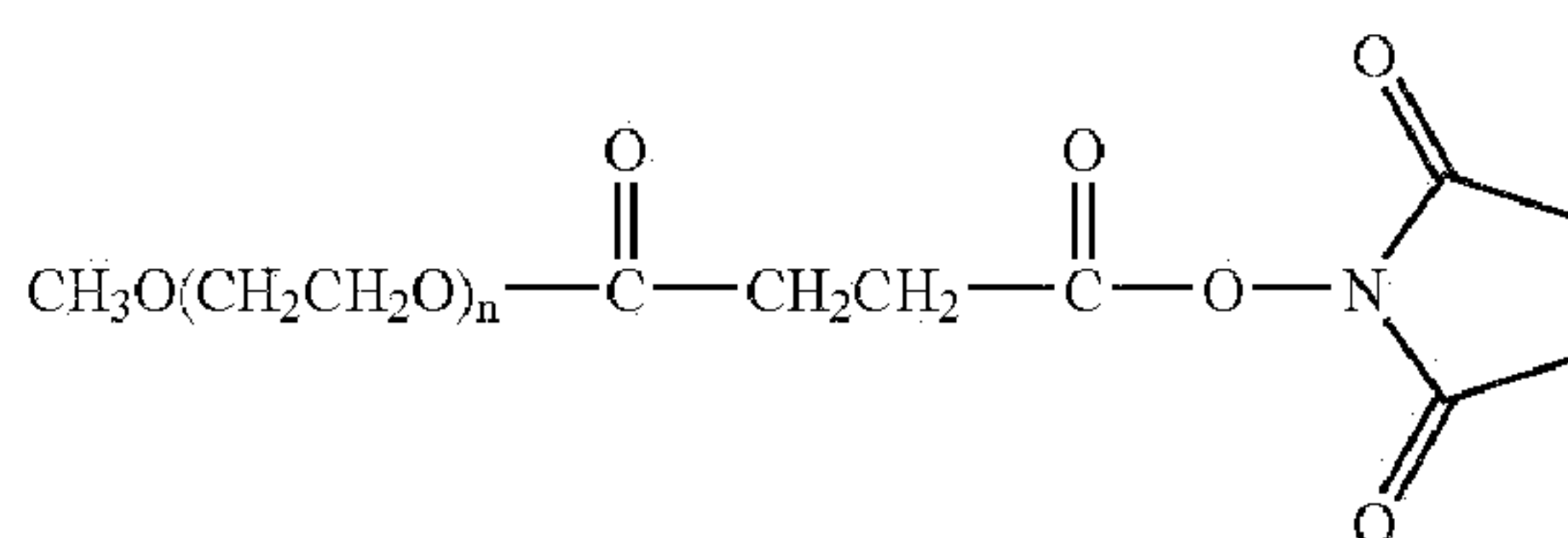
mPEG Succinimidyl succinate
