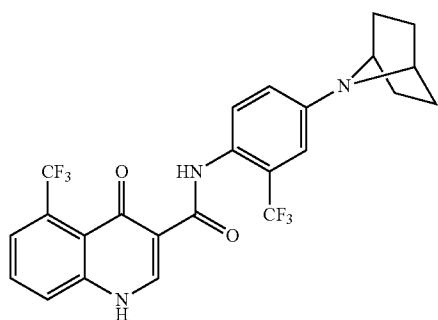
(Form A)
