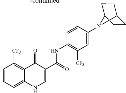
1 (Form B)
