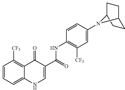
1 (Form A)
