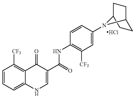
1 (Form B-HCl)
