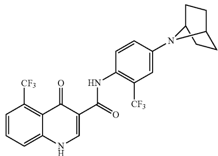
1 (Form B)
