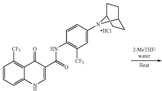
1 (Form A-HCl)
