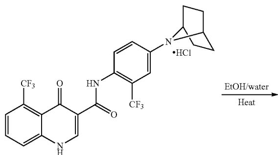
1 (Form A-HCl)
