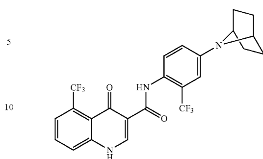
(Form B)
