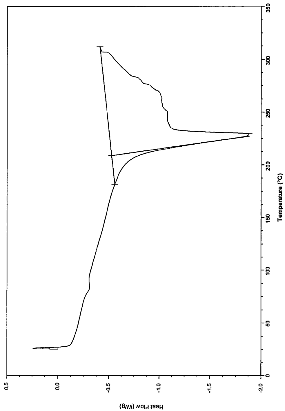
Figure 17 DSC
