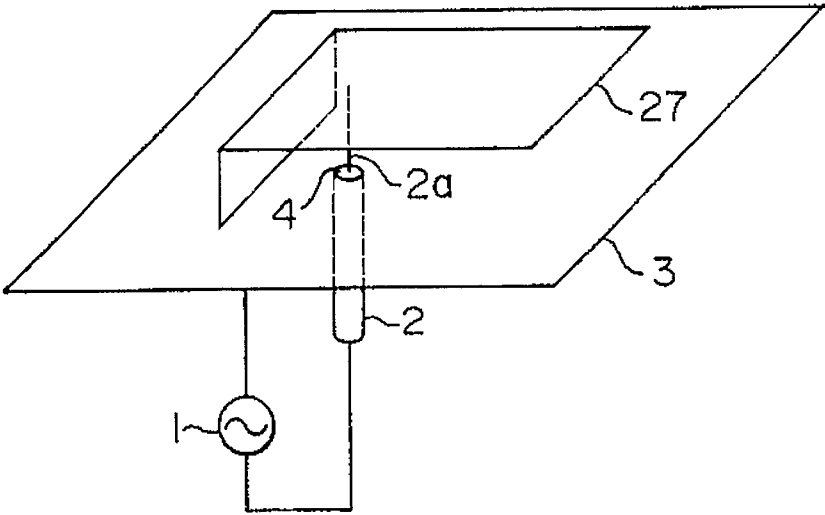
FIG. 22 (PRIOR ART)
