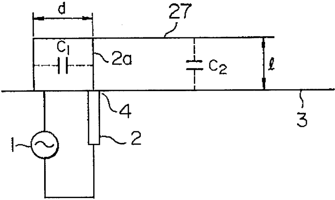
FIG. 23 (PRIOR ART)
