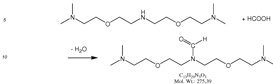
N,N -Bis-[2-(2-dimethylamino-ethoxy)-ethyl]-formamide
