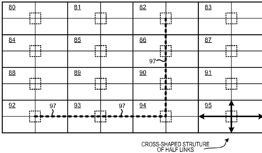
MANHATTAN-PATTERN ISLANDS
