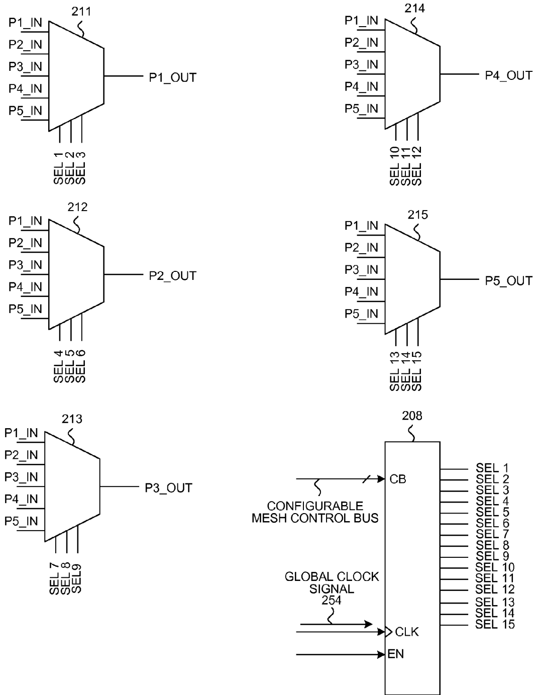
RUN TIME CONFIGURABLE SWITCH CIRCUIT
