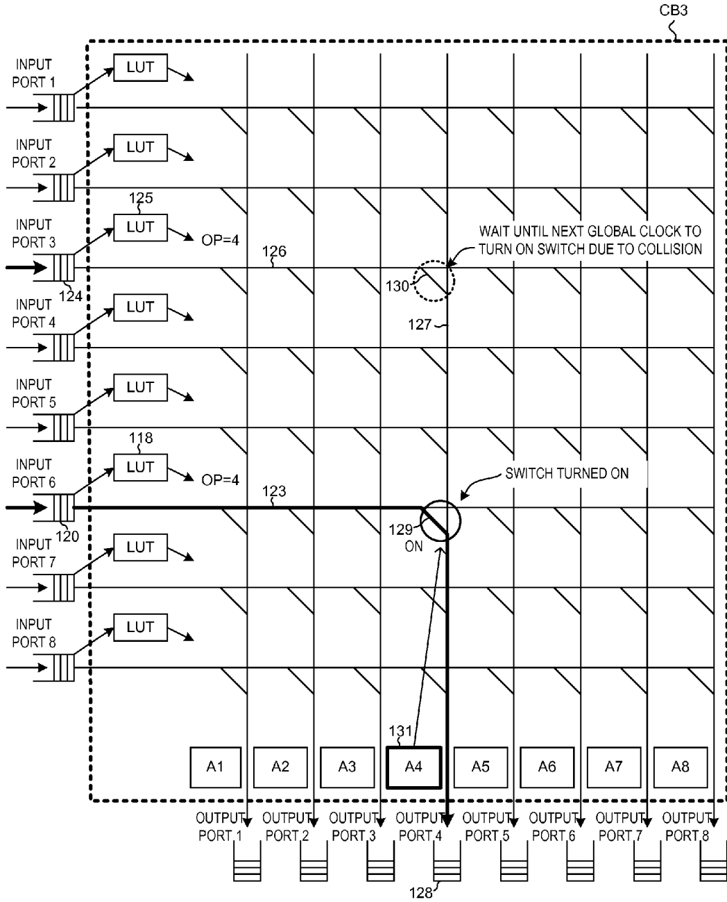
8-WAY CROSSBAR SWITCH FIG. 13
