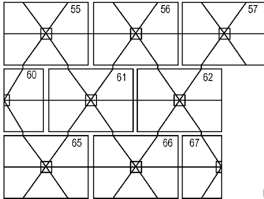
CONFIGURABLE MESH DATA BUS FIG. 26
