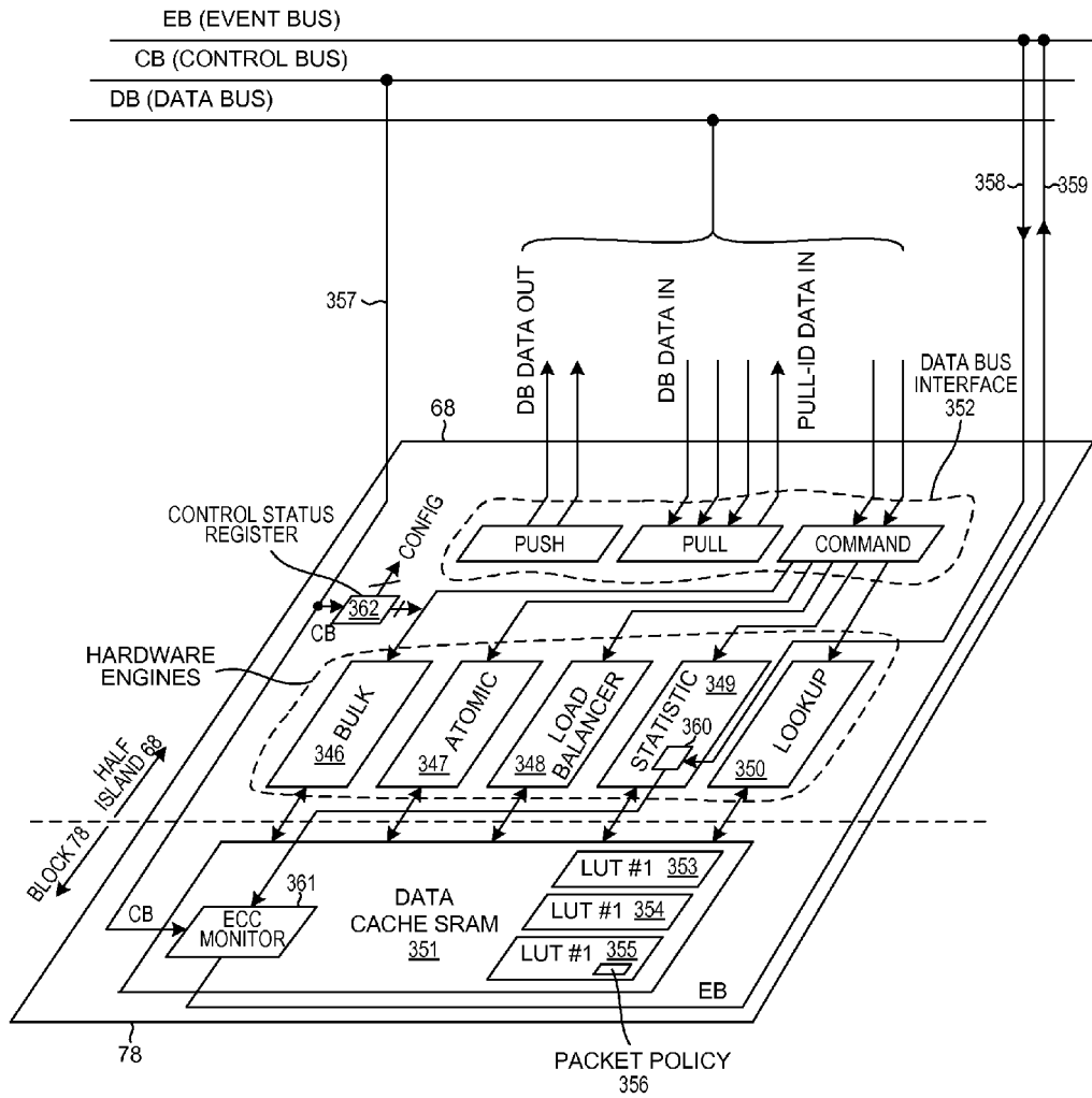
MU ISLAND FIG. 52
