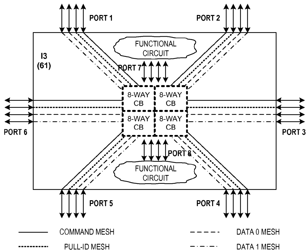
THE FOUR MESHERS OF THE CONFIGURABLE MESH DATA BUS
