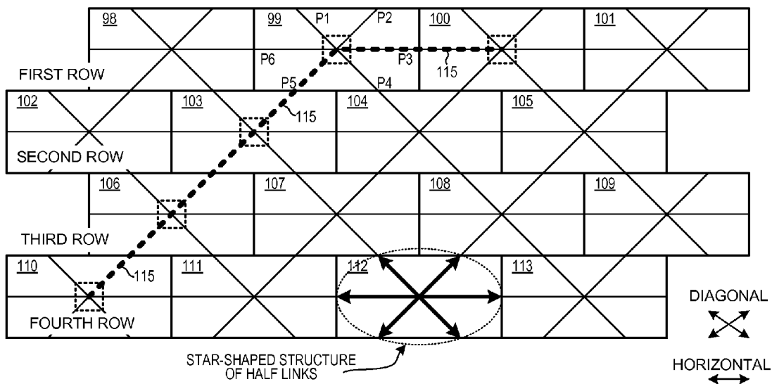
STAGGERED-PATTERN ISLANDS WITH STAR-SHAPED HALF-LINK STRUCTURE
