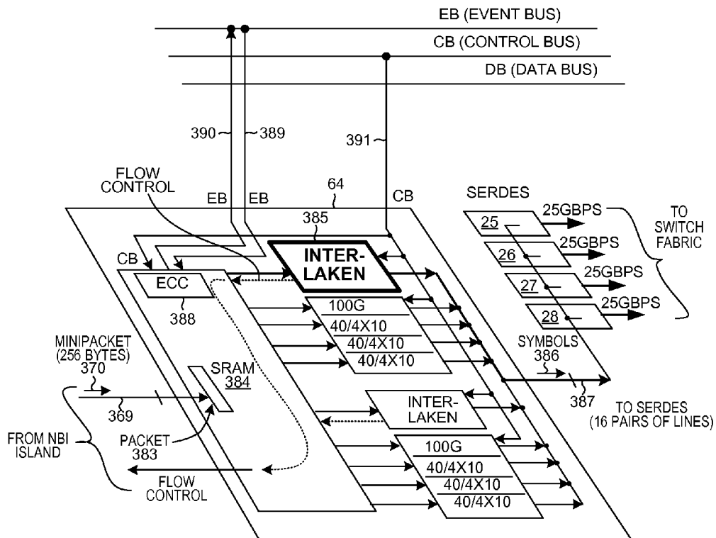
MAC ISLAND (EGRESS)
