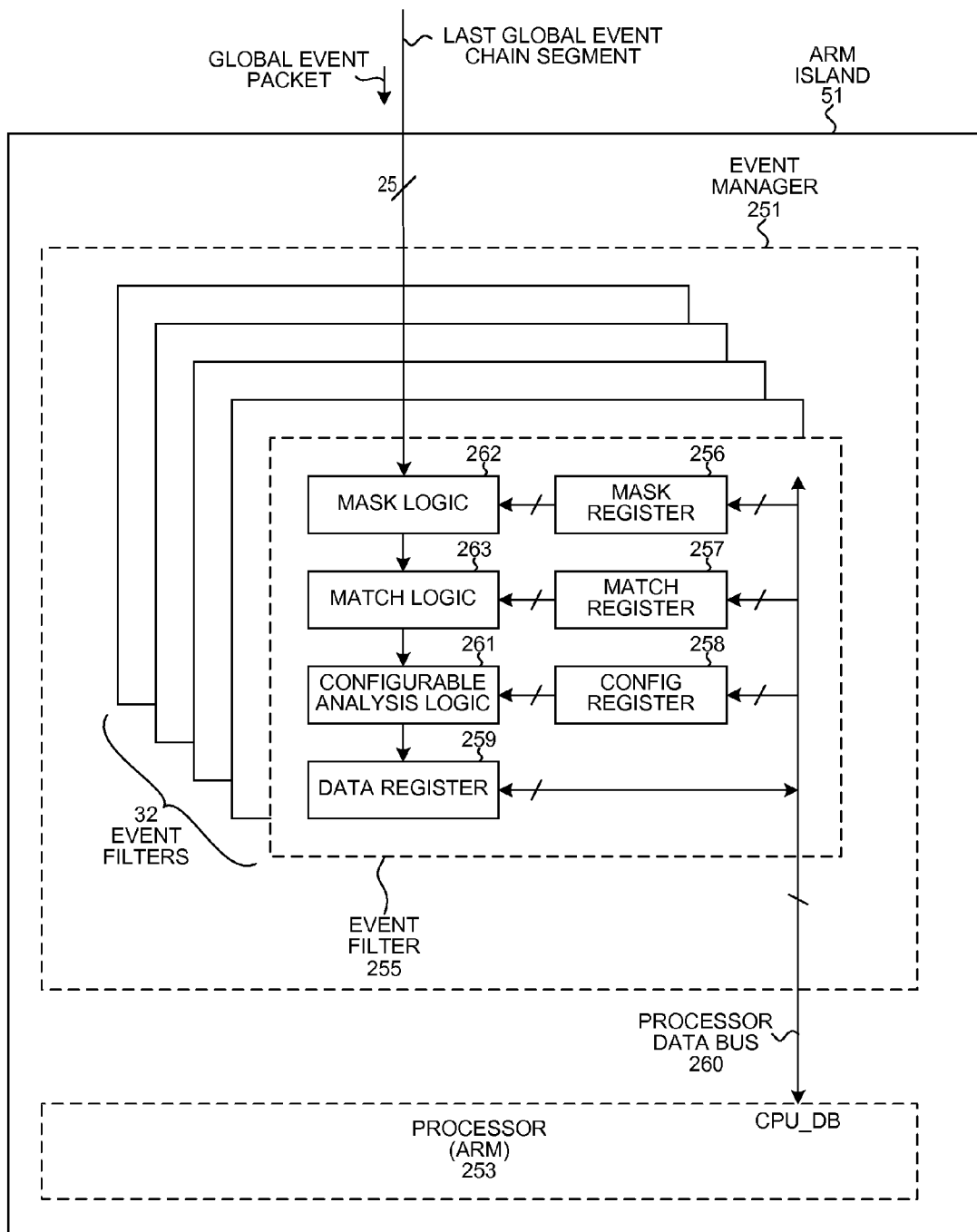
EVENT MANAGER FIG. 42
