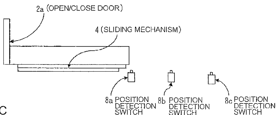
FIG.5B (DOOR FULL-OPEN STATE)
