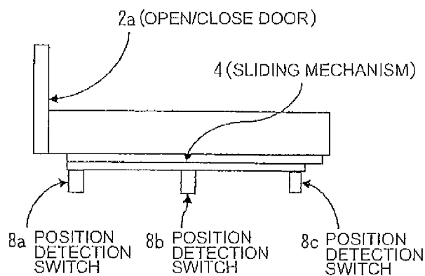
FIG.5A POSITION DETECTION SWITCHES AND MANUAL OPENING/CLOSING OPERATION PREDICTIONS (DOOR FULL-CLOSED STATE)
