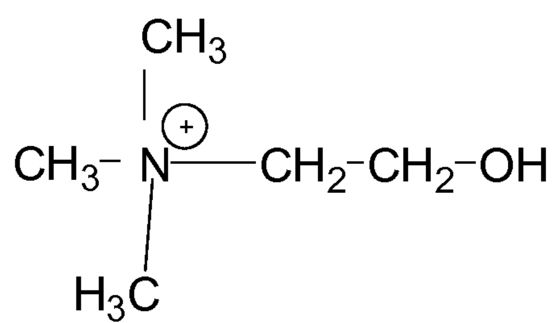
Choline,
