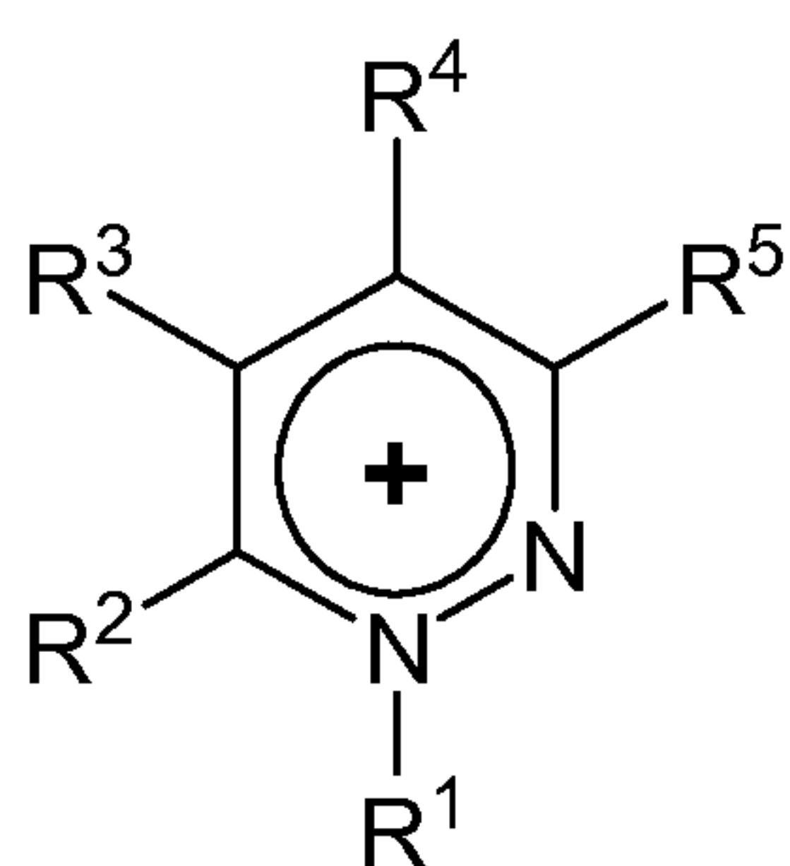
10 Pyridazinium,
