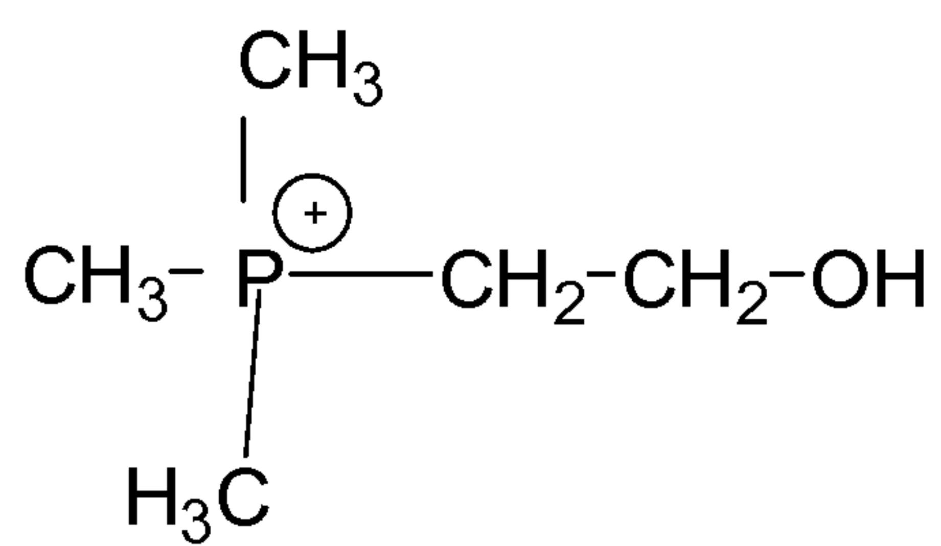
Phosphonium Choline,
