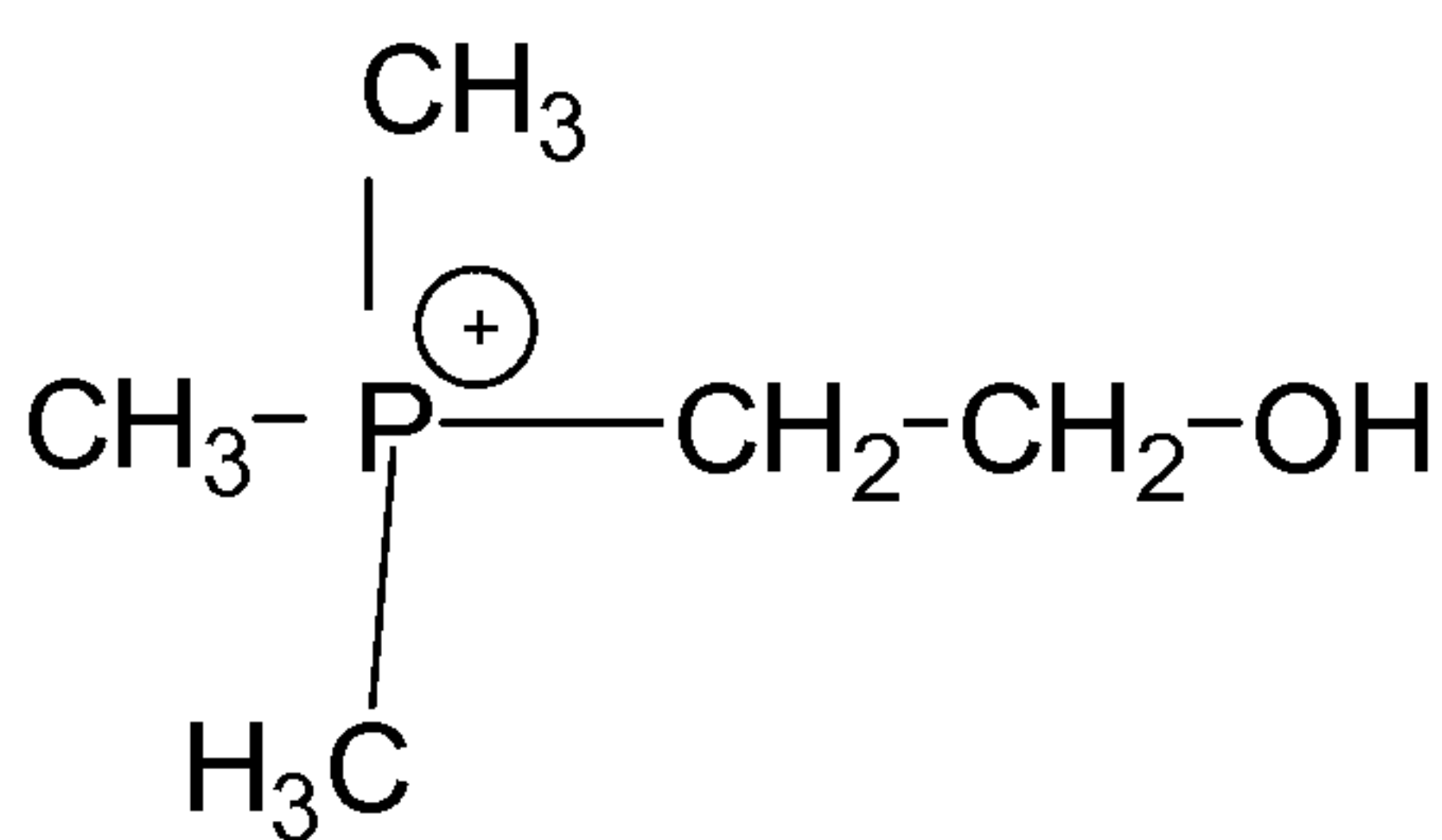
Phosphonium Choline,
