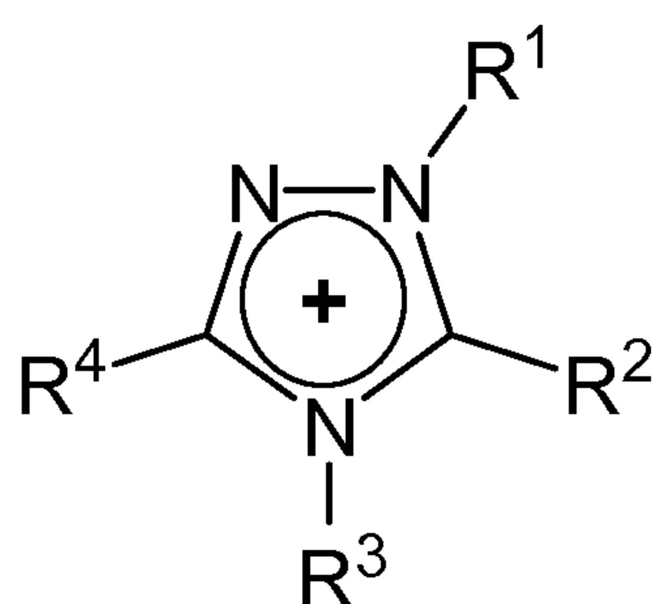
Triazolium,
