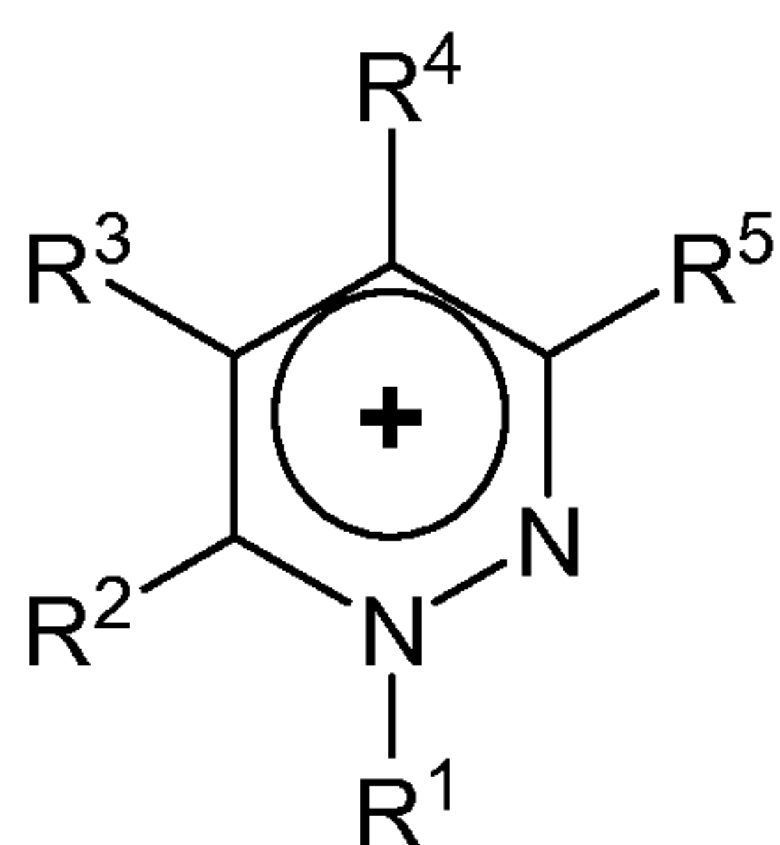
Pyridazinium,
