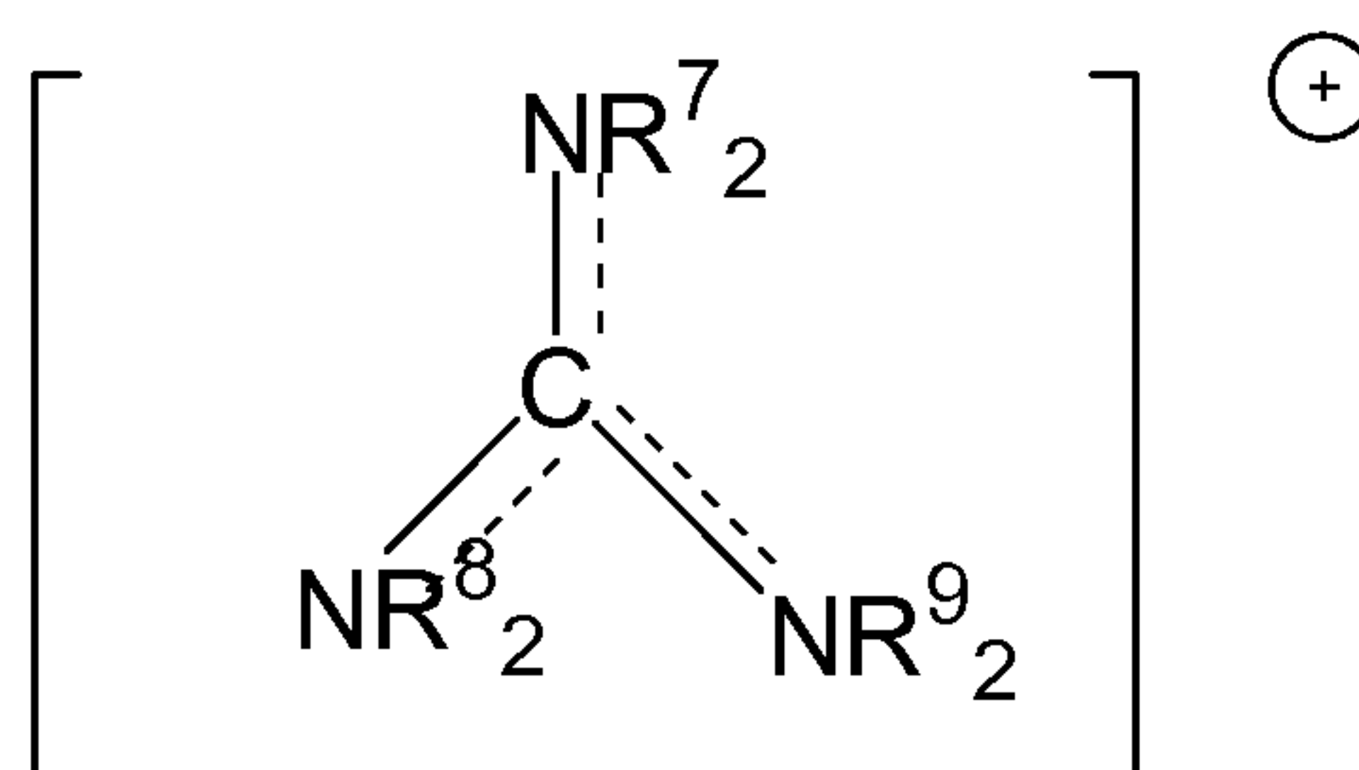
Guanidinium,
