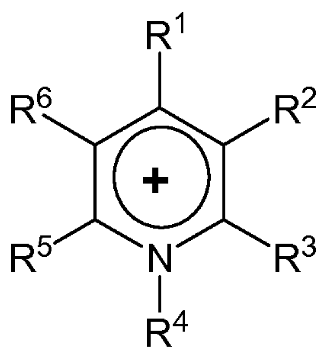
Pyridinium
