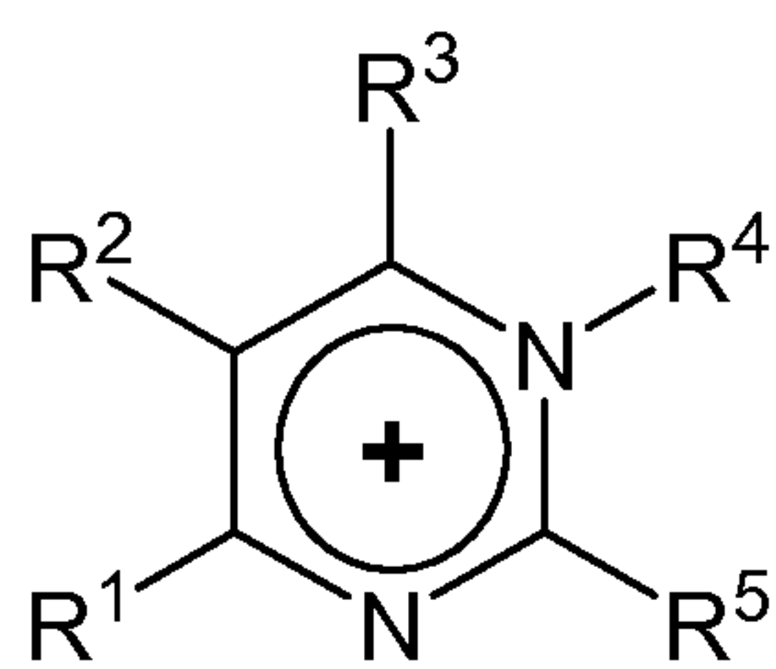
Pyrimidinium,
