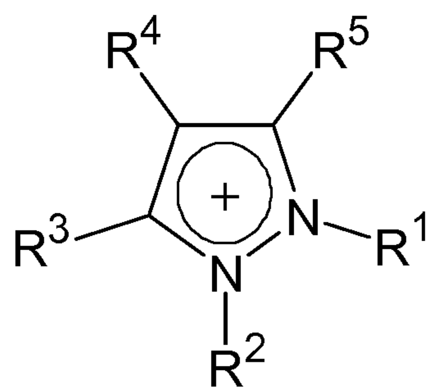
Pyrazolium,
