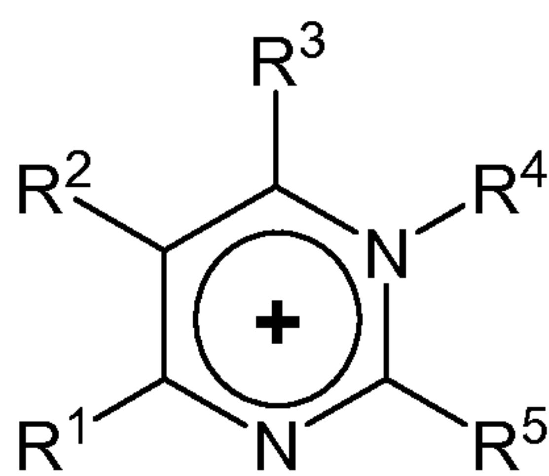
15 Pyrimidinium,
