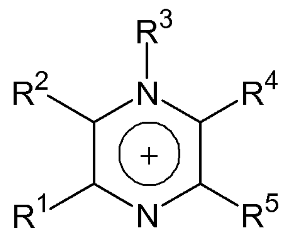
Pyrazinium,
