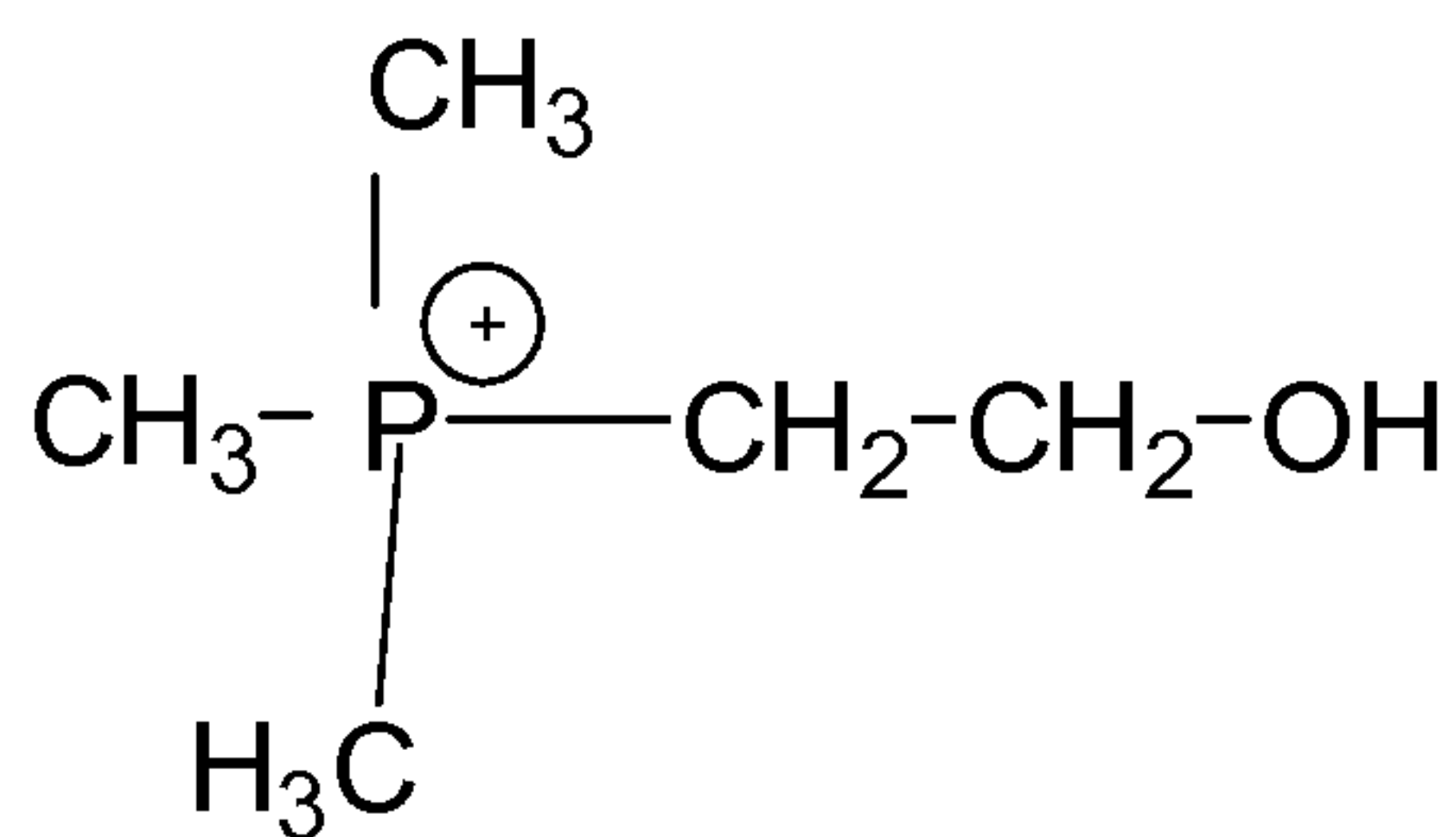
Phosphonium Choline,
