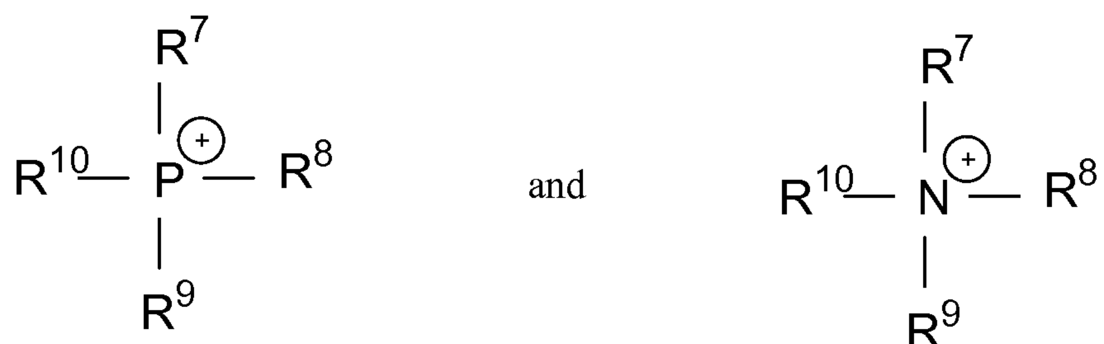
Phosphonium
