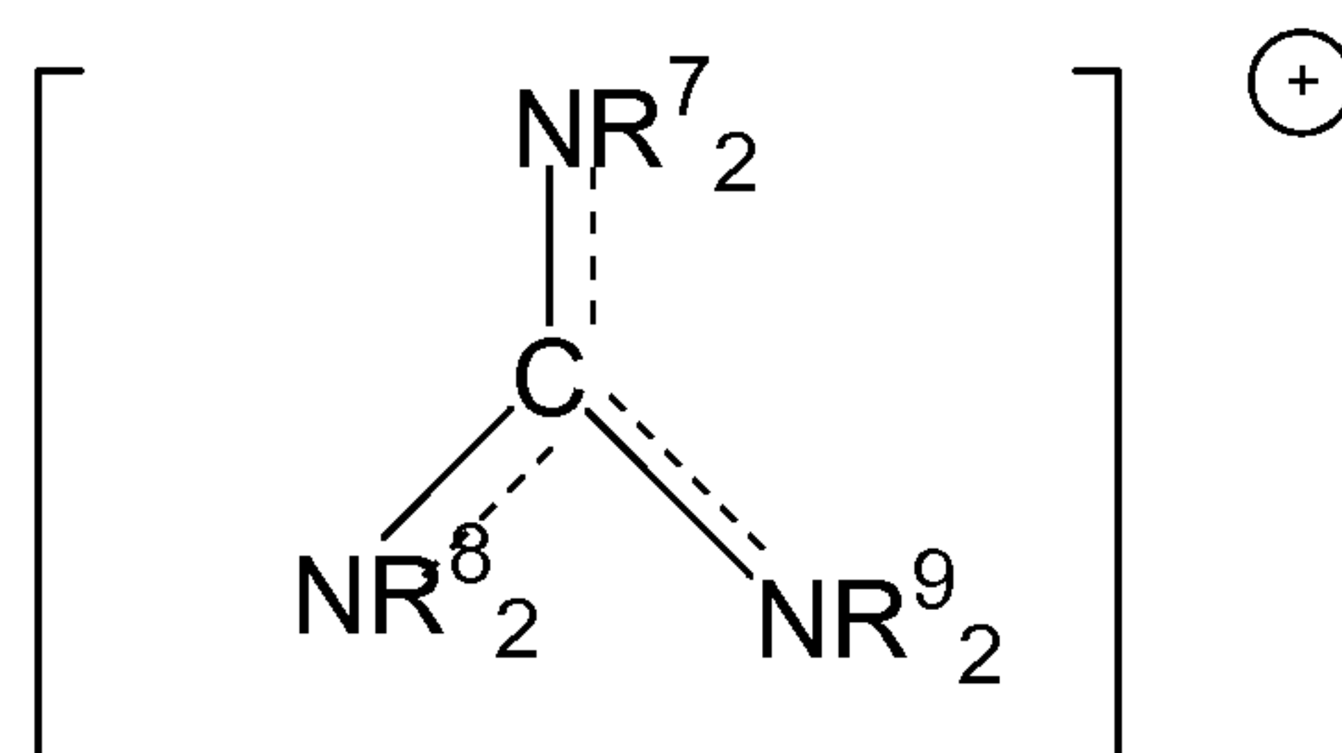
Guanidinium,
