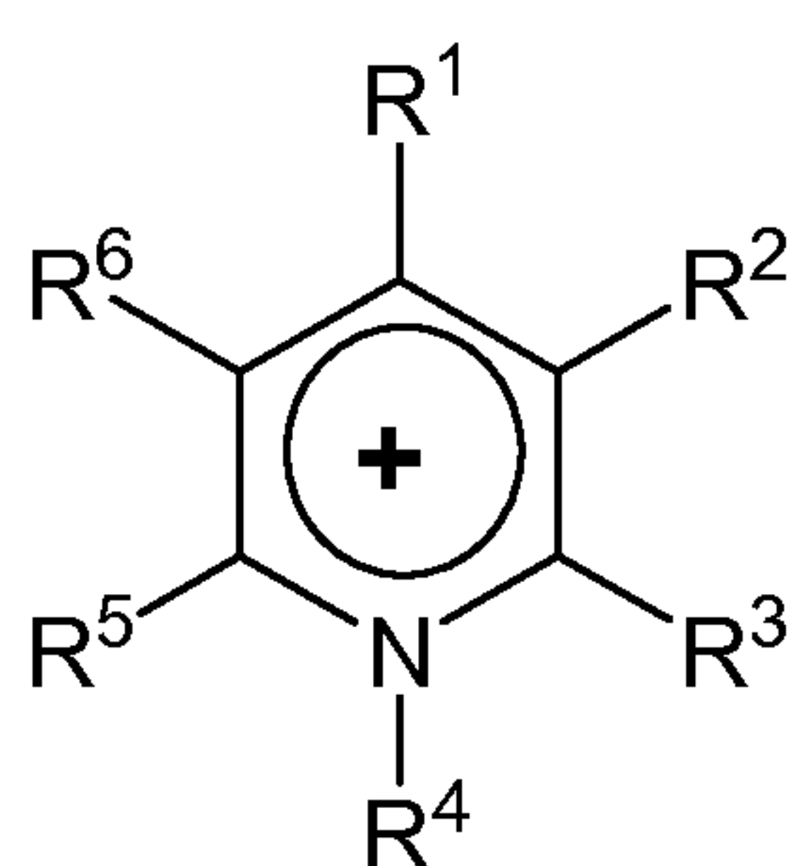
10 Pyridinium;
