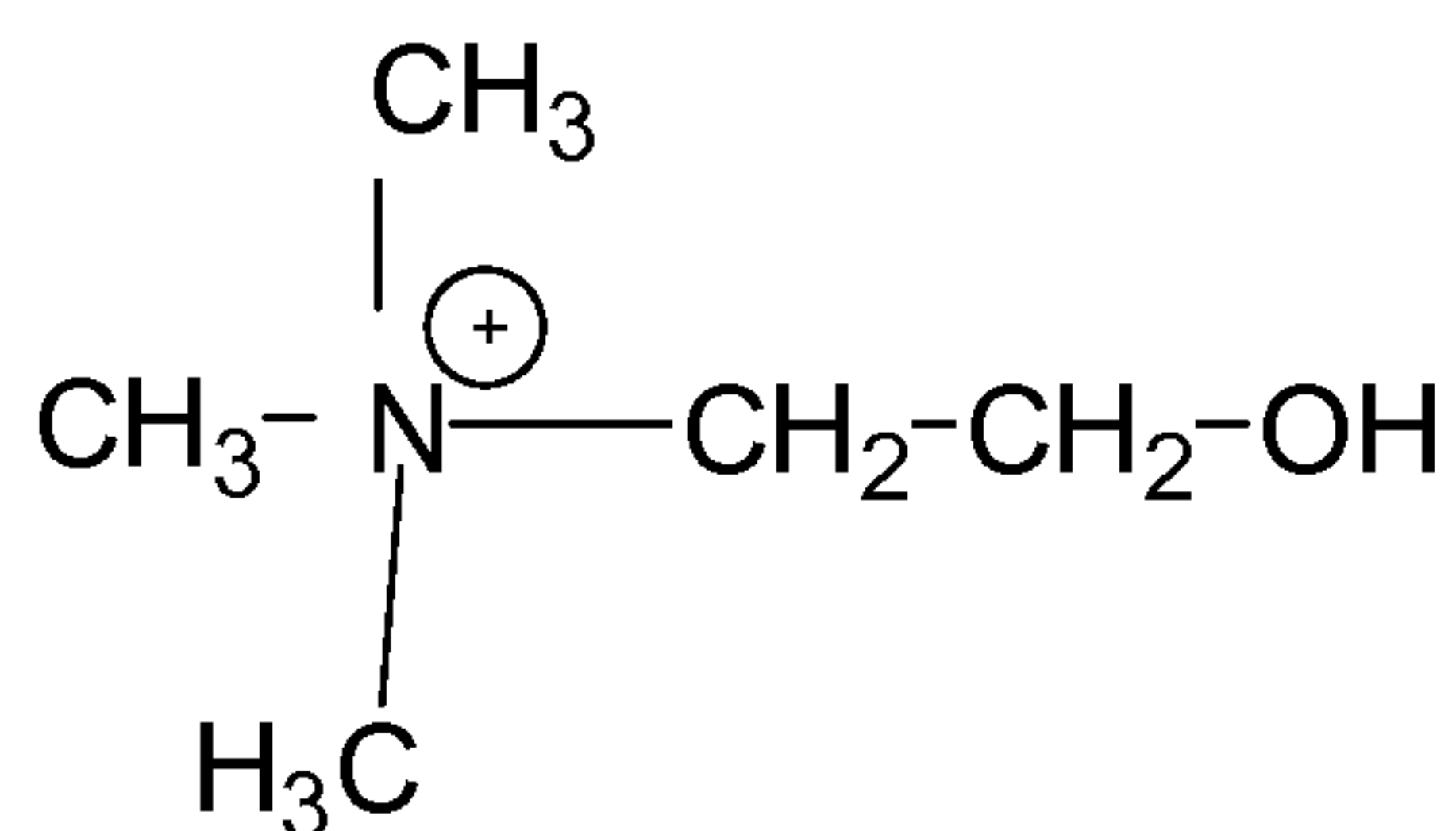
Choline,
