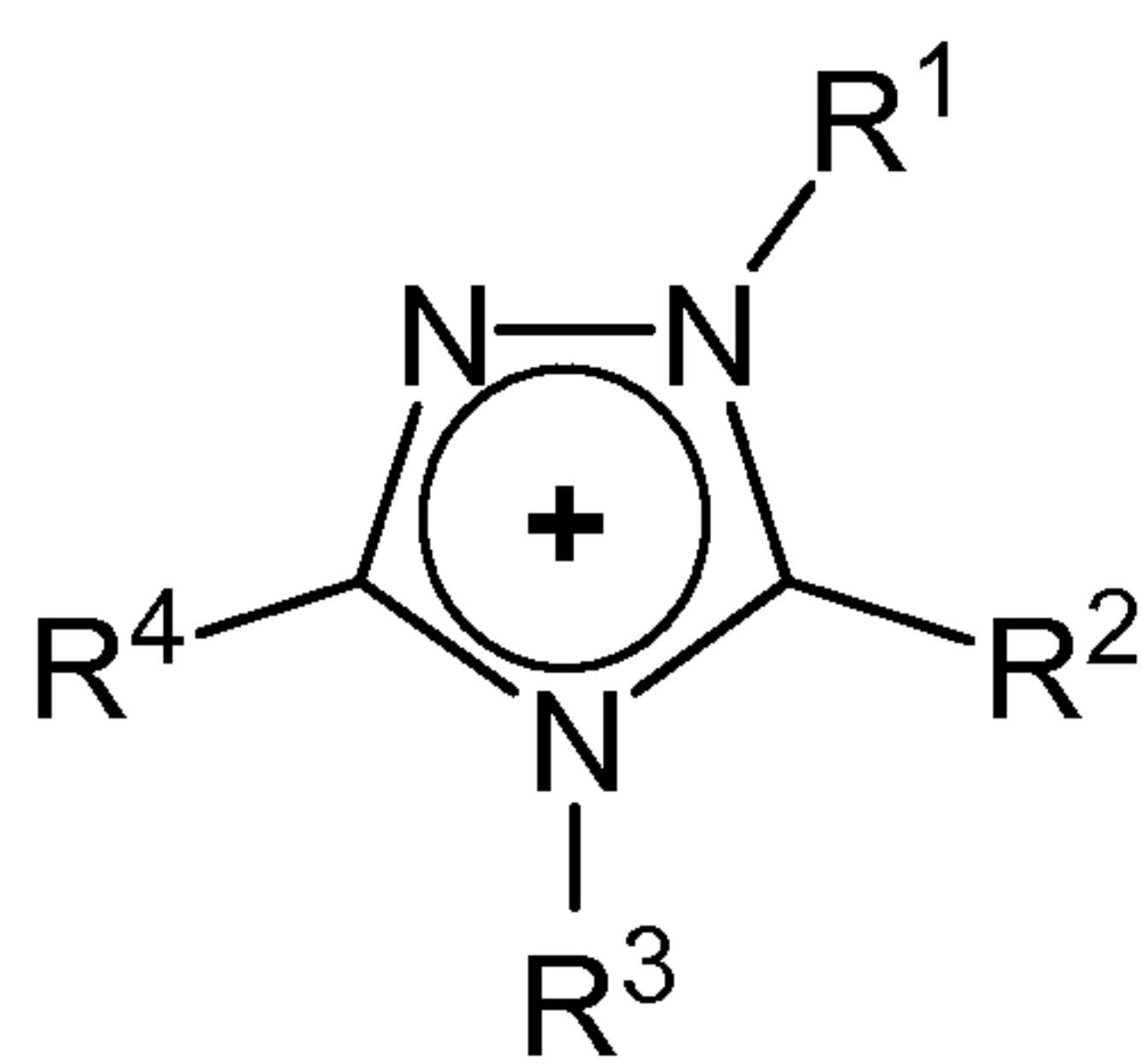
Triazolium,
