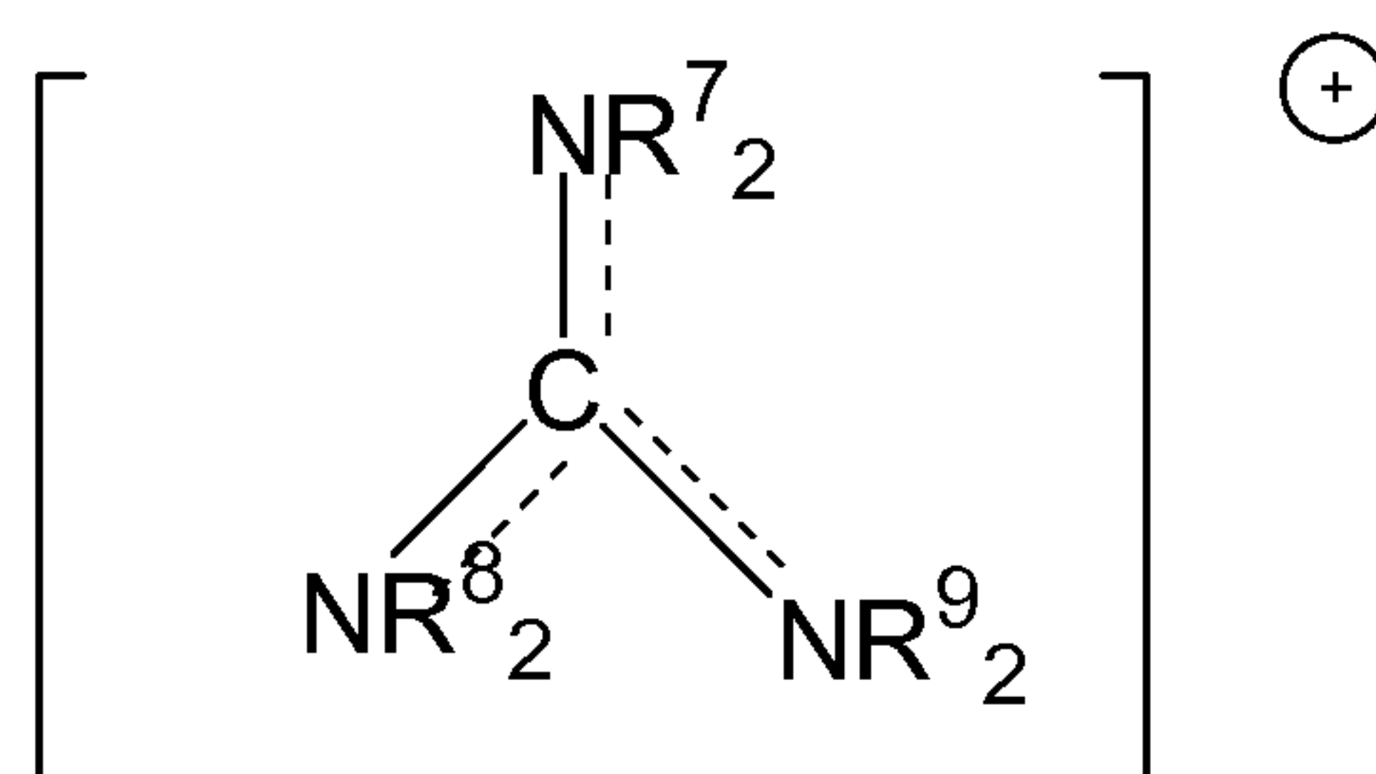
Guanidinium,
