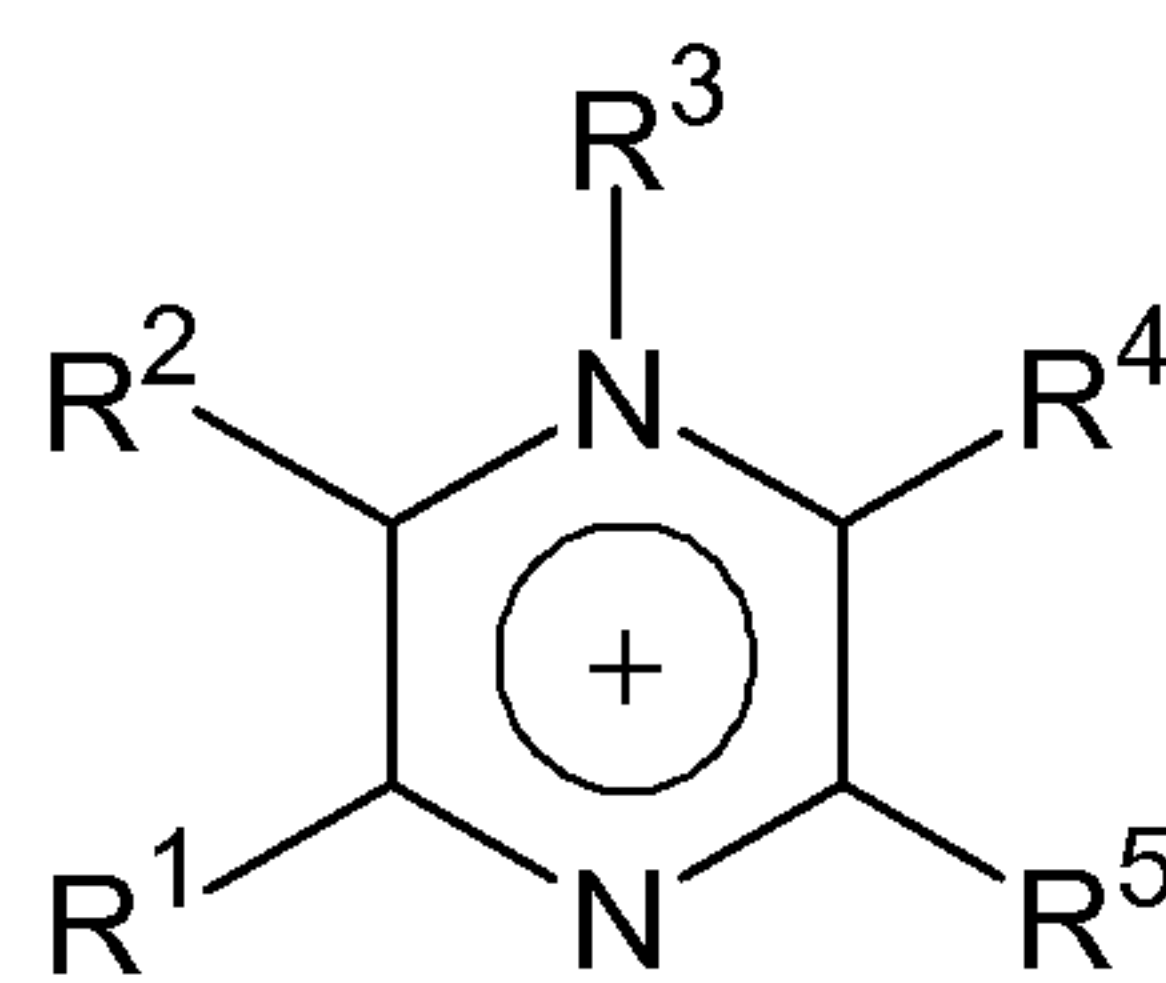
Pyrazinium,
