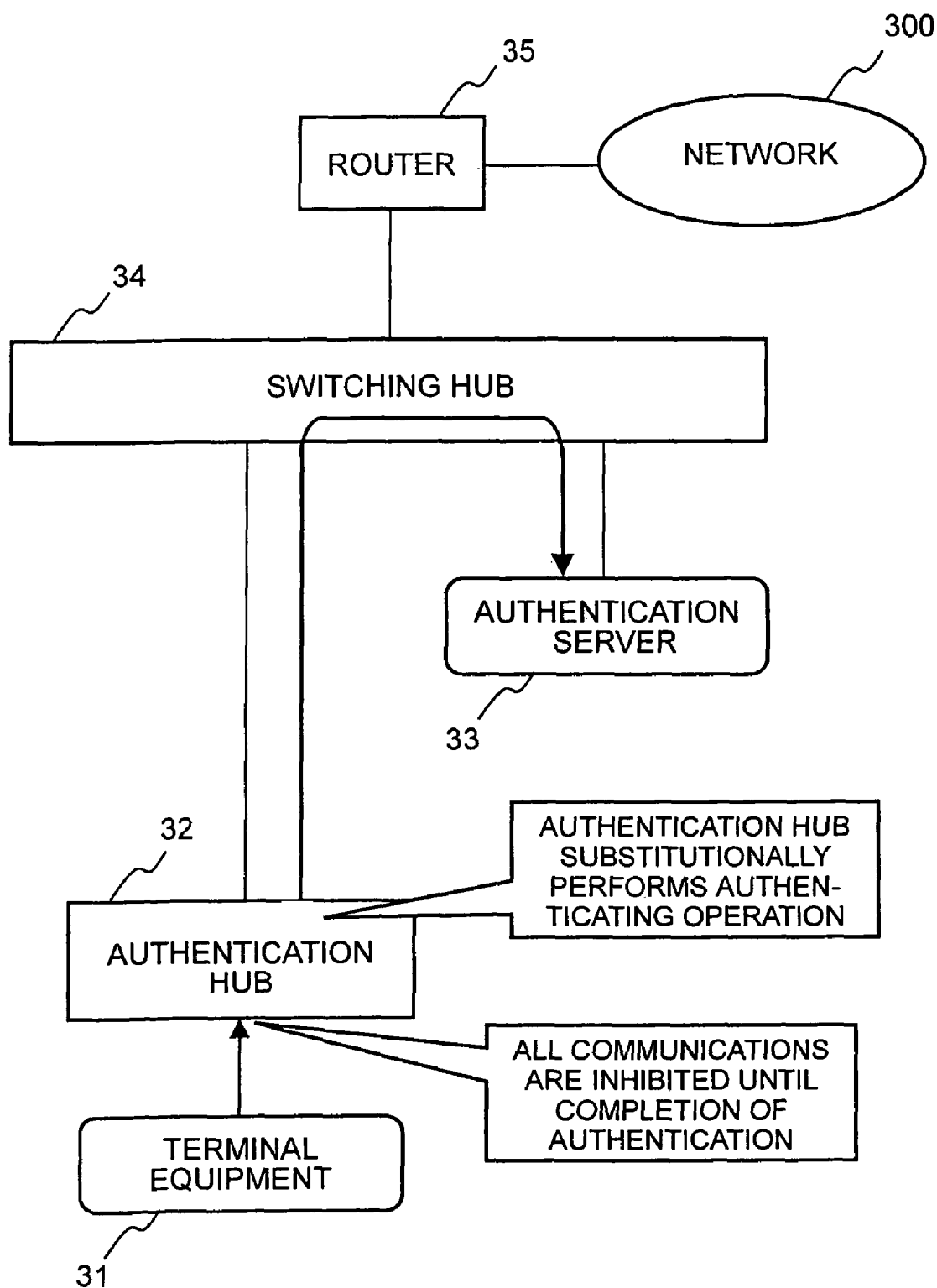
FIG. 1 PRIOR ART
