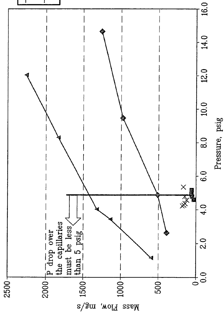
Mass Flow vs. Pdrop for 1.5" Regular Wall Capillary and Thin Wall Capillary
