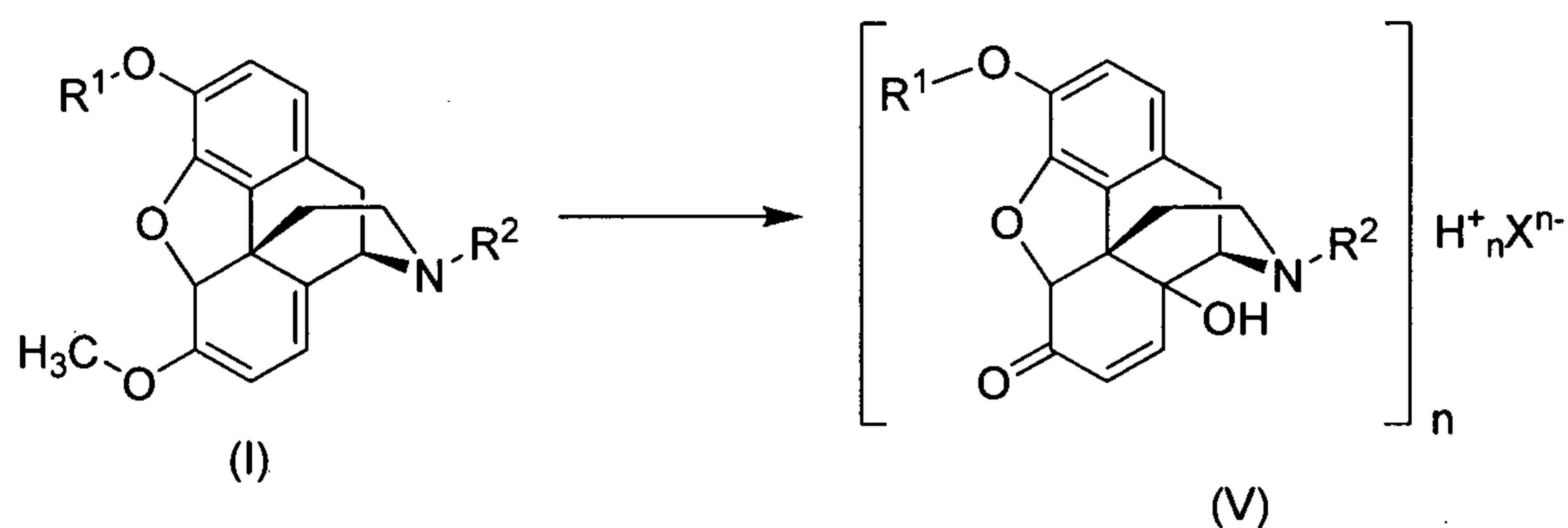
Scheme 5
