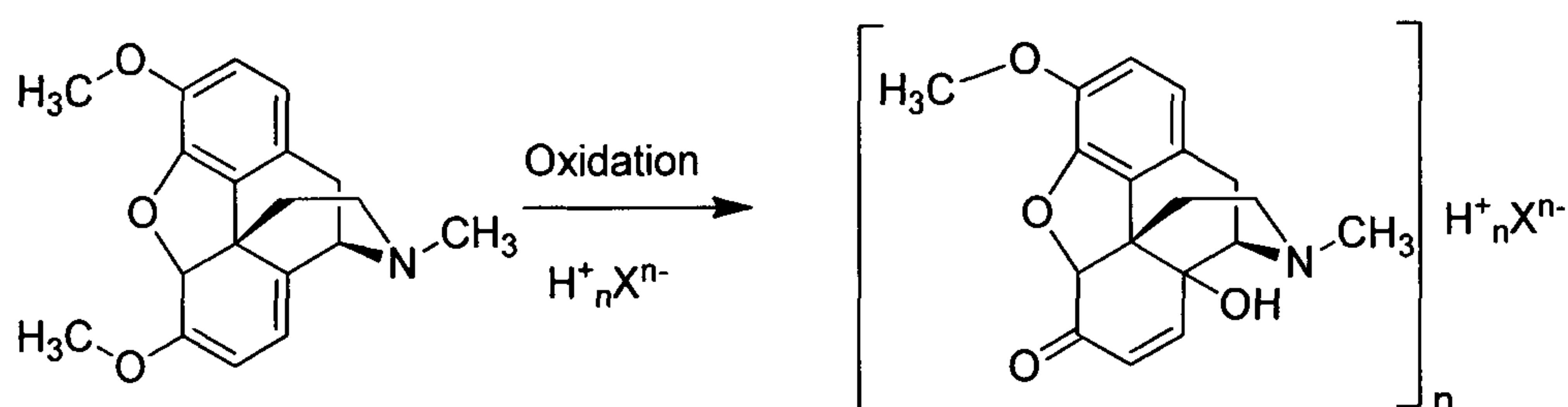
Scheme 11
