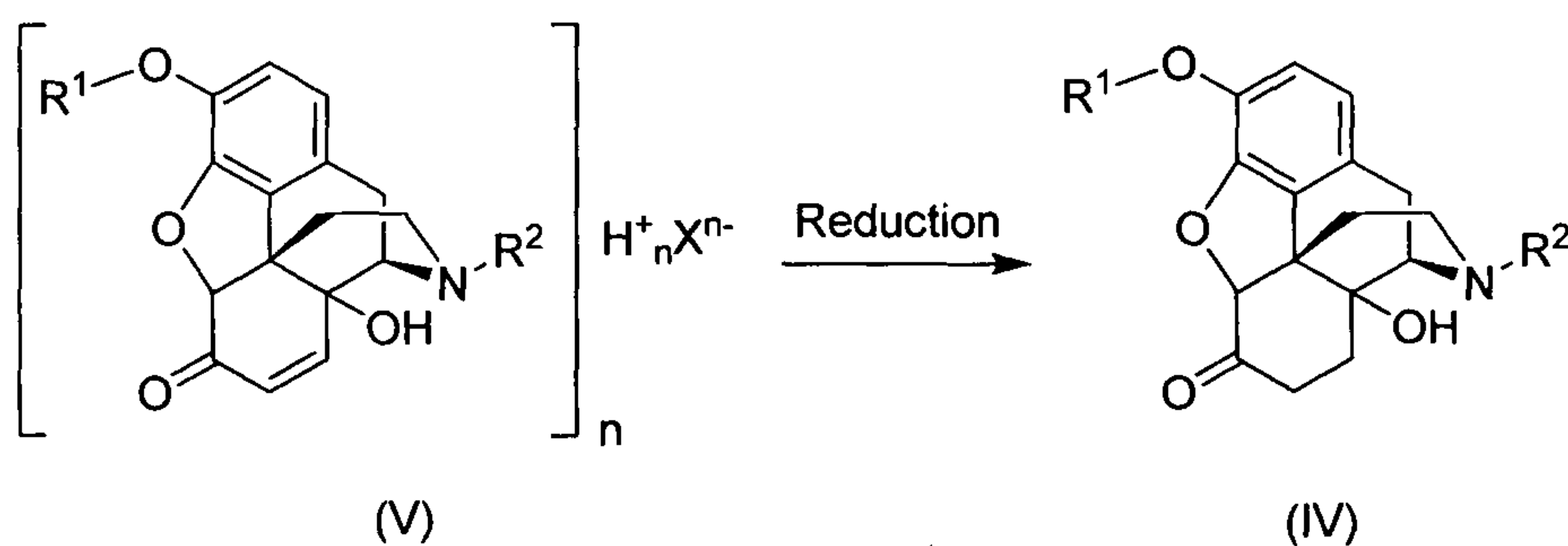
Scheme 17
