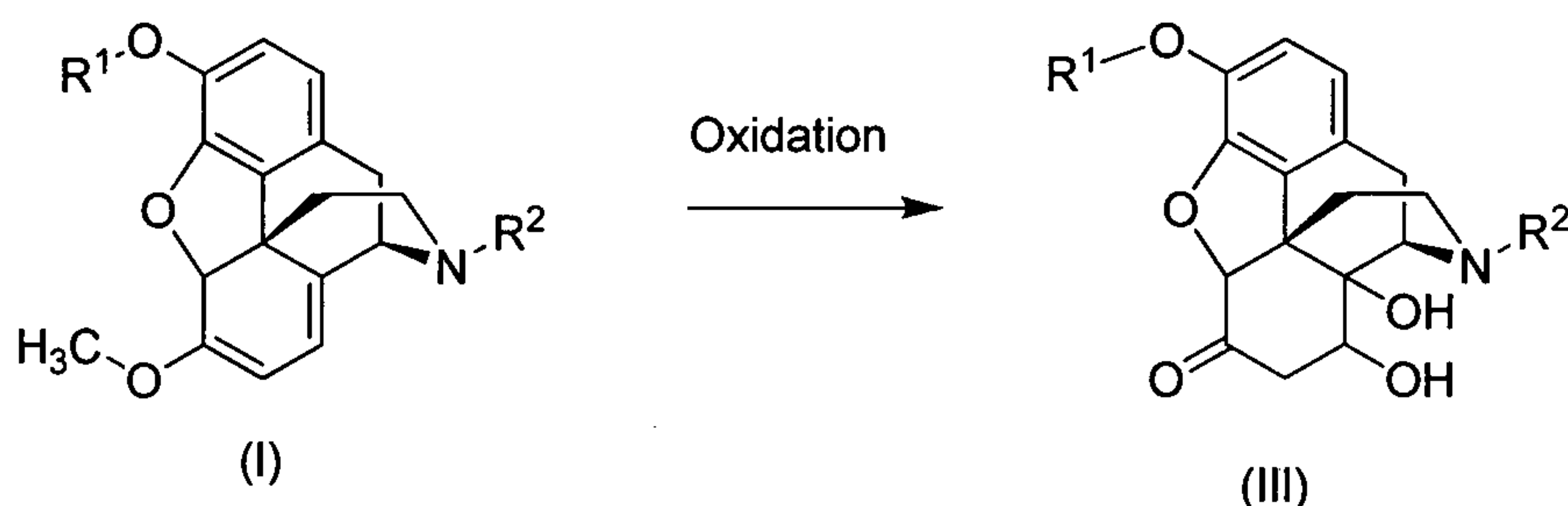
Scheme 6
