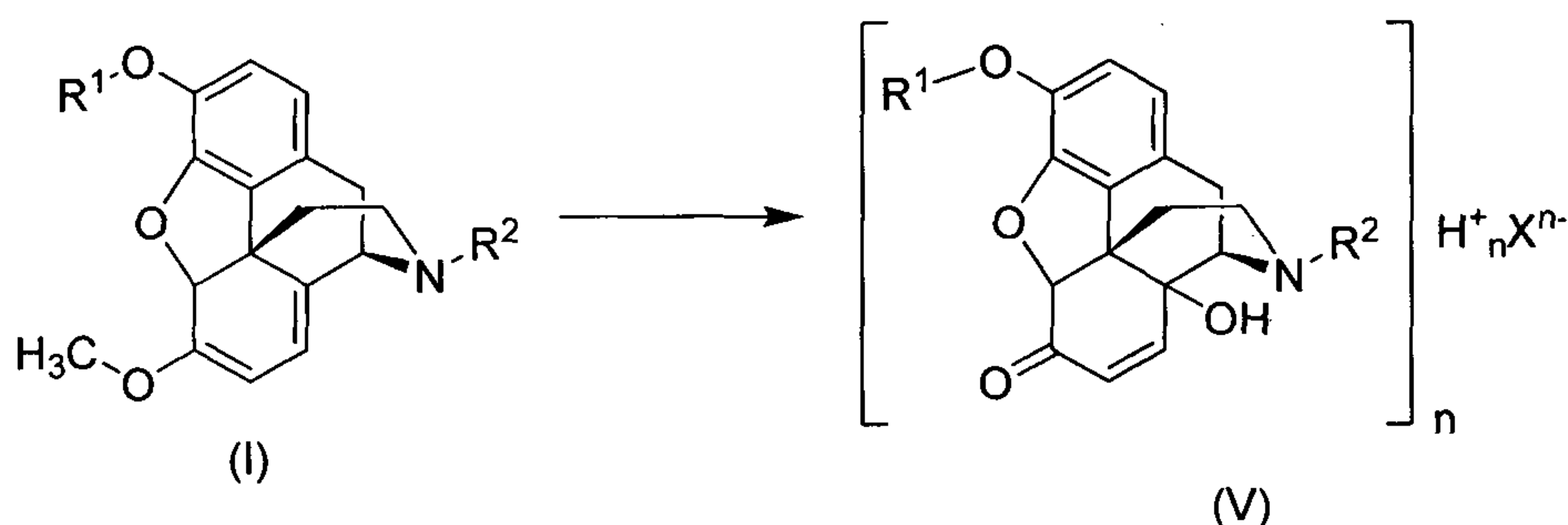
Scheme 5
