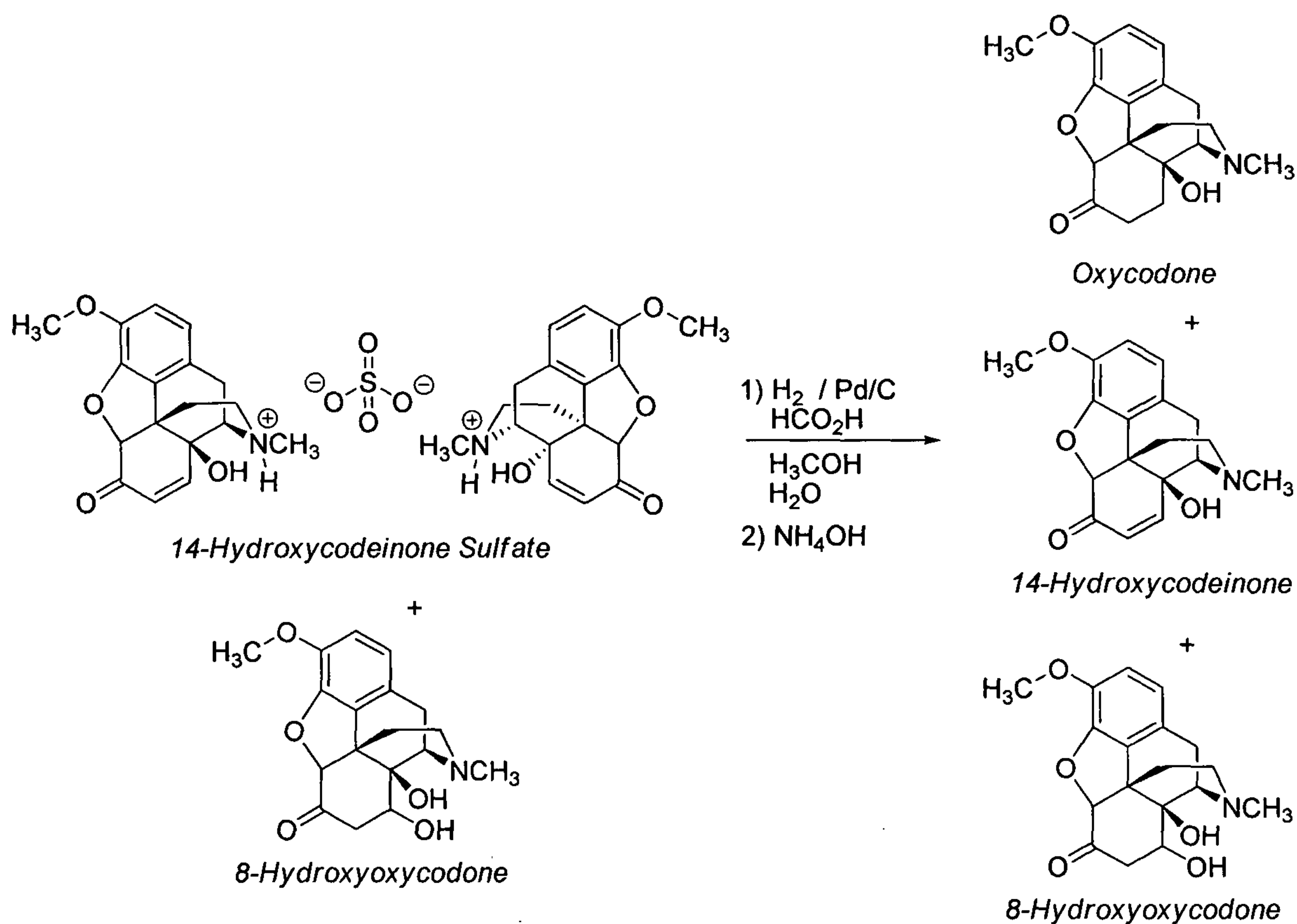
Scheme 18
