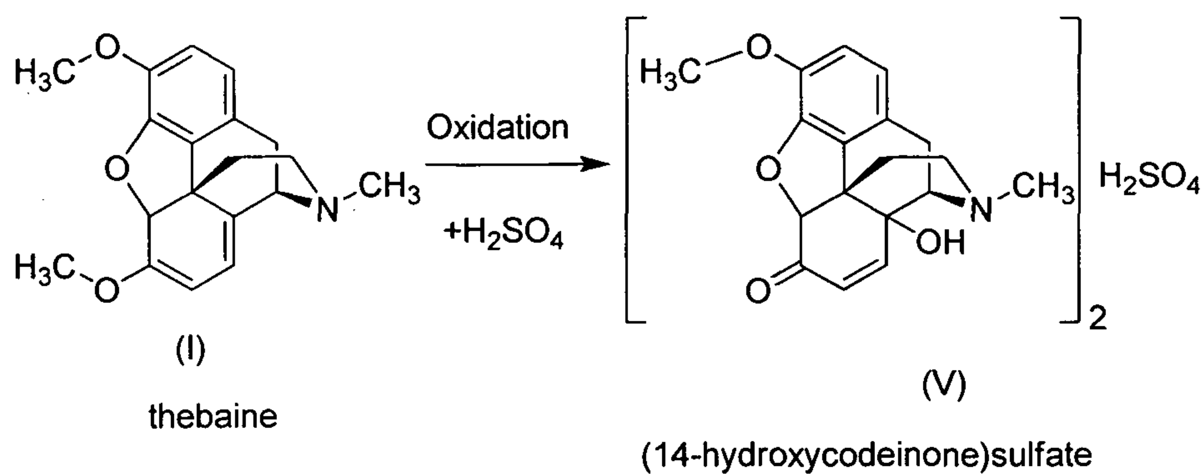
Scheme 7
