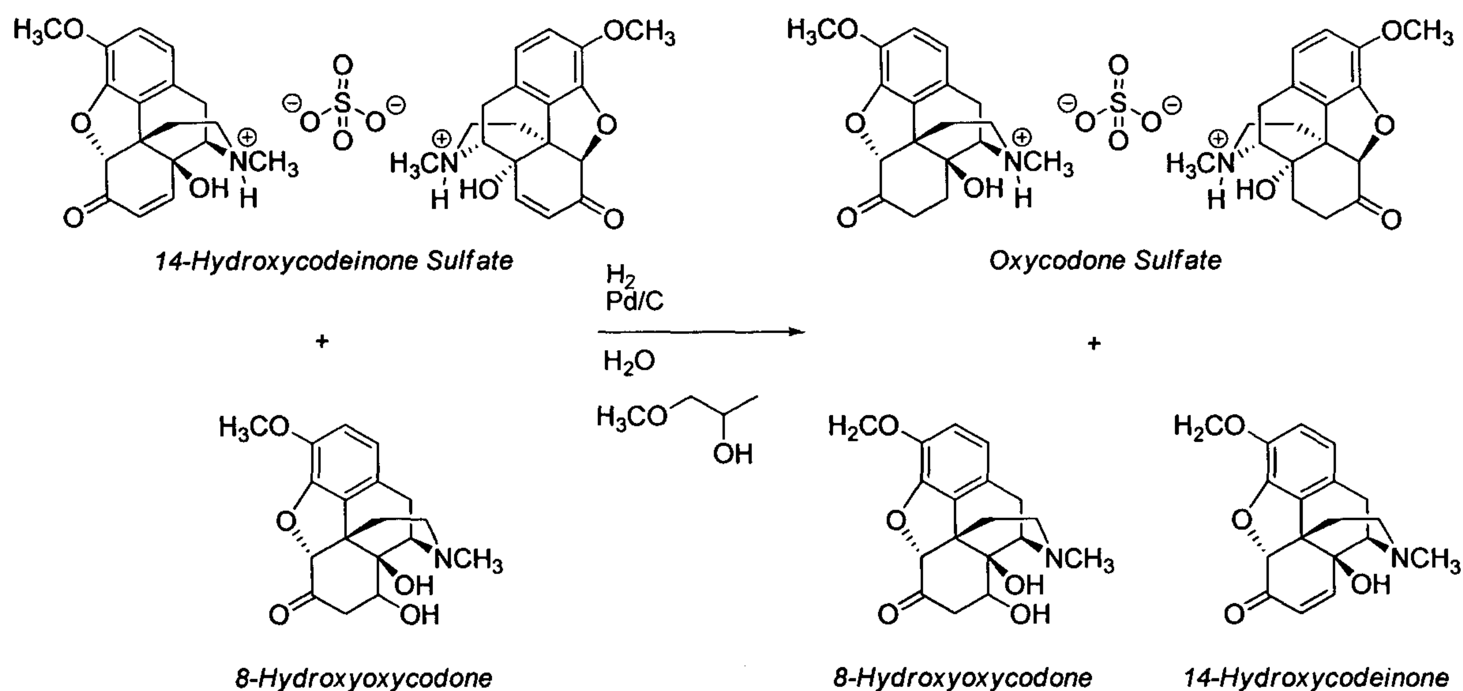
Scheme 18A
