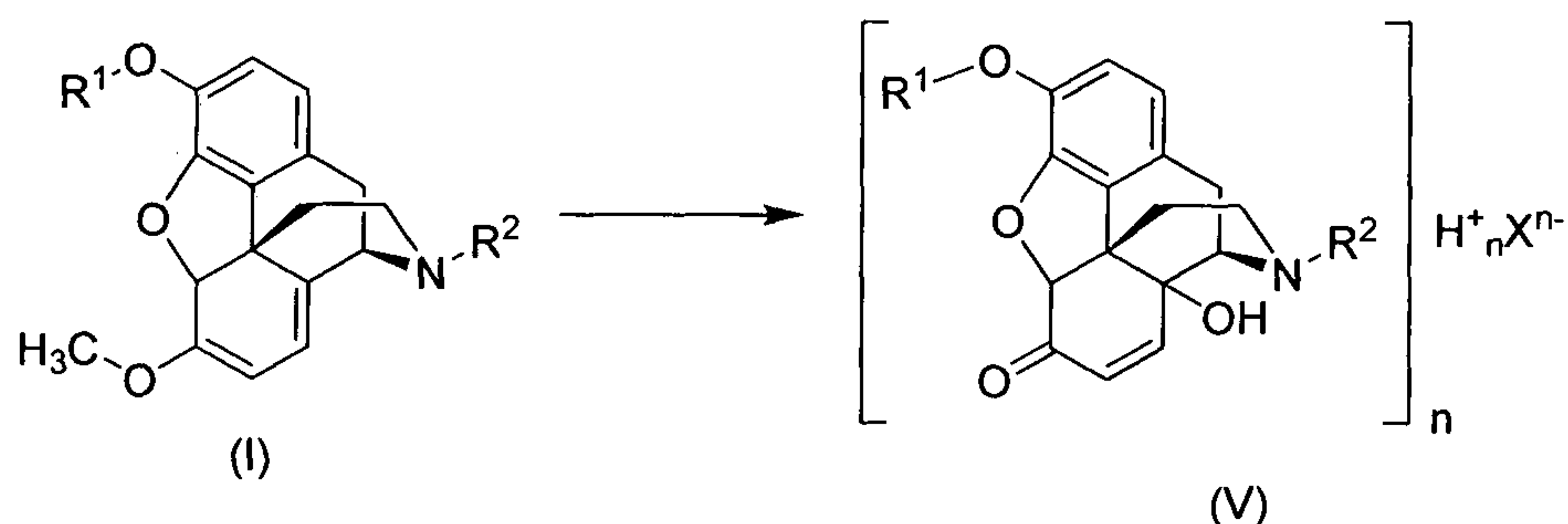
Scheme 9
