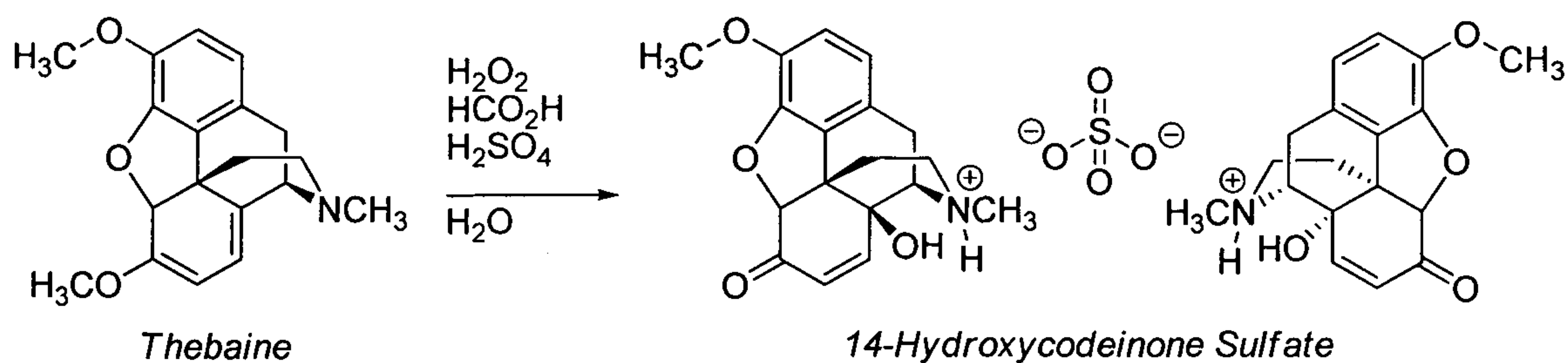
Scheme 13
