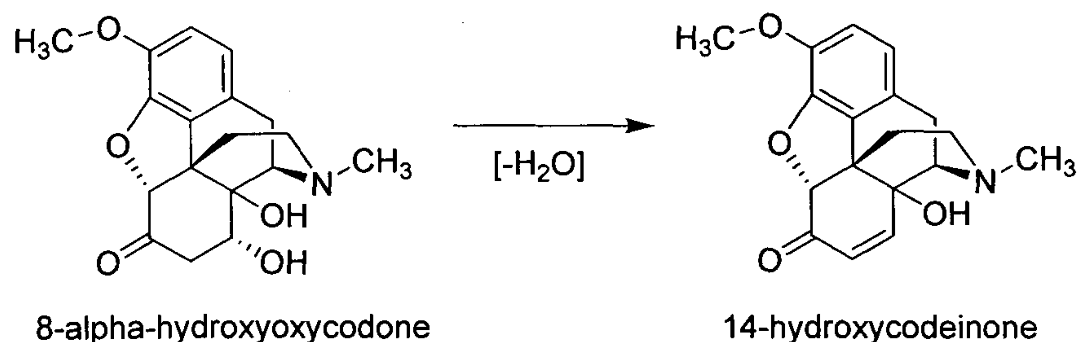
Scheme 3
