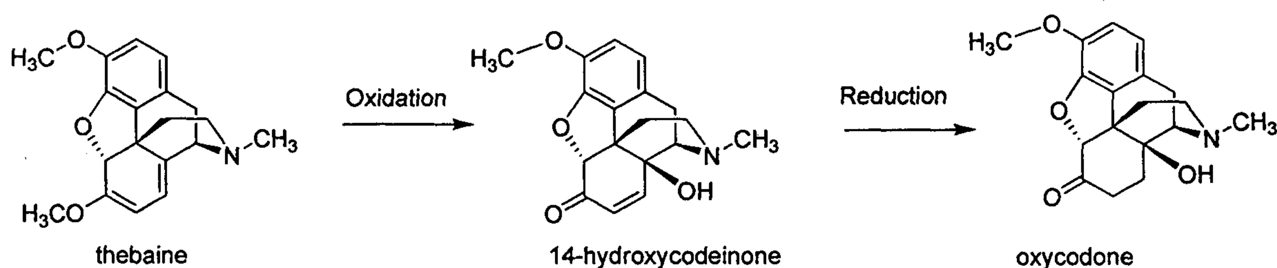
Scheme 1
