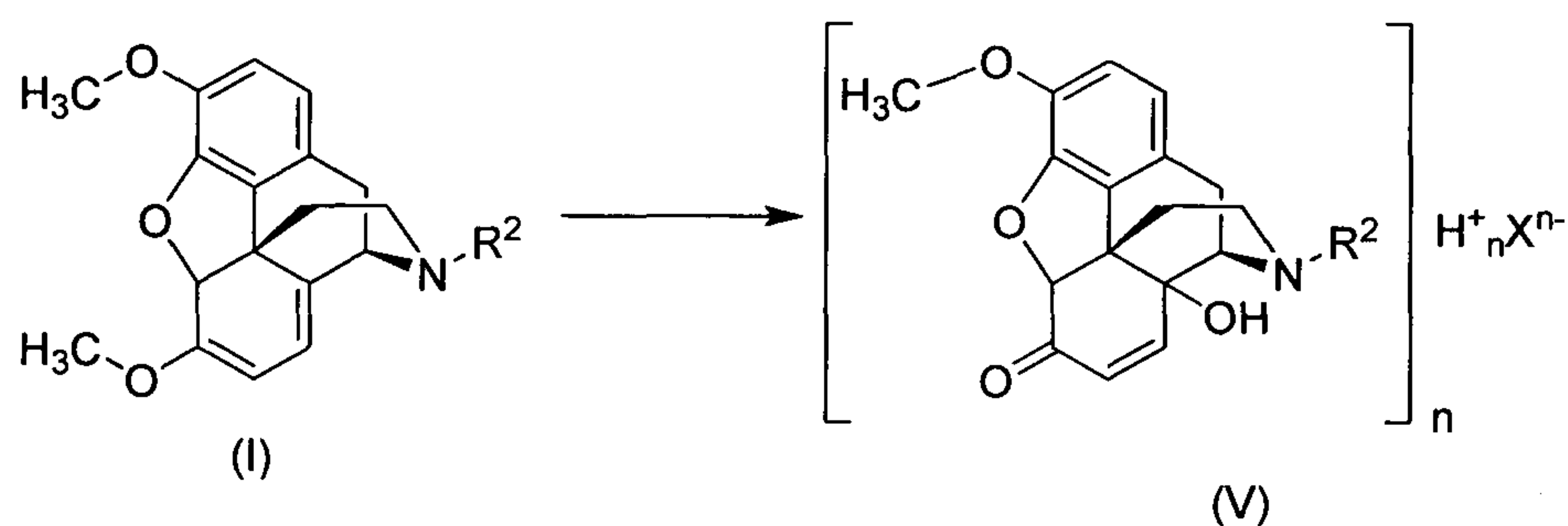
Scheme 14
