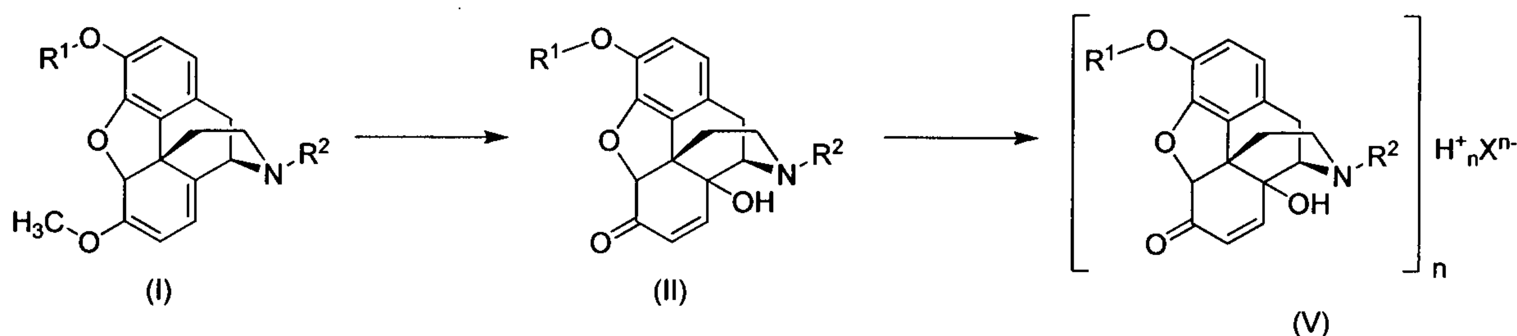
Scheme 10
