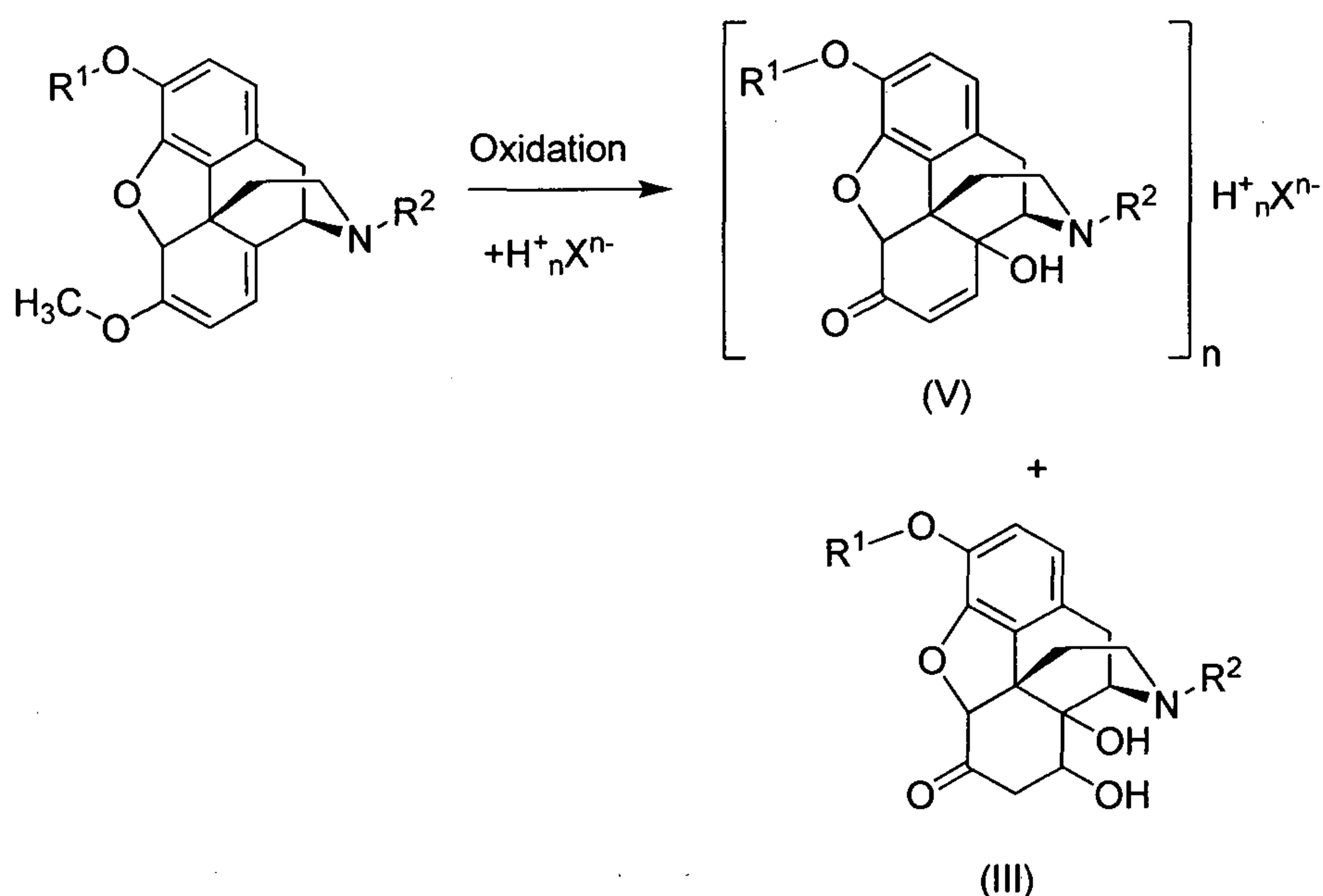
Scheme 16
