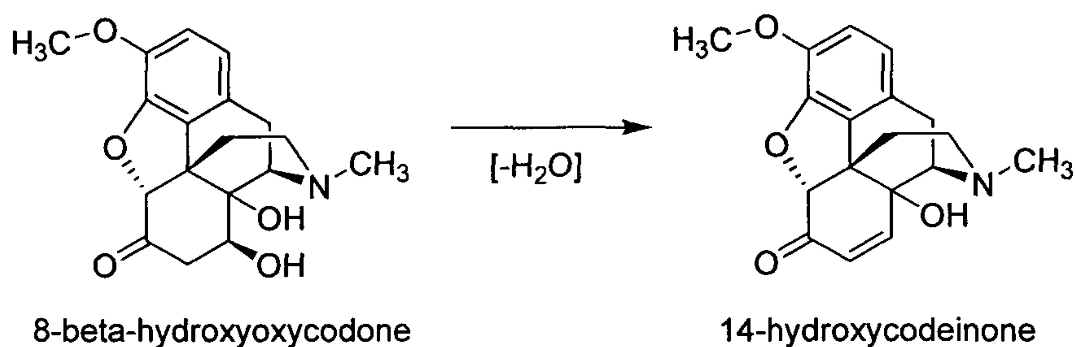
Scheme 4
