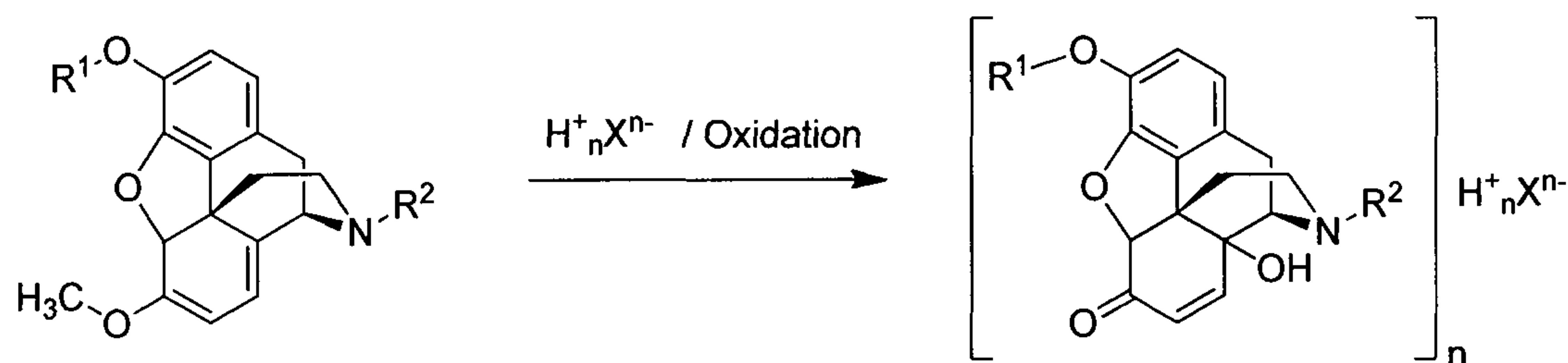
Scheme 12
