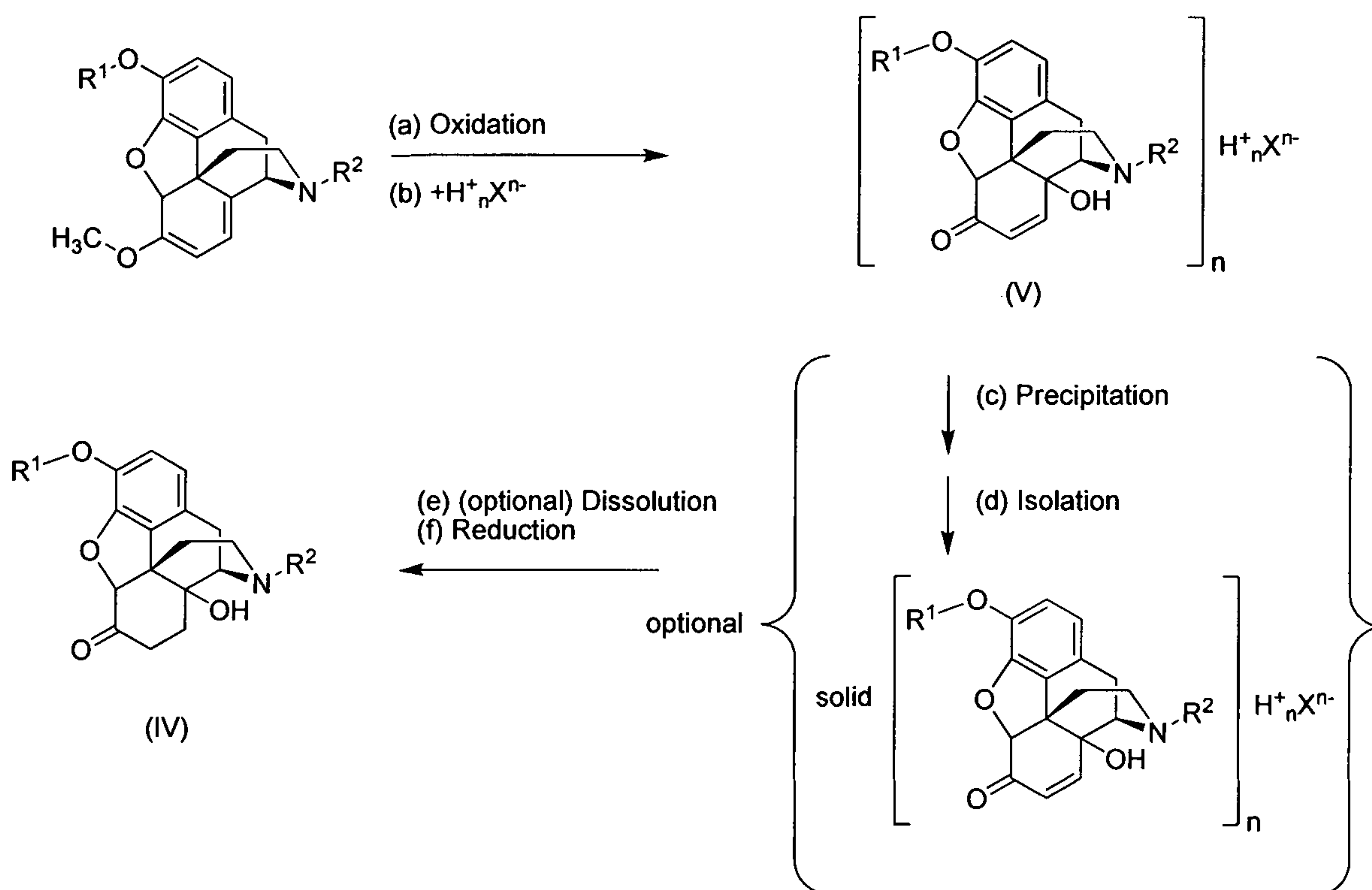
Scheme 19
