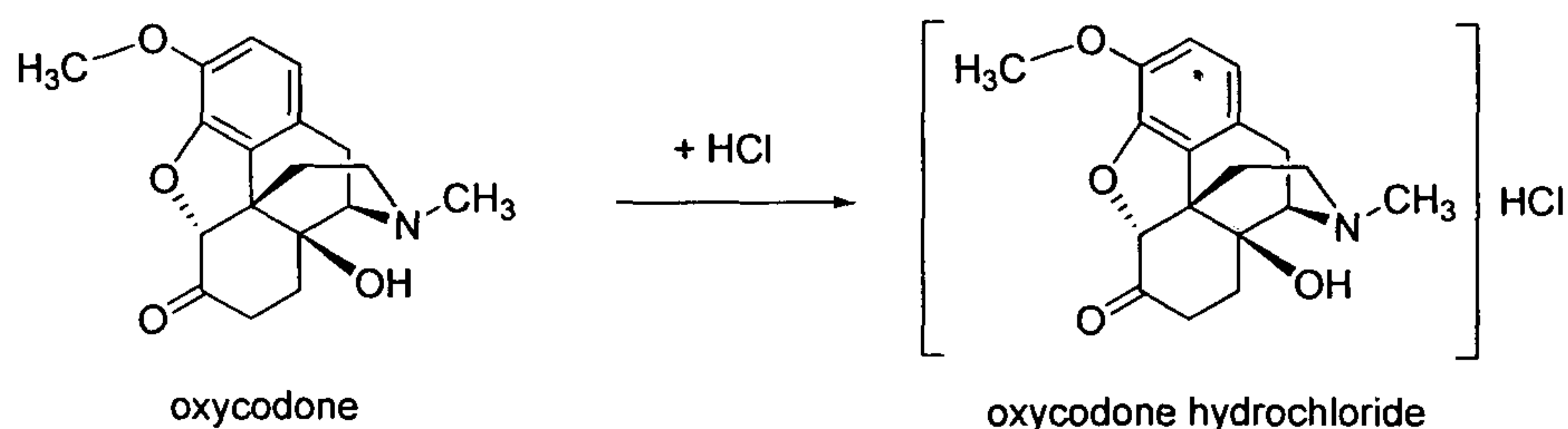
Scheme 2
