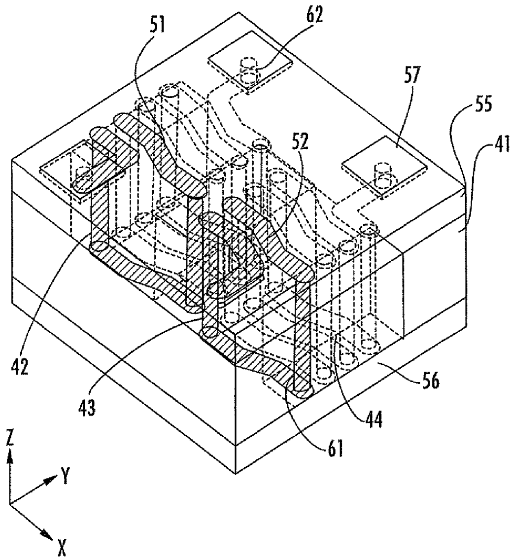
FIG. 3 (PRIOR ART)
