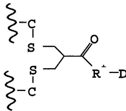
formula (VI)
