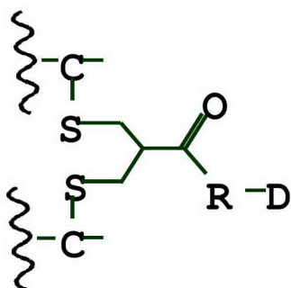
formula (V)
