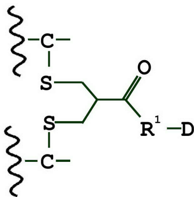
formula (V)
