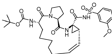
Compound 2116
