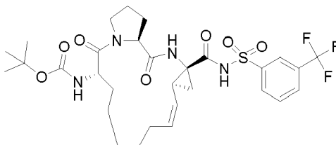
Compound 2149
