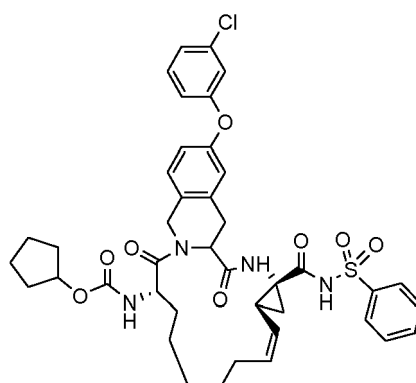
Compound 2004
