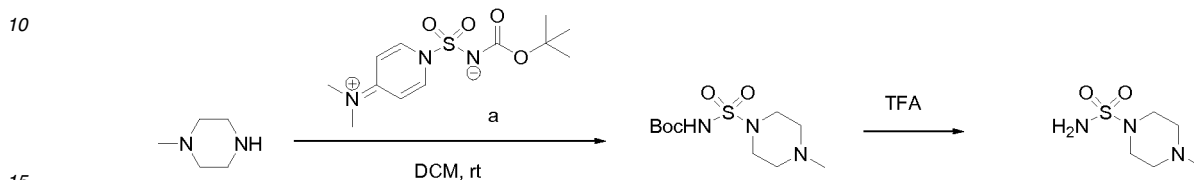
Scheme 5
