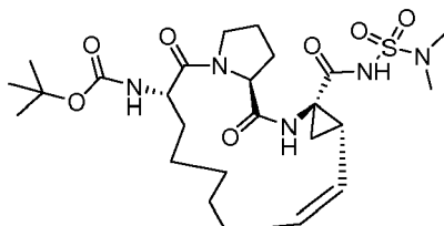
Compound 2202
