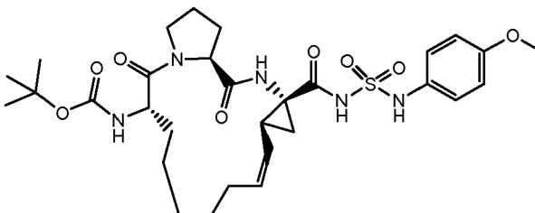
Compound 2244
