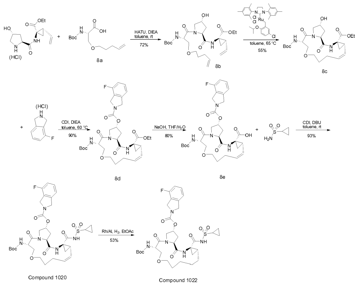
Scheme 8
