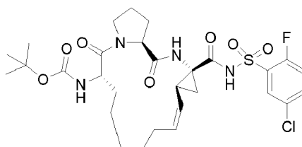
Compound 2150
