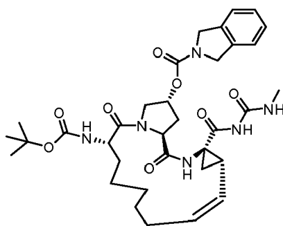
Compound 703
