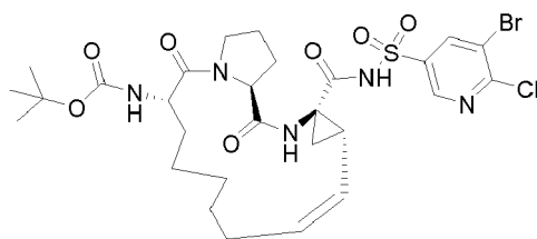
Compound 2154
