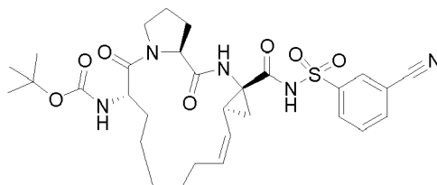
Compound 2152
