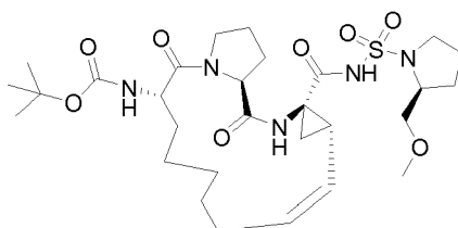
Compound 2252
