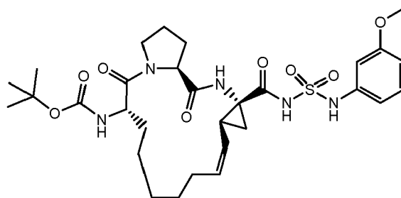
Compound 2240
