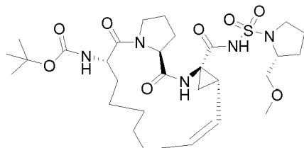
Compound 2251
