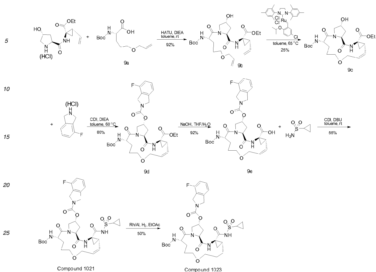
Scheme 9
