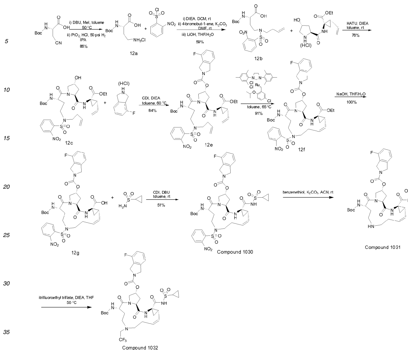
Scheme 12
