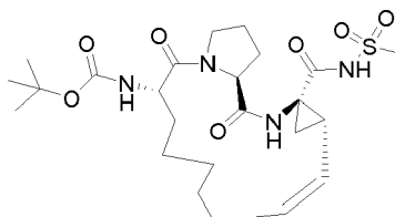
Compound 2103
