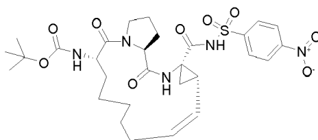
Compound 2102
