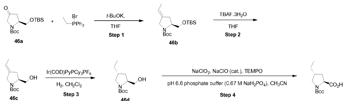
Scheme 4a
