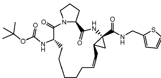
Compound 305
