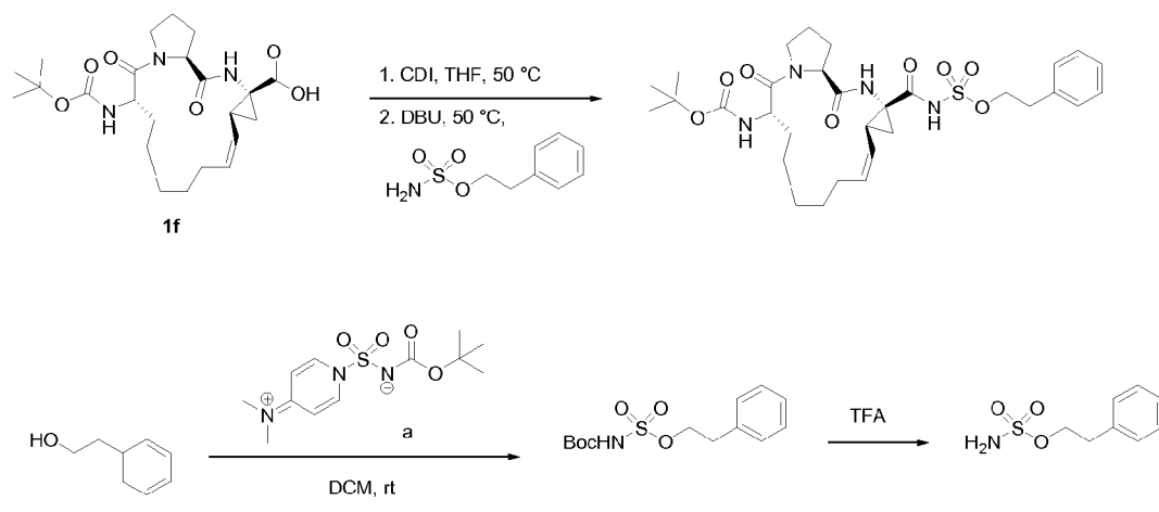
Scheme 6
