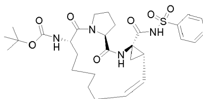
Compound 2101
