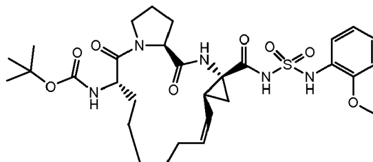
Compound 2236
