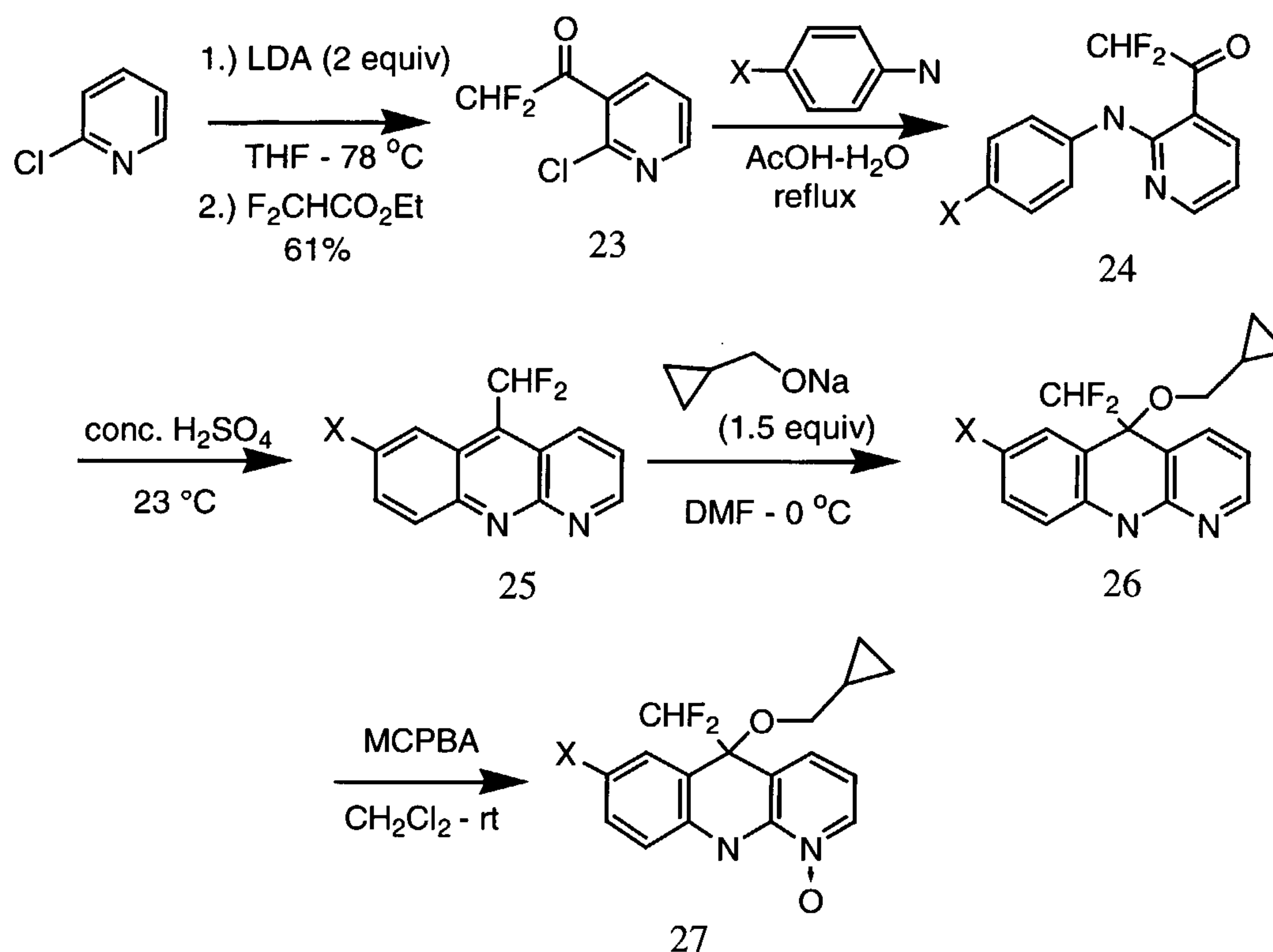
Scheme 5
