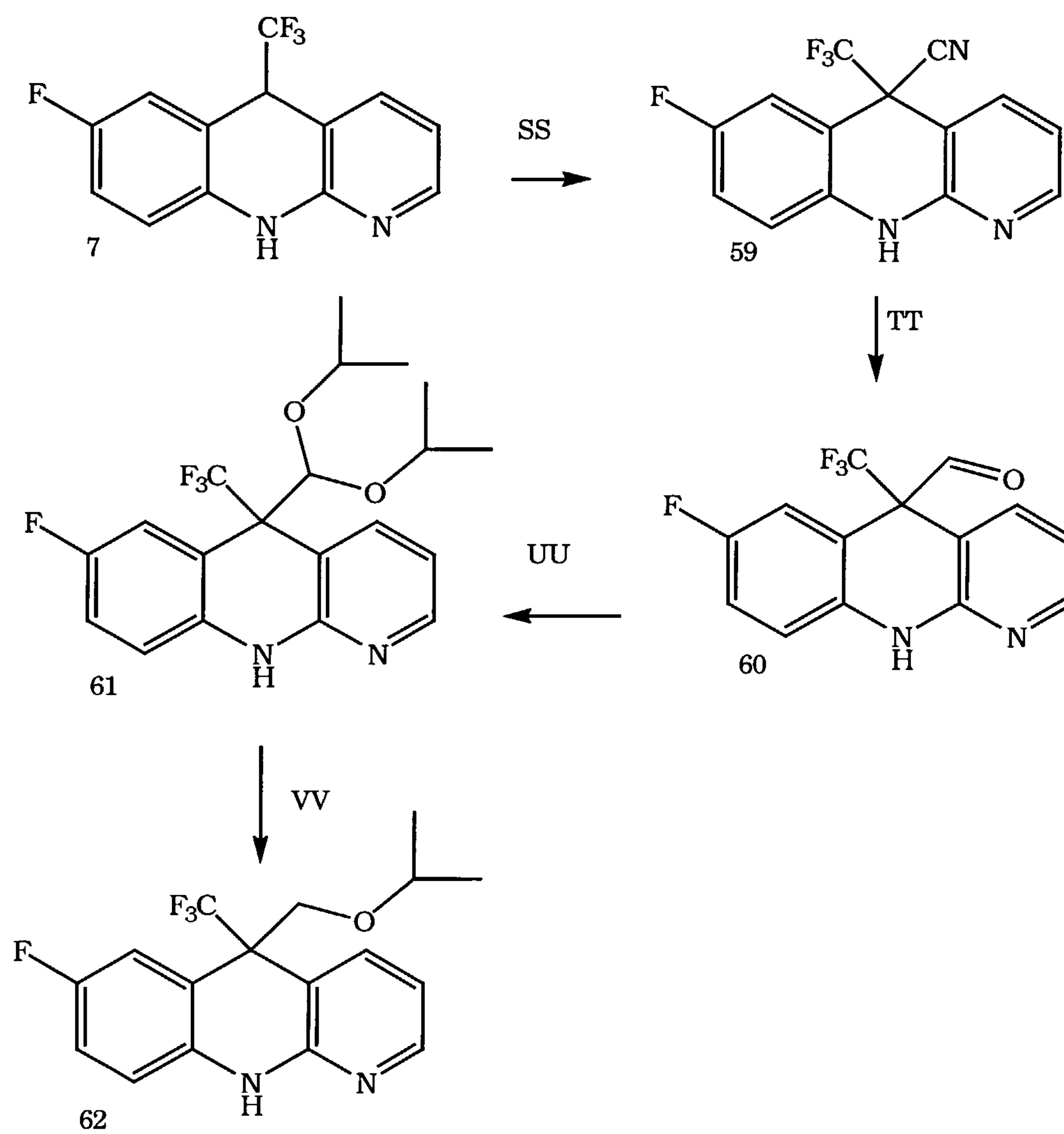
Scheme 8
