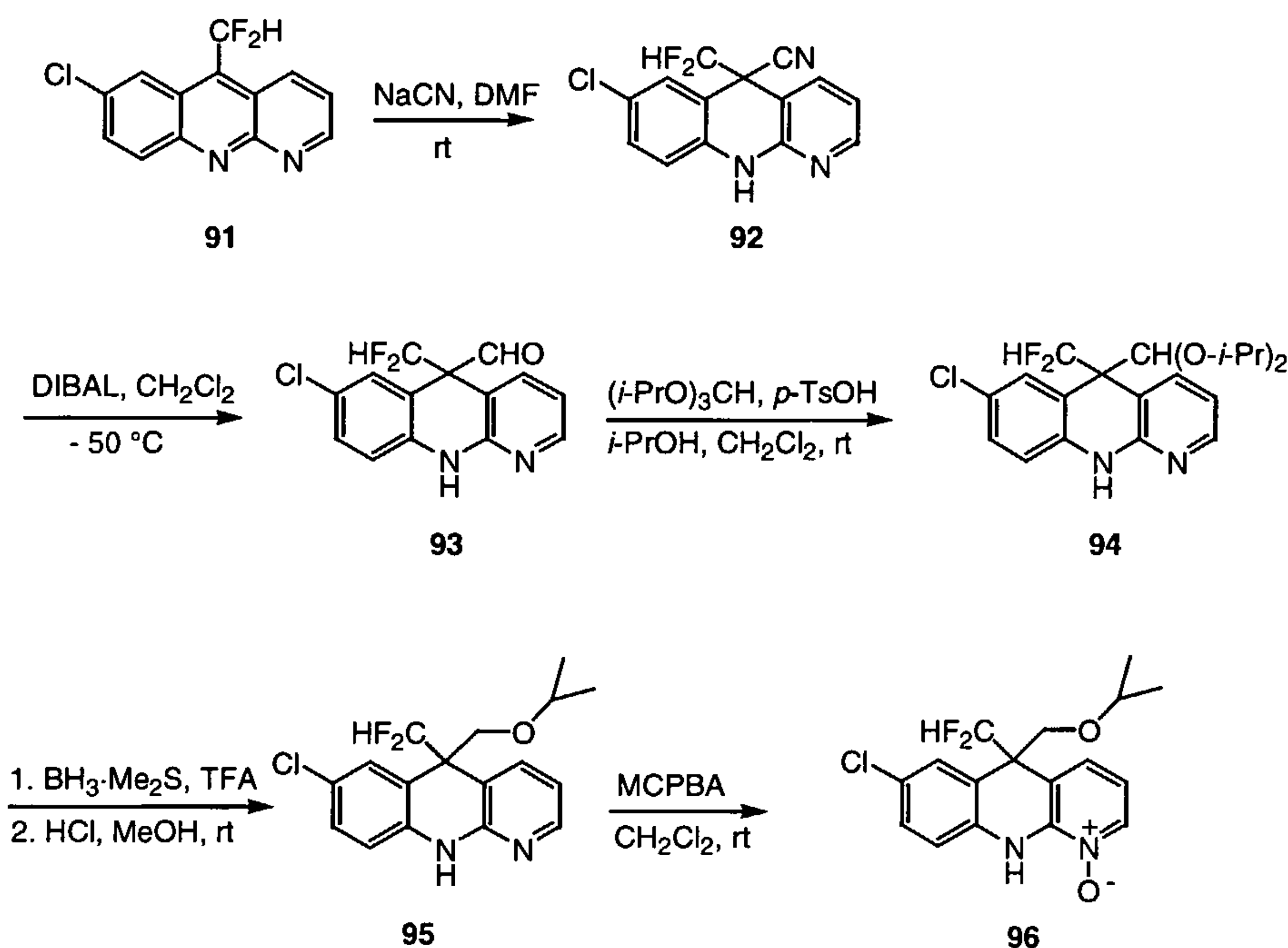
Scheme 12
