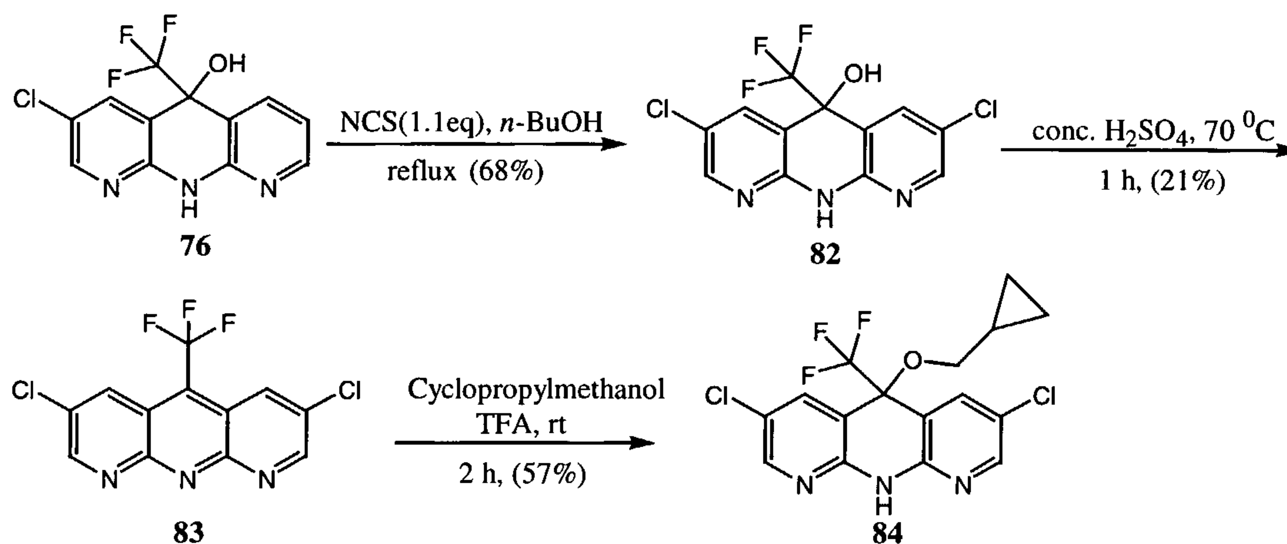
Scheme 11
