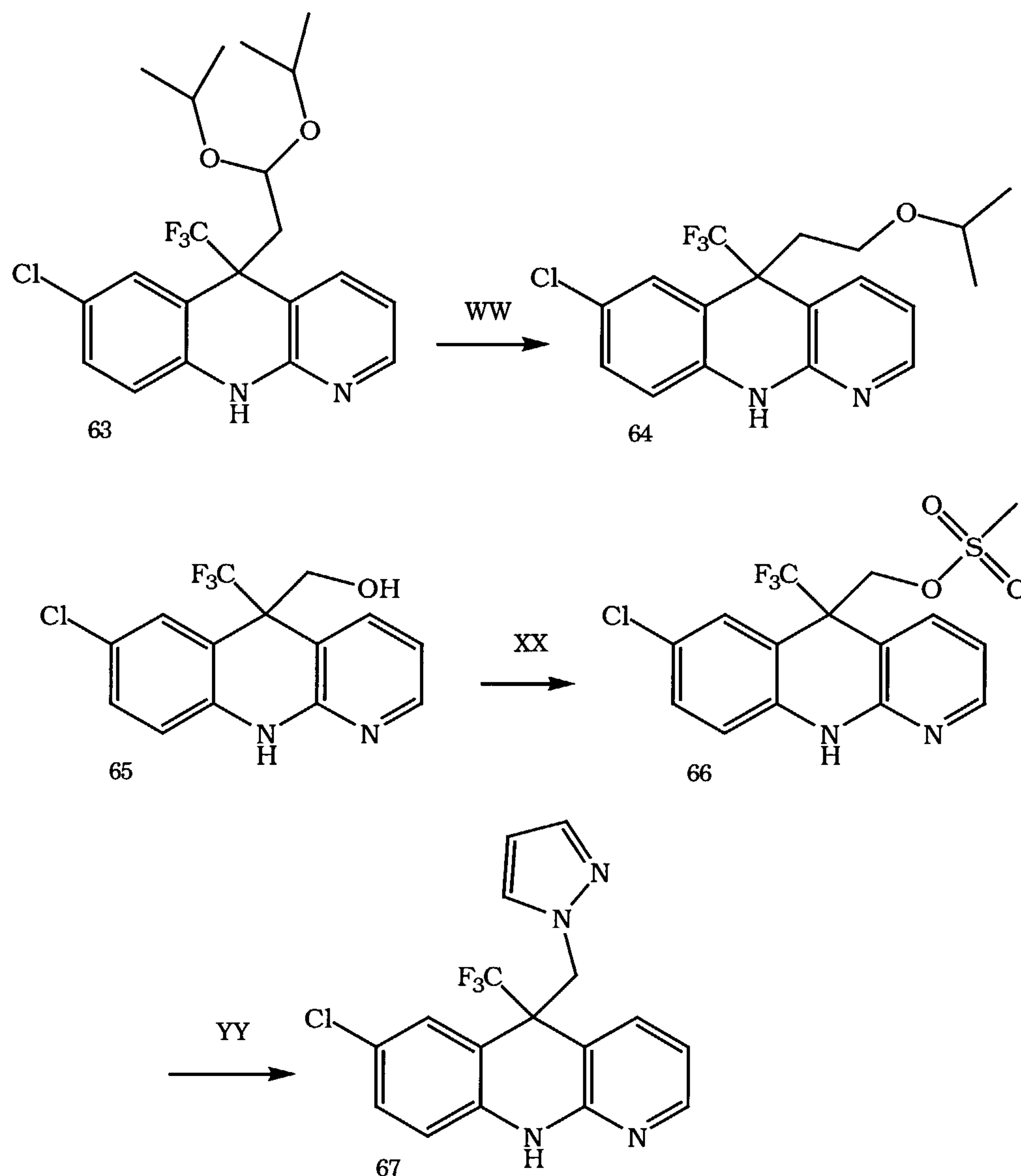
Scheme 9
