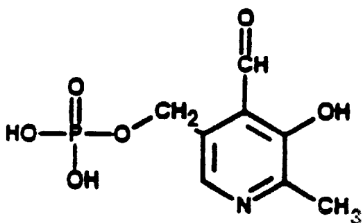
Pyridoxal-5'-Phosphate
