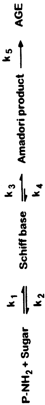
Scheme 5
